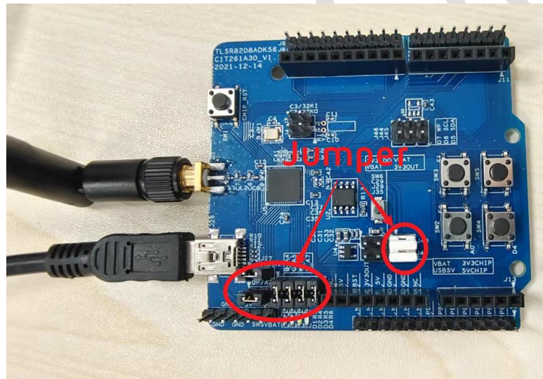
Figure 2-1 USB power supply
