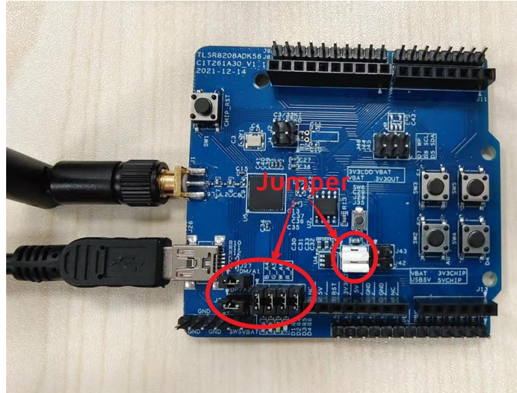
Figure 2-2 USB to LDO 3.3V power supply
