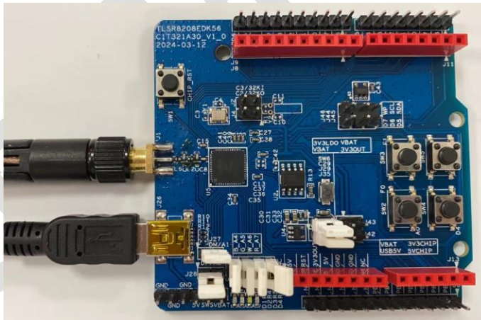
Figure 1-2 USB to LDO 3.3V power supply
