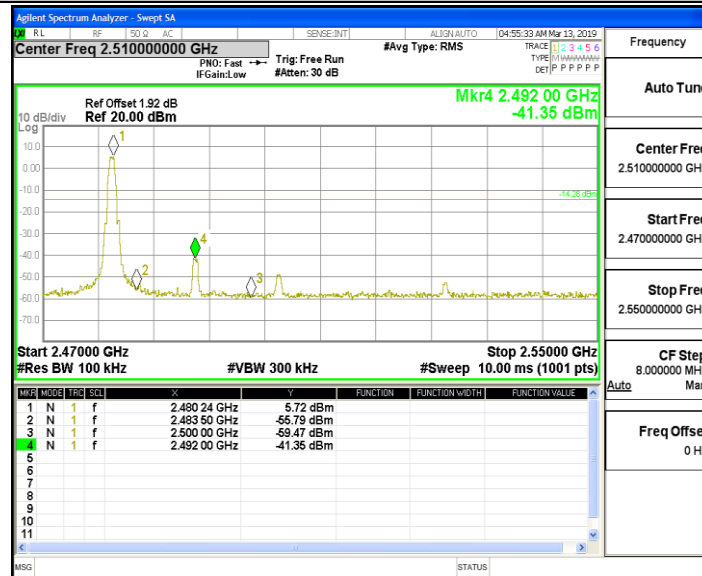
TX_Ant1_High_2480
