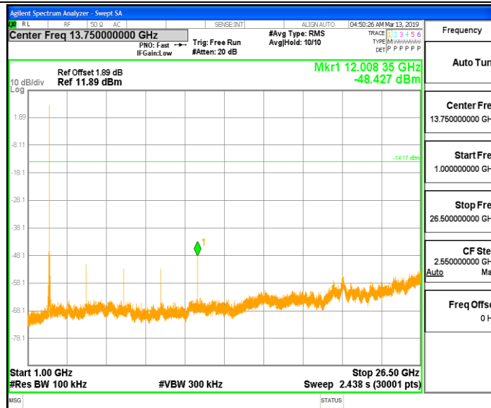
TX_Ant1_2442_0~Reference
