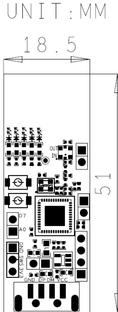
Figure 3 Mechanical dimensions
