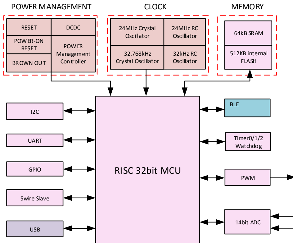
Figure 1 Block diagram
