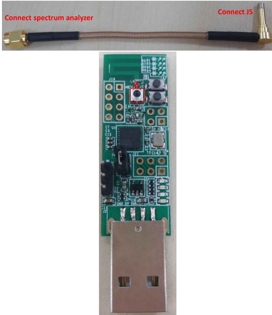
Figure 6 Connection chart to test RF signal
