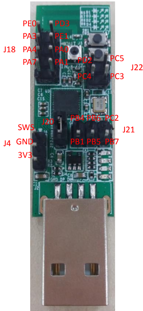
Figure 7 Test GPIO signals on header pins
