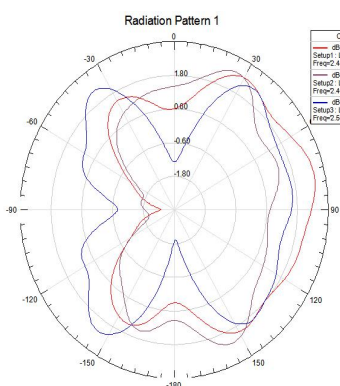
Radiation Pattern XOZ
