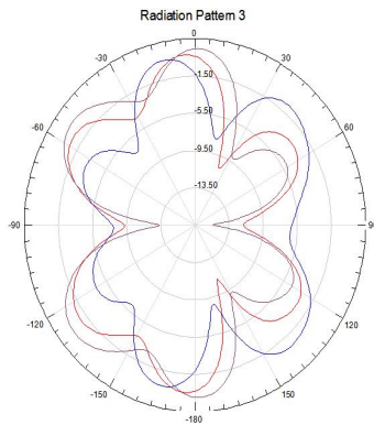
Radiation Pattern YOZ
