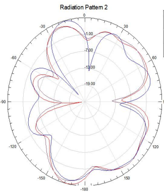
Radiation Pattern XOY
