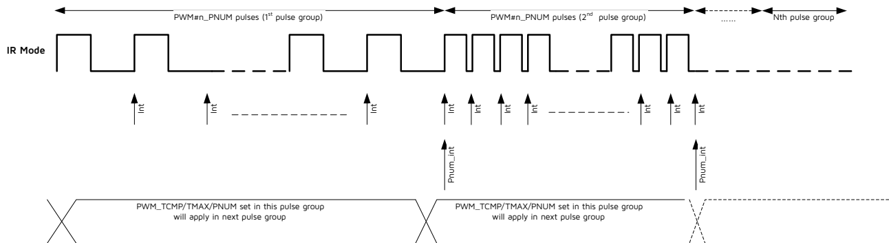
Figure 12-5 IR Mode (n=0)
