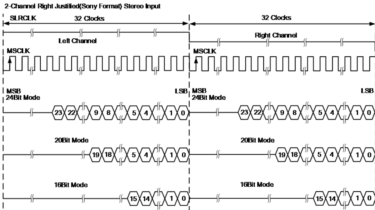
Figure 11-12 Timing Diagram of RJ Format
