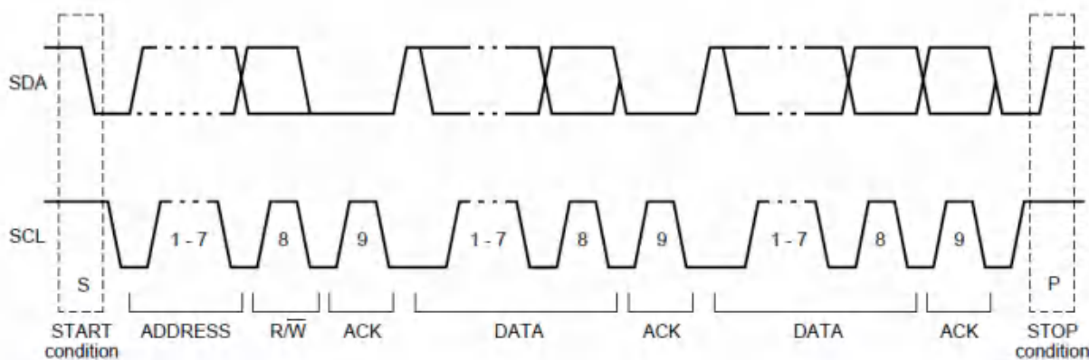
Figure 11-6 I2C Timing
