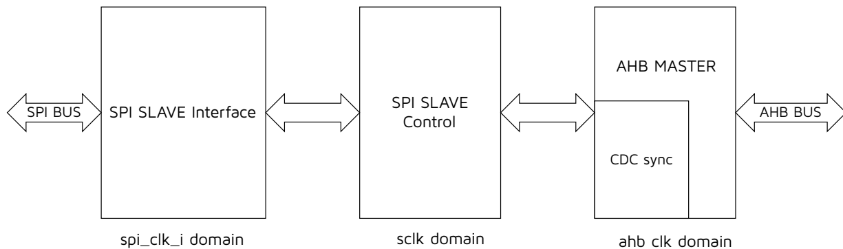
Figure 11-20 SPI_SLV Diagram
