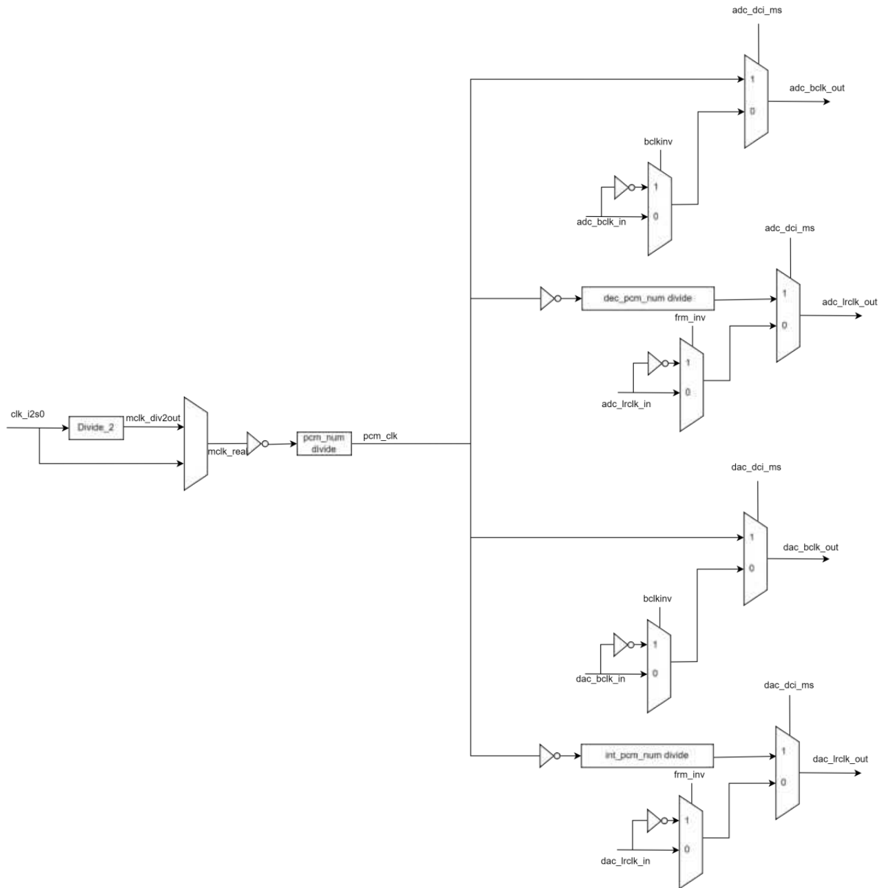
Figure 11-15 Clock Tree of I2S0 Module
