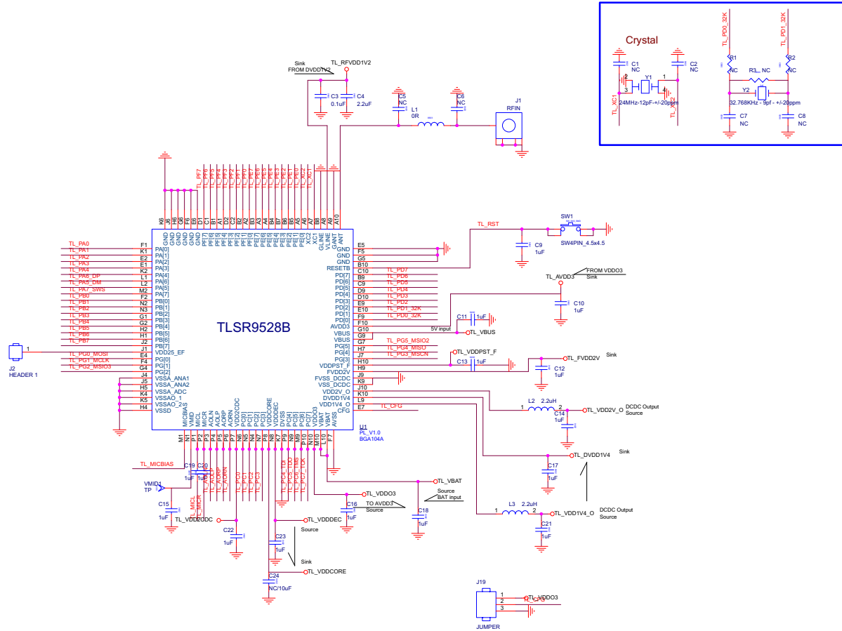
Figure 3-2 Reference Schematic of TLSR9528B
