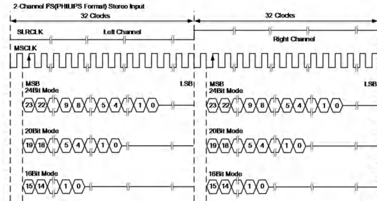
Figure 11-10 Timing Diagram of I2S Format
