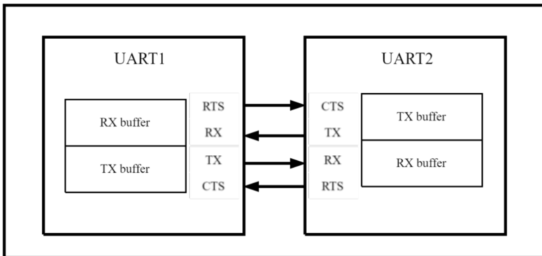
Figure 11-25 Hardware Flow Control between 2 UARTs
