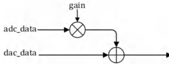
Figure 5-8 Sidetone Structure
