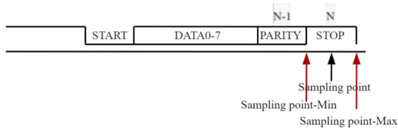
Figure 11-24 UART Protocol Formats and Sampling Point
