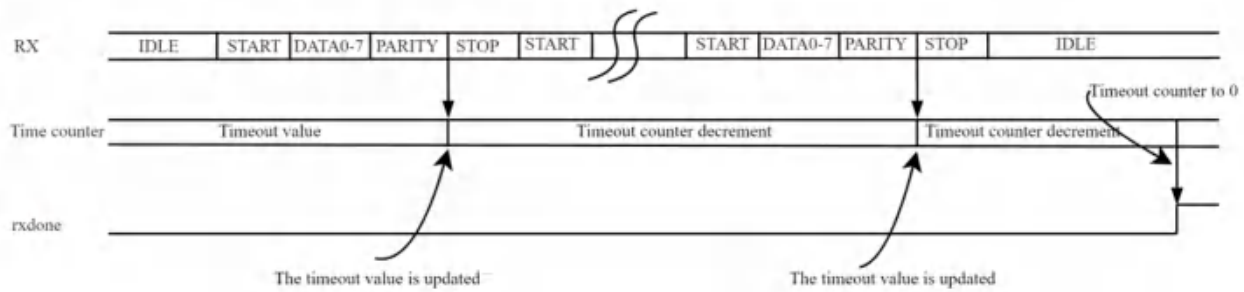
Figure 11-26 Timeout Flag Used for Data Transmission
