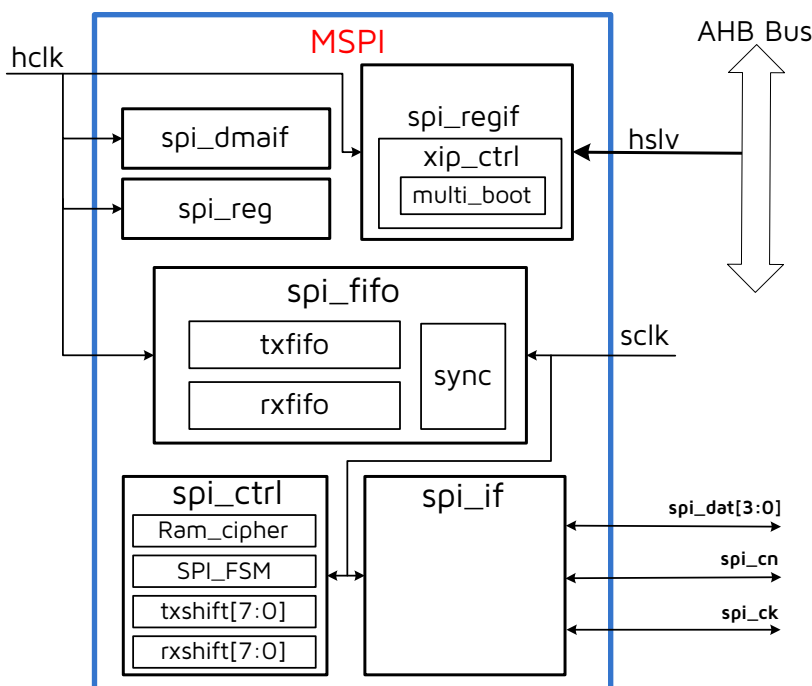
Figure 11-17 Memory SPI Diagram
