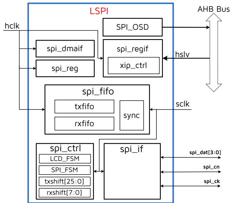
Figure 11-18 LSPI Diagram
