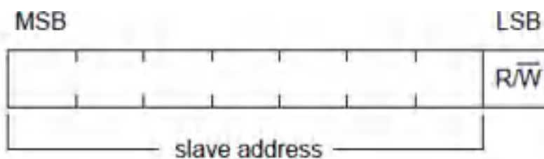
Figure 11-7 Byte Consisted of Slave Address and R/W Flag Bit
