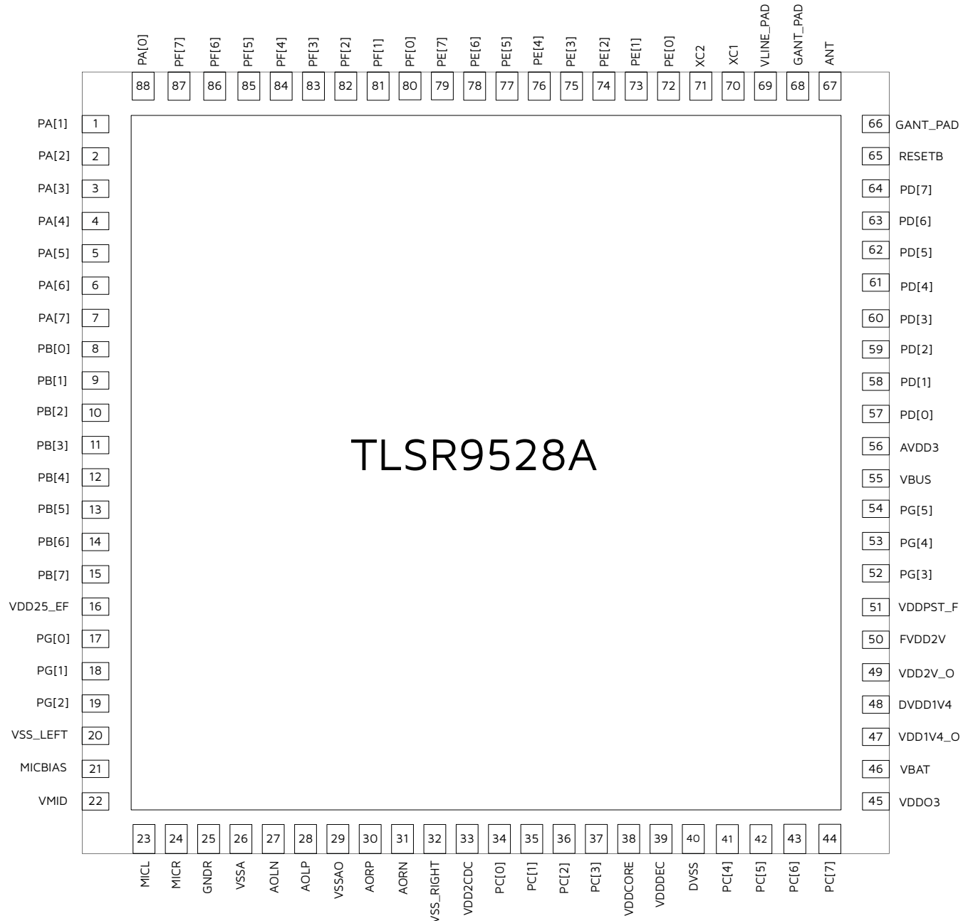
Figure 1-4 Pin Assignment of TLSR9528A
