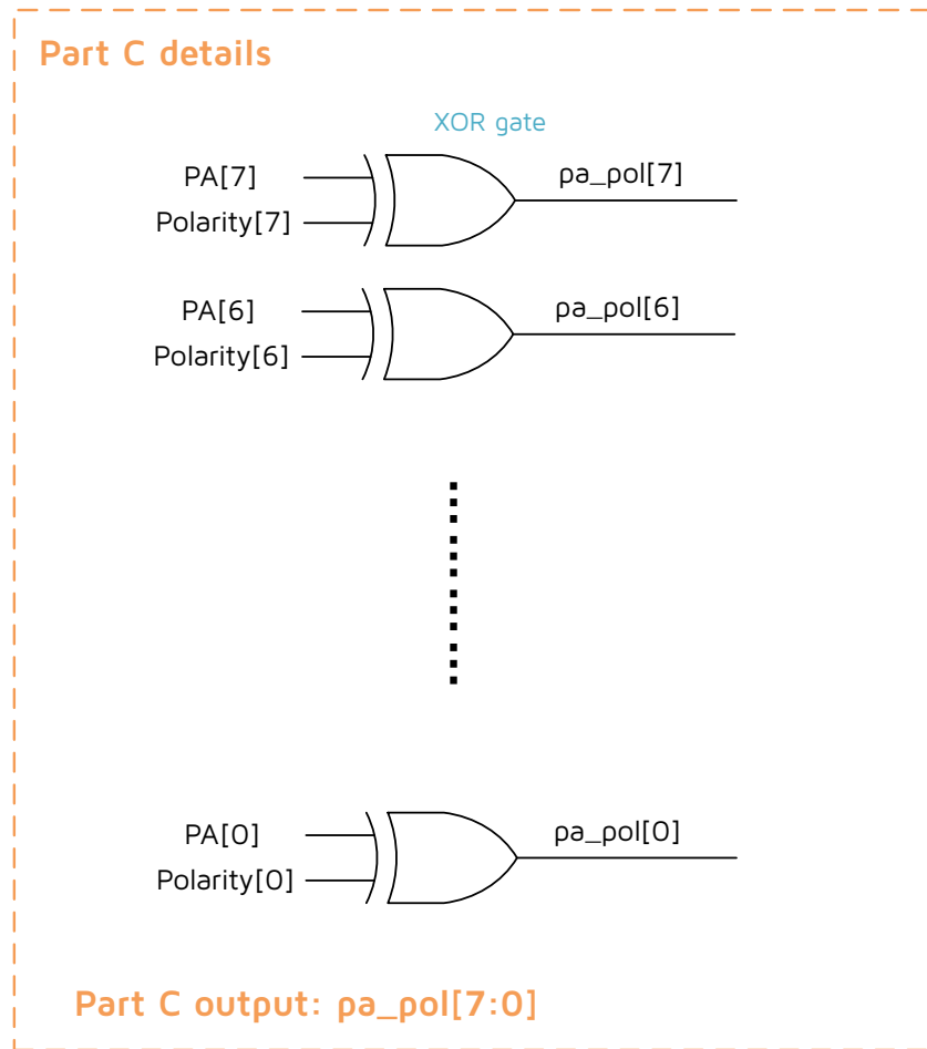
Figure 11-4 Detailed Circuit of Part C
