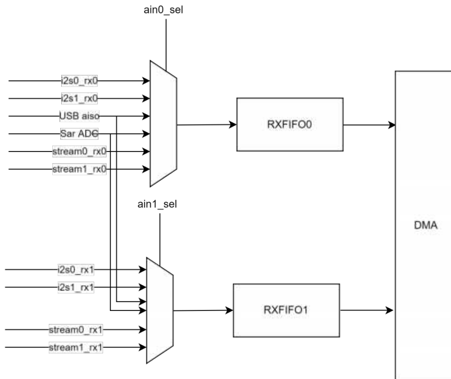
Figure 5-10 RXFIFO Input
