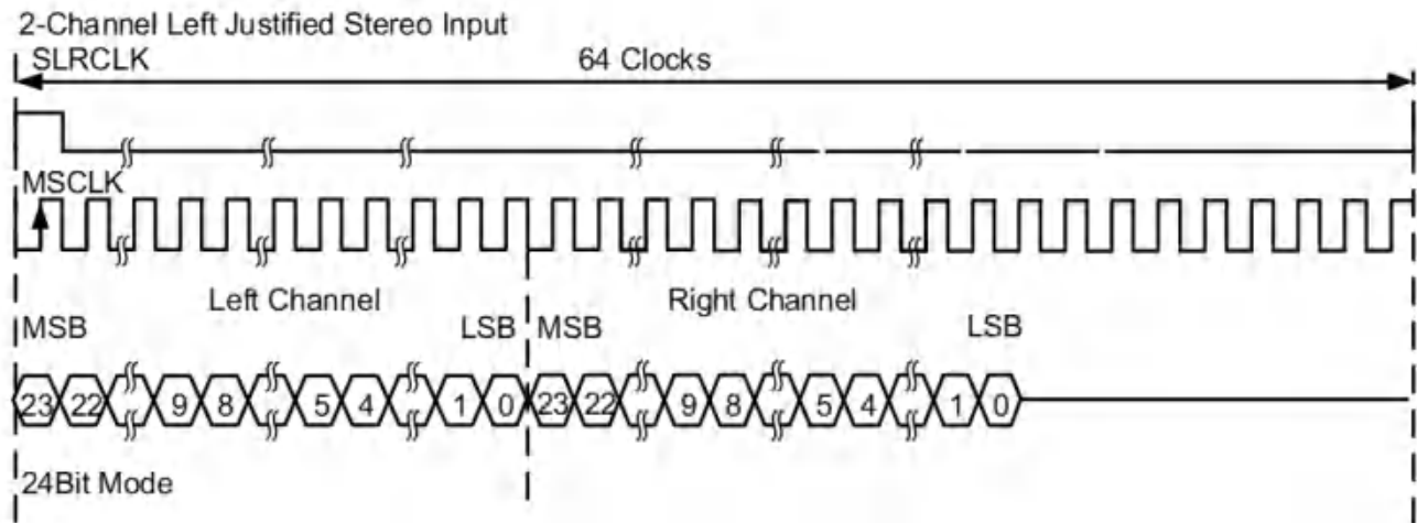
Figure 11-13 Timing Diagram of DSP Format Mode A
