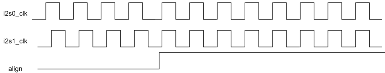
Figure 11-16 Phase Relationship between i2s0_clk and i2s1_clk
