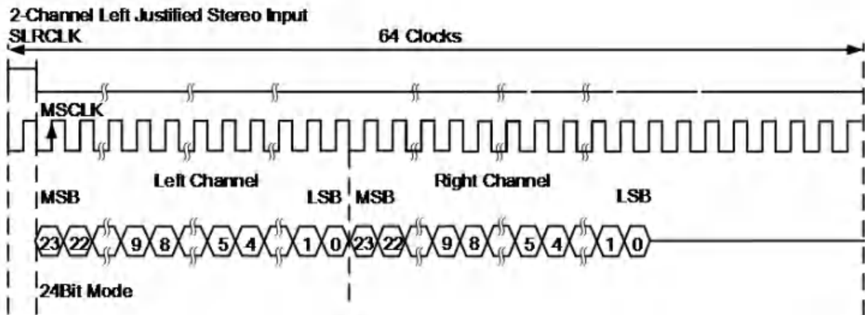
Figure 11-14 Timing Diagram of DSP Format Mode B
