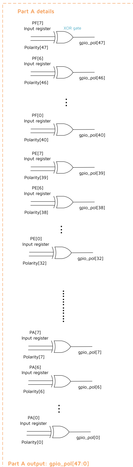
Figure 11-2 Detailed Circuit for Part A
