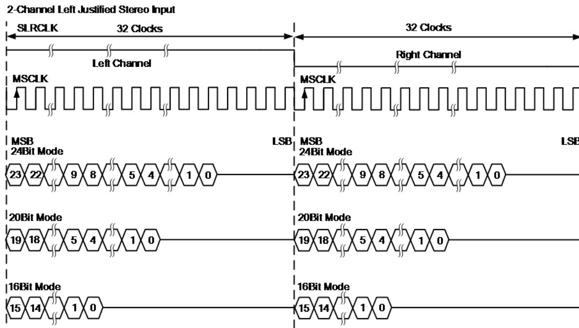
Figure 11-11 Timing Diagram of LJ Format
