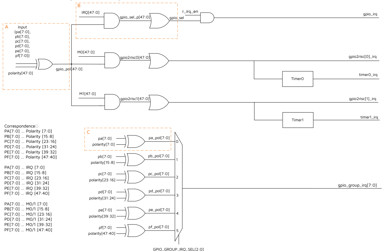
Figure 11-1 Logic Relationship between GPIO and Related Modules
