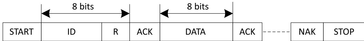
Figure 11-9 Write Format in Slave Mode
