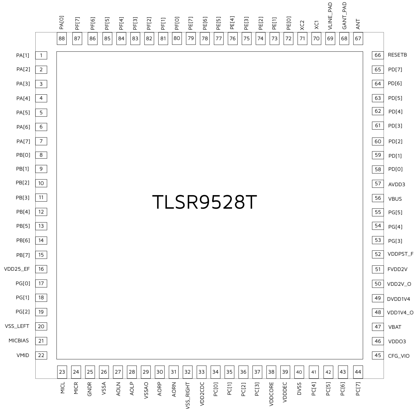
Figure 1-6 Pin Assignment of TLSR9528T
