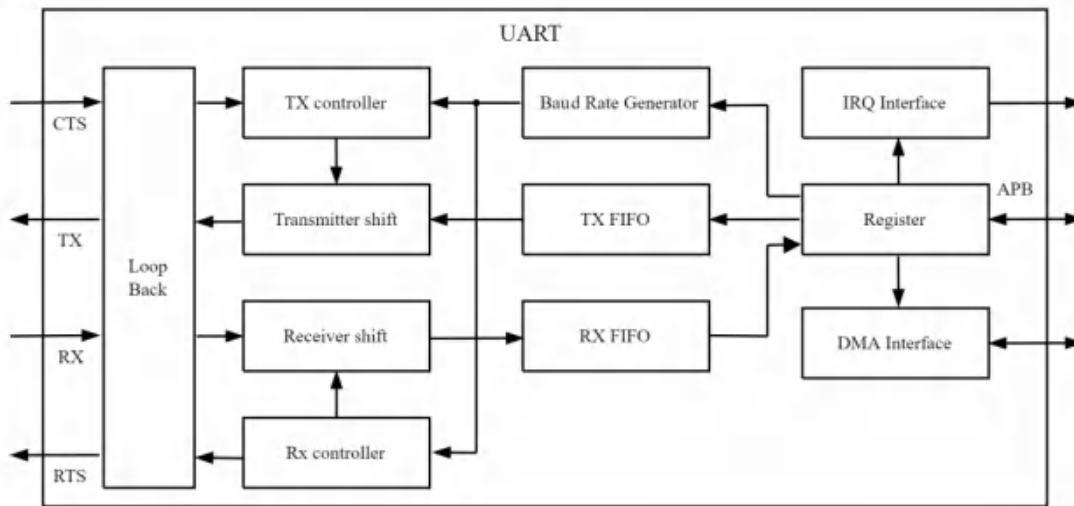
Figure 11-23 Block Diagram of UART
