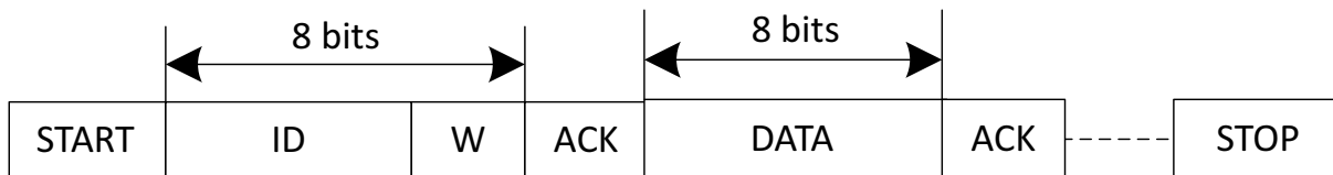
Figure 11-9 Write Format in Slave Mode
