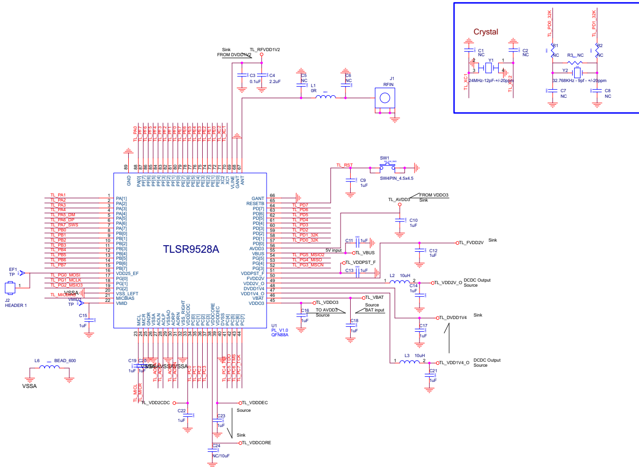
Figure 3-1 Reference Schematic of TLSR9528A
