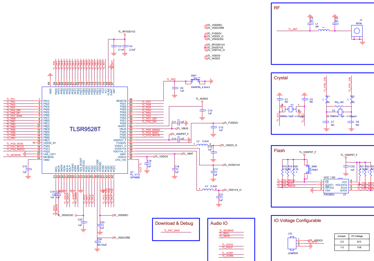
Figure 3-3 Reference Schematic of TLSR9528T
