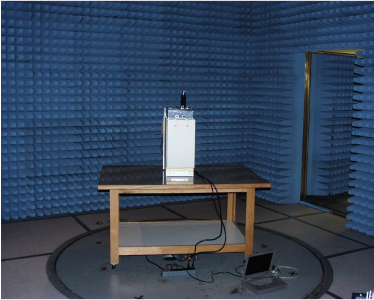
Back view of worst case radiated and line conducted emissions
