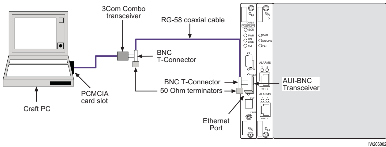
Figure 3. Connecting the Craft PC to the TurboMAX via the Ethernet Port
