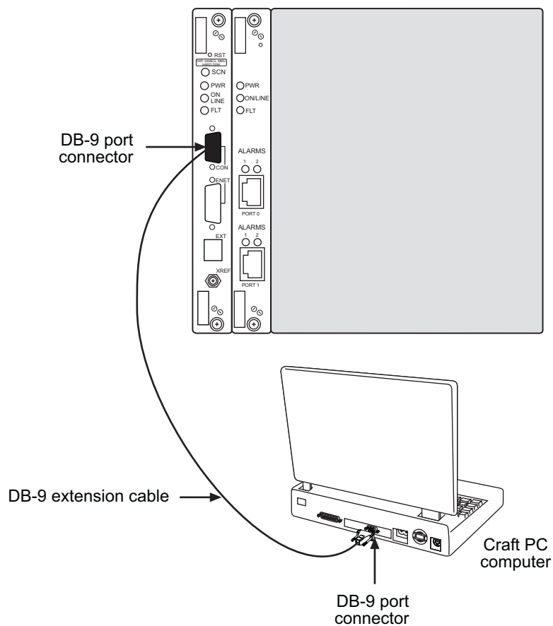
Figure 4. Connecting the Craft PC to the TurboMAX via the Serial Port
