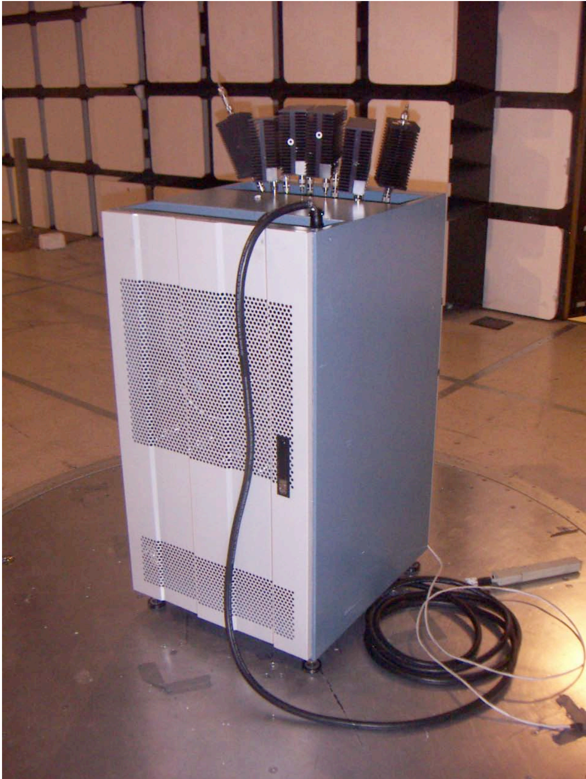
Rear View
