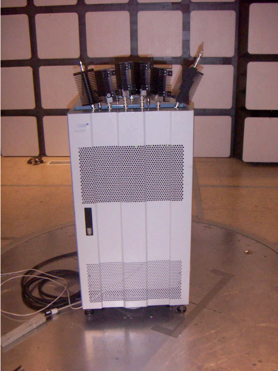
Front View
