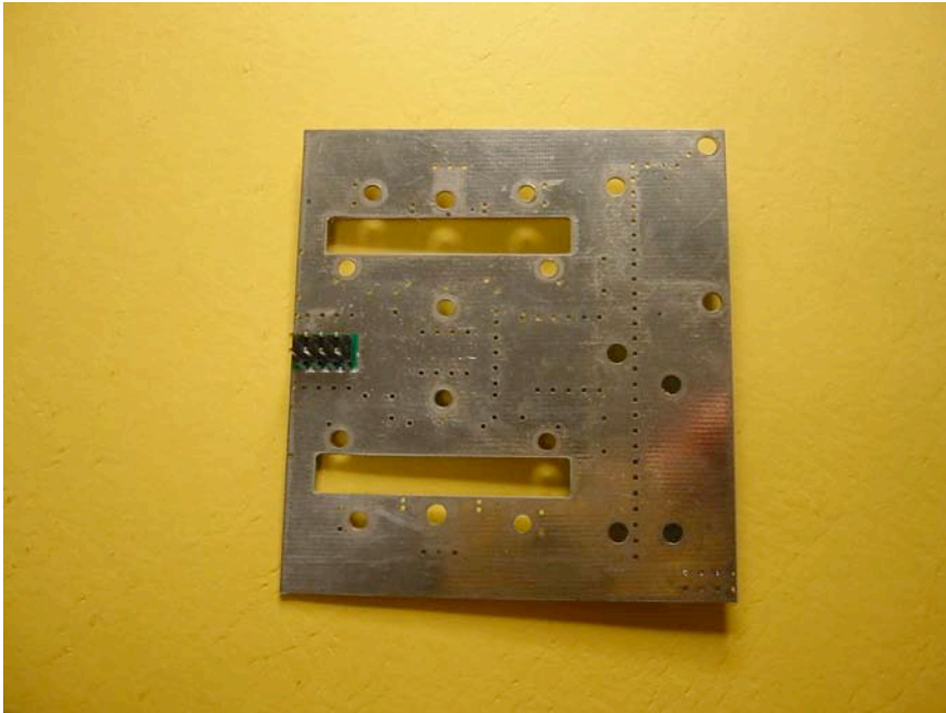
Combiner top
