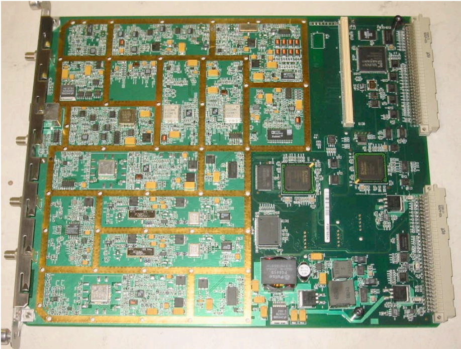
TRX board bottom
