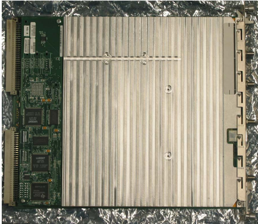
Radio Board 850TRX-Card, Side View #1
