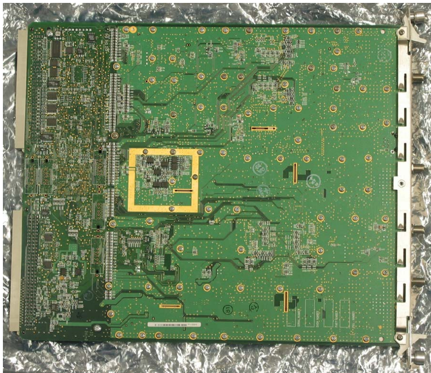
Radio Board 850TRX-Card, SideView #2
