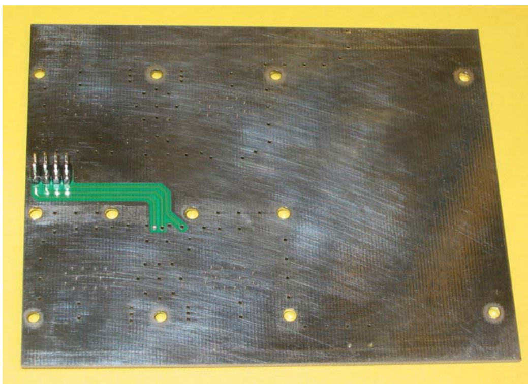
DSWR-Detector, PCB Back View (Reverse & Forward Power Detector)
