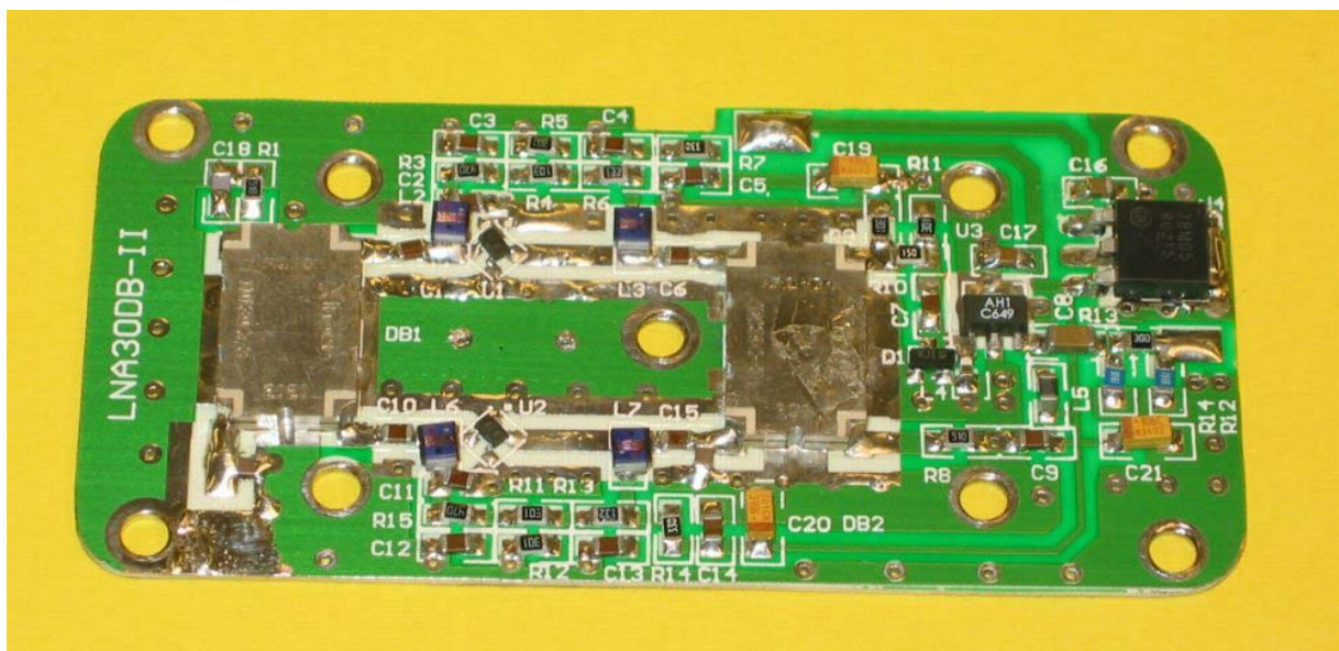
LNA, PCB Front View (Part of Duplexer Module)
