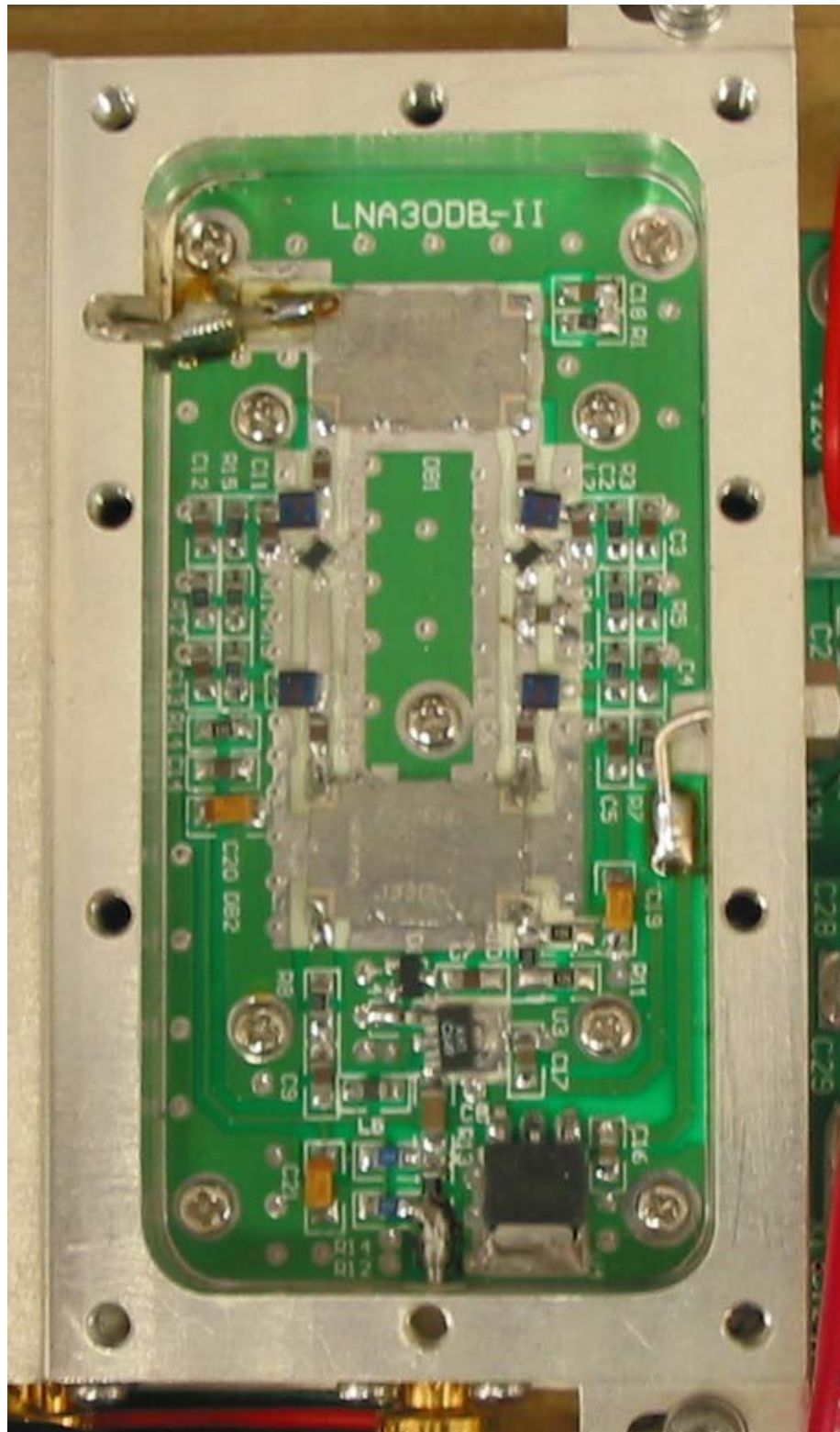
LNA (Part of Duplexer Module)
