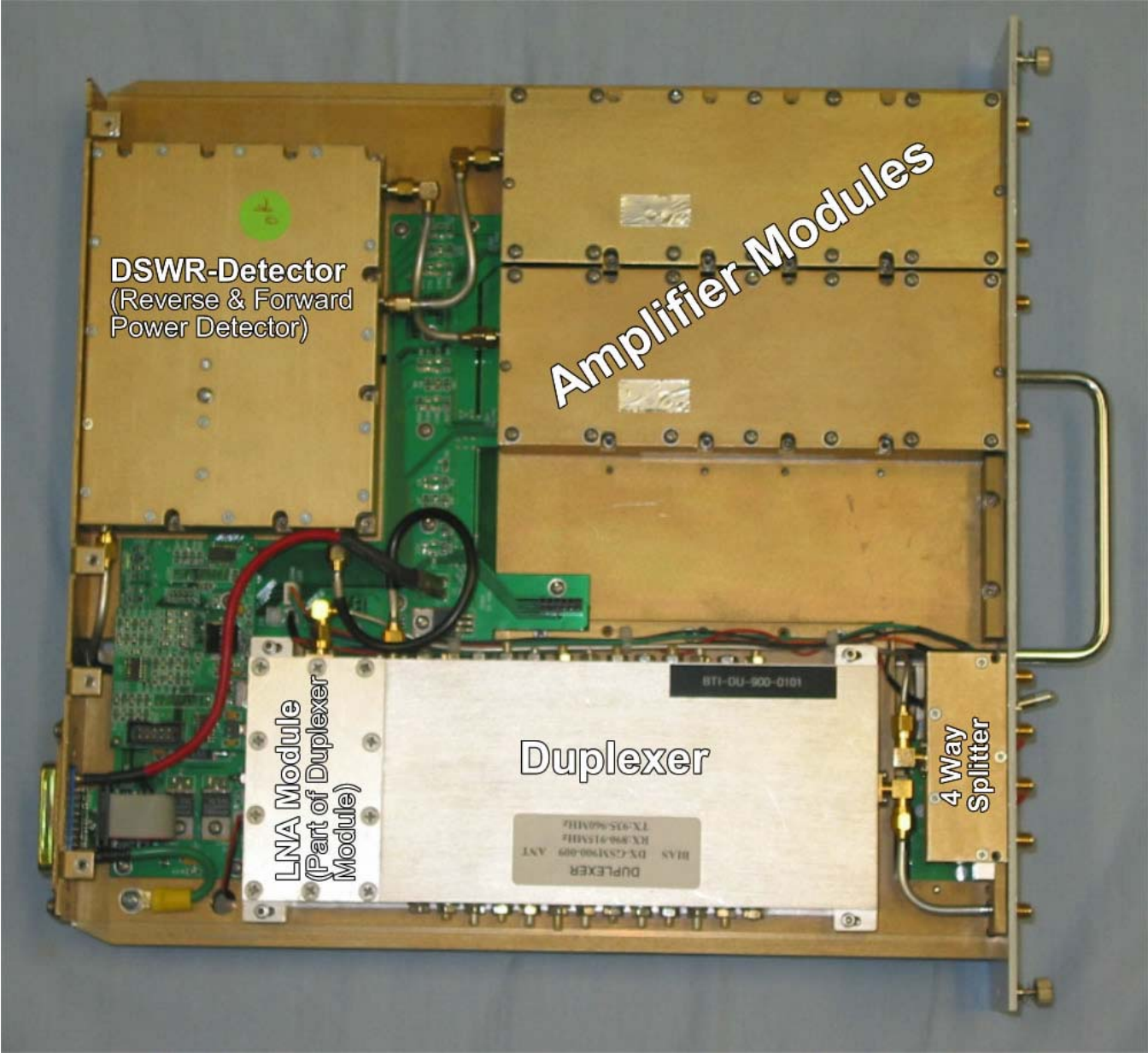
RF-Module, Internal Overview
