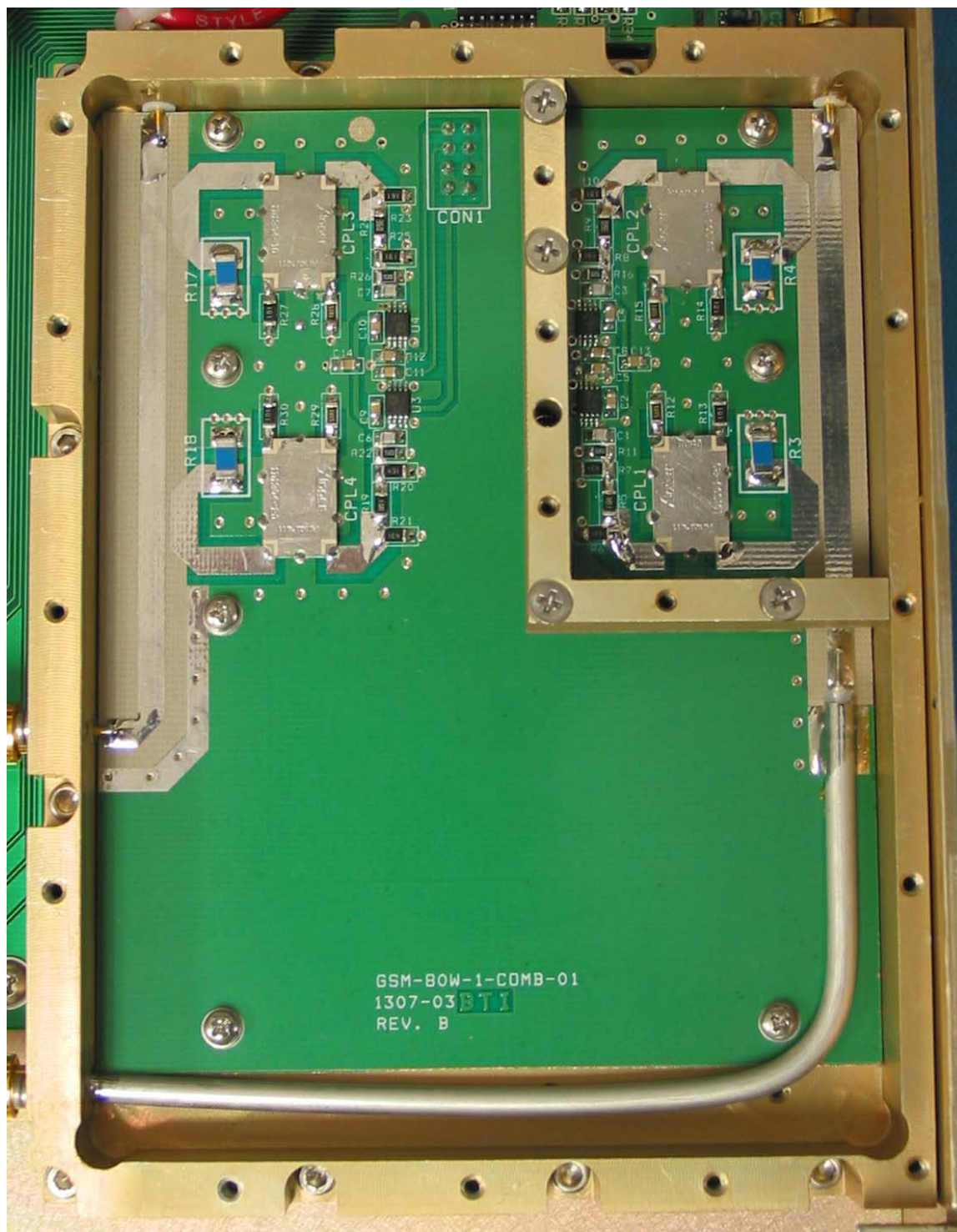
DSWR-Detector (Reverse & Forward Power Detector)
