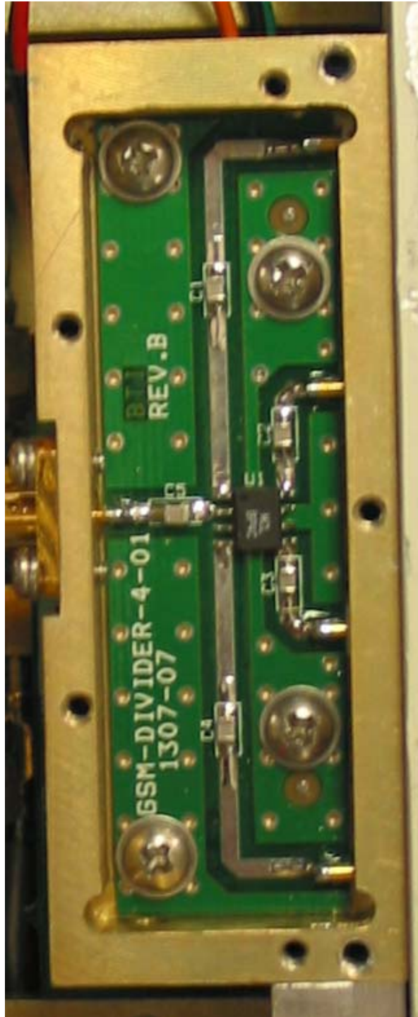
4 Way Splitter
