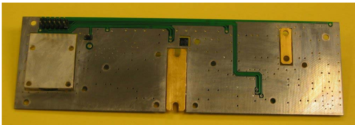
Amplifier, PCB Back View
