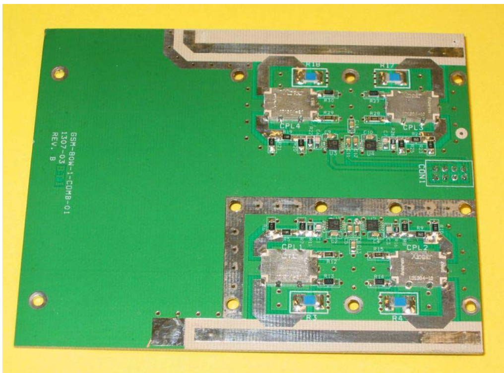
DSWR-Detector, PCB Front View (Reverse & Forward Power Detector)
