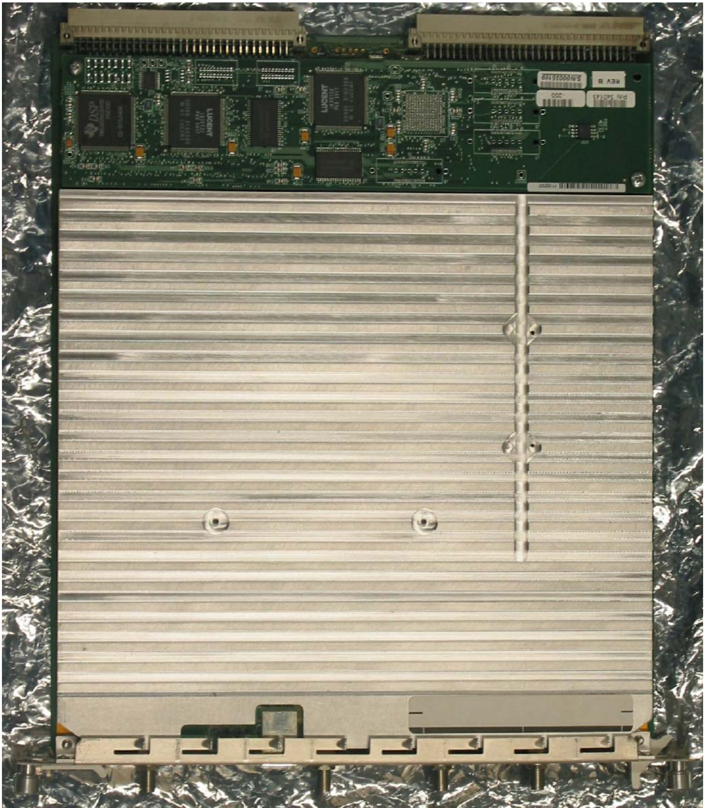
Radio Module, 850TRX-Card, Top Side, Overview
