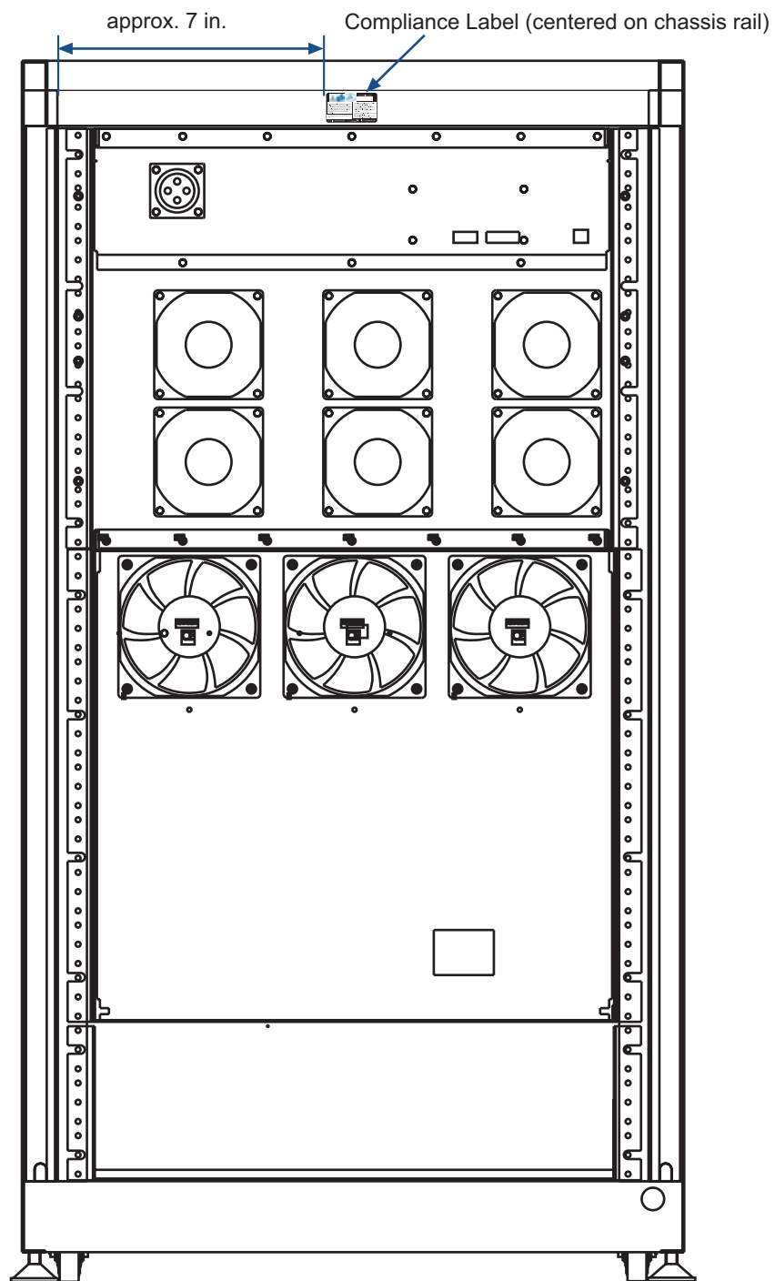
FCC label placement Rear of cabinet, door not shown
