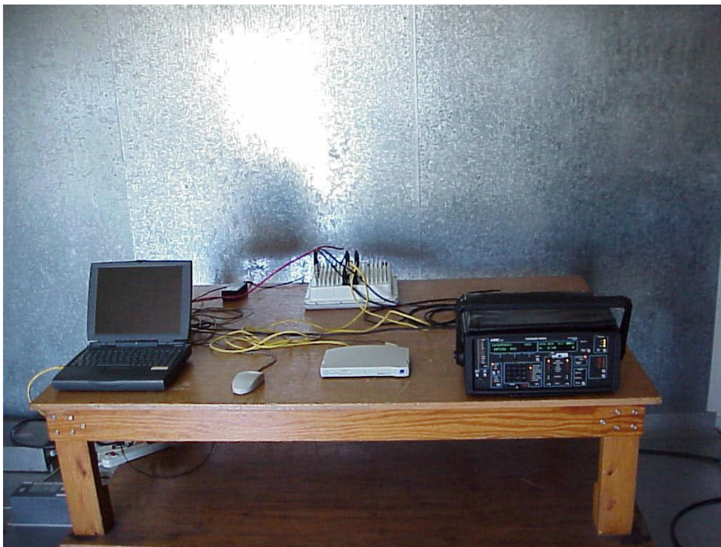
Link CX, AC Line conducted emissions setup photo
