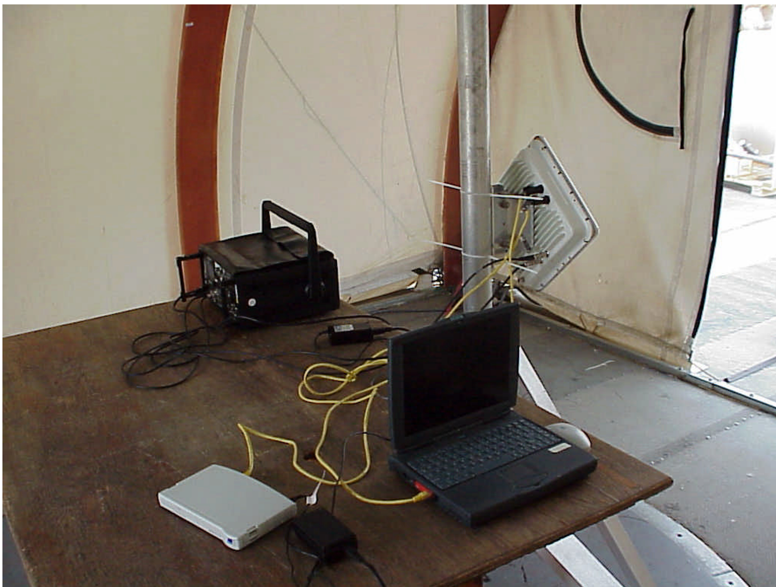
Link CX, 15.205 Radiated emissions, Restricted bands, setup
