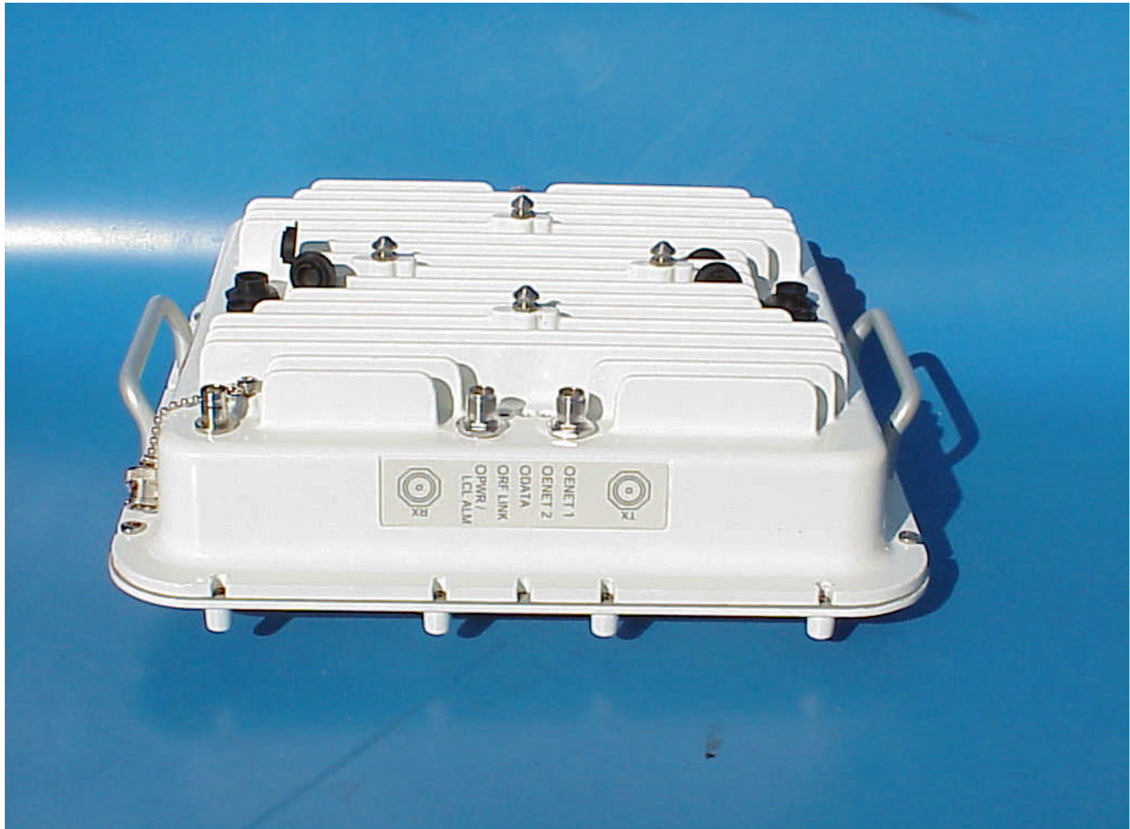
Link CX external side view showing DS3 connectors and LED windows
