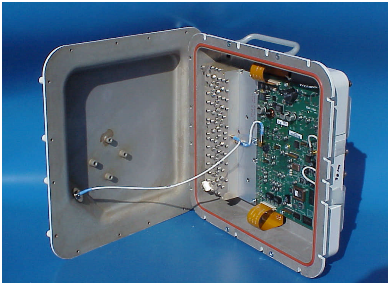
Link CX antenna cable attachment (external antenna configuration, 5.8 GHz versions only)
