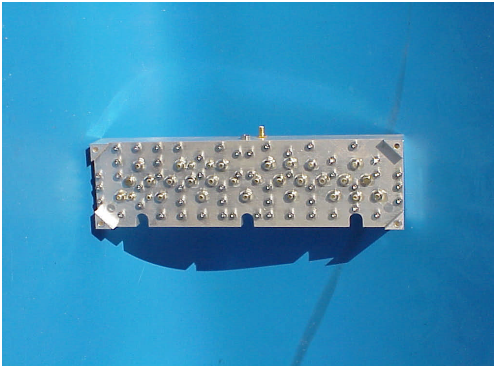
Link CX duplexer, top view
