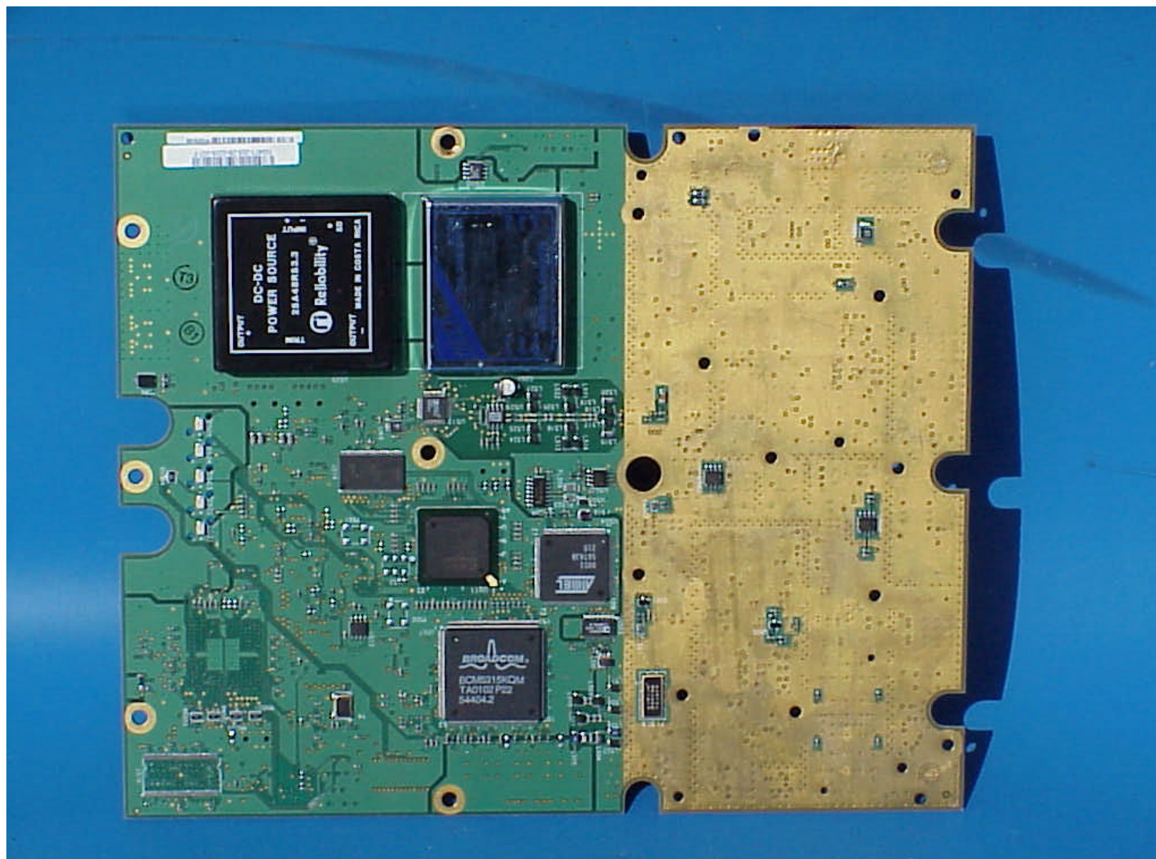
Link CX pcb bottom view without shields
