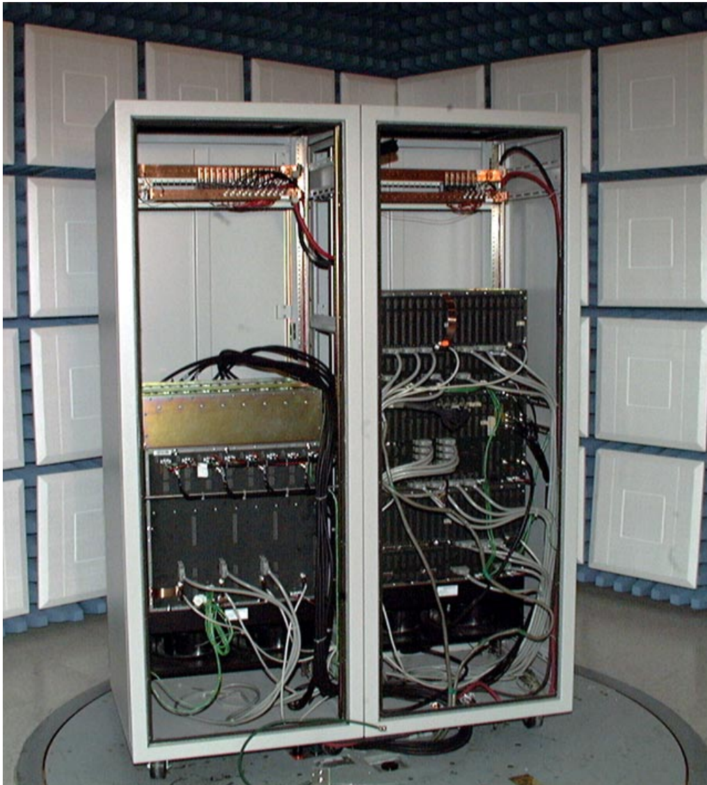
Figure 4.2 Open doors rear view of PWAN Base Station
