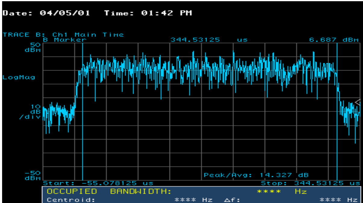
Figure 11.49 Time-Domain Power Envelope, Peak/Average Ratio at \leq 99.0\% Occurrence — Block B
