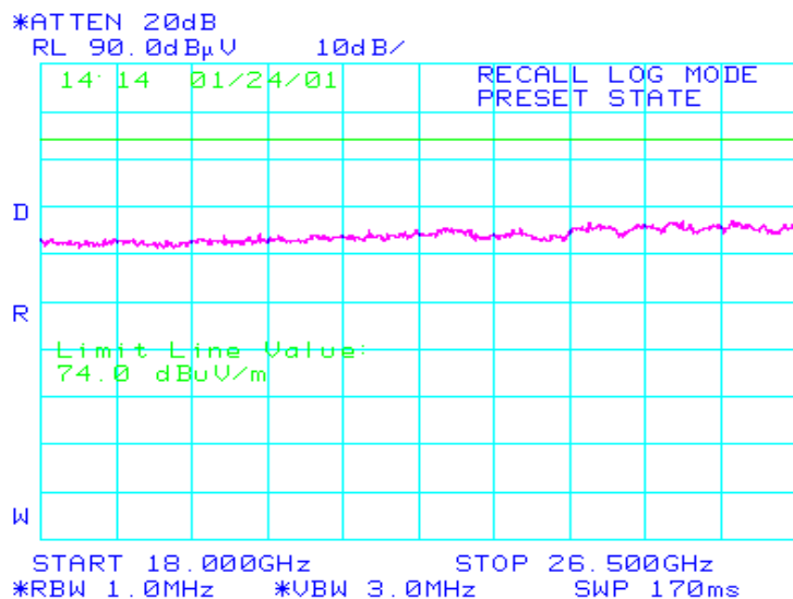
Figure 11.97 18.0 GHz – 26.5GHz @ 1.5-m Antenna Height Emissions Scan, Horizontal Polarization
