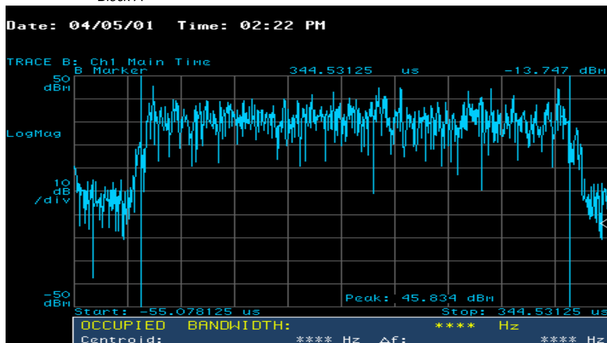
Figure 11.45 Time-Domain Power Envelope, Peak Power at \leq 99.0\% Occurrence —Block A
