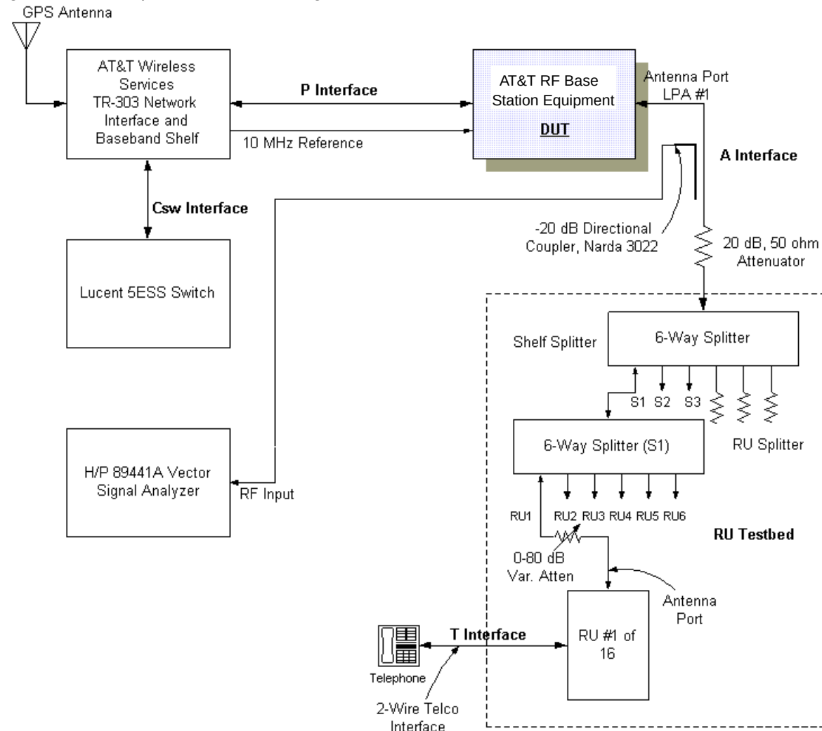
Figure 11.6 Output Power Test Configuration
