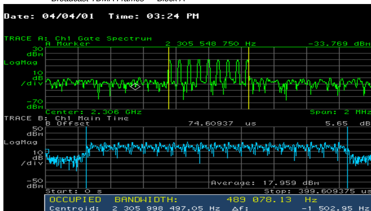
Figure 11.28 Time-Keyed Remote Synchronization Pilots Power vs. Frequency, 99.0% Occupied Bandwidth, and Time-Domain Average Burst Power During Broadcast TDMA Frames — Block A
