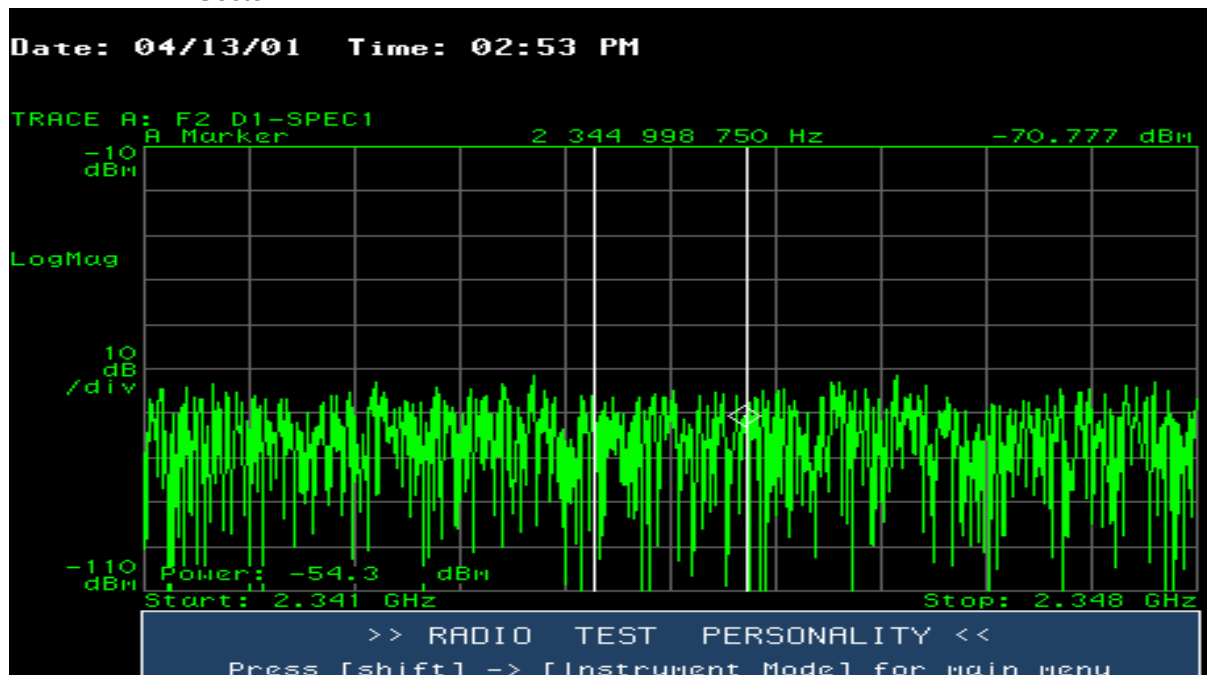
Figure 11.78 7 MHz Upper Guard Band Between 2341 MHz and 2348 MHz — Sector D
