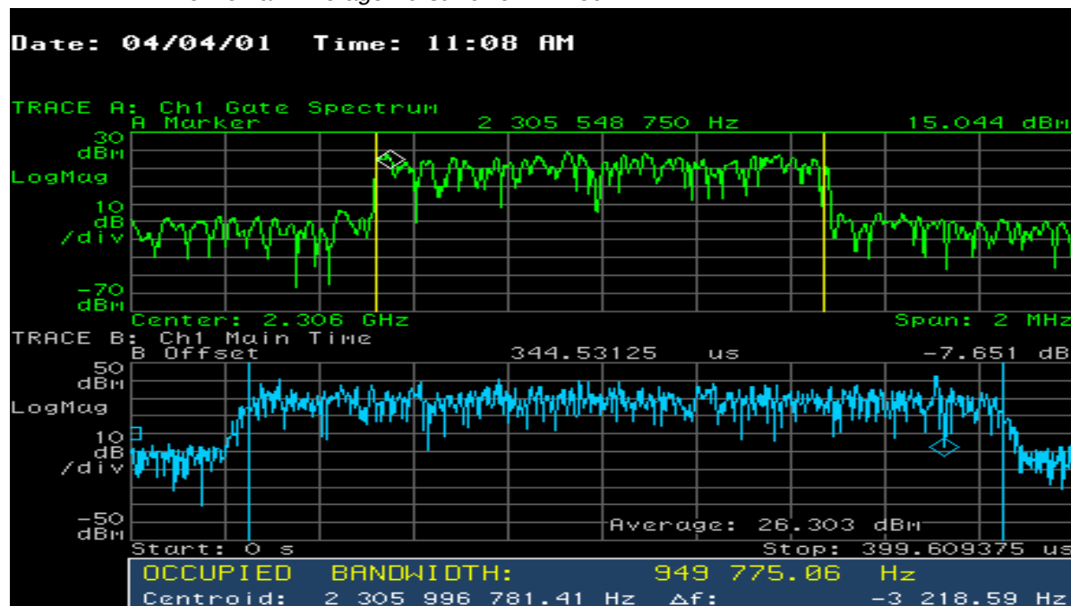
Figure 11.22 High-Speed Data Channel Power vs. Frequency, 99% Occupied BW, and Time-Domain Average Burst Power — Block A
