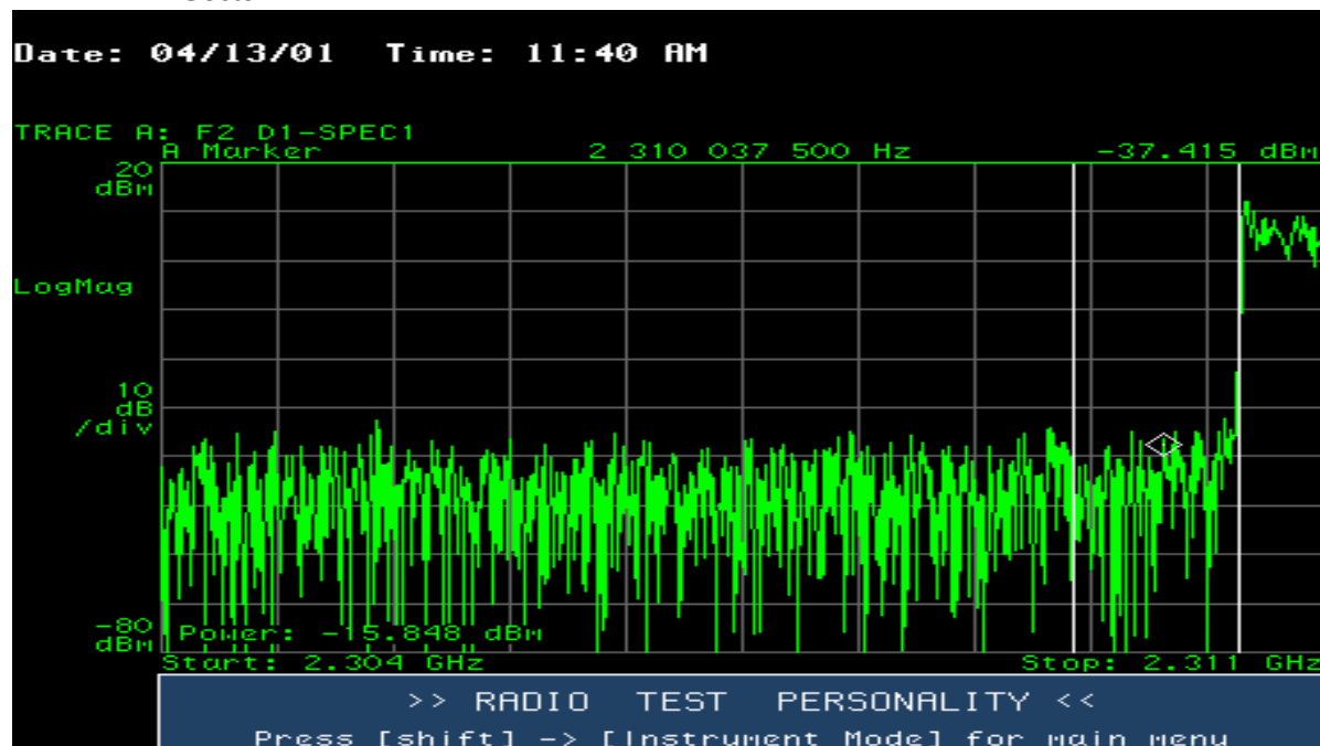
Figure 11.68 7 MHz Lower Guard Band Between 2309.5 MHz and 2310.5 MHz — Sector A
