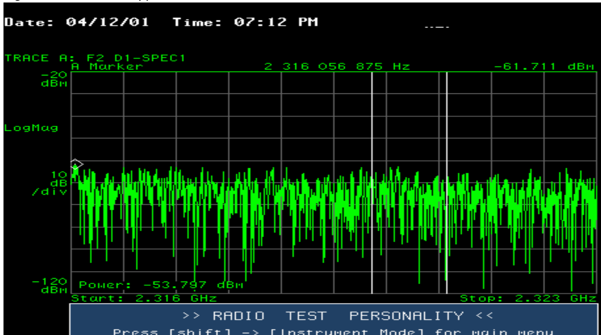
Figure 11.58 7 MHz Upper Guard Band Between 2316 MHz and 2323 MHz — Sector D
