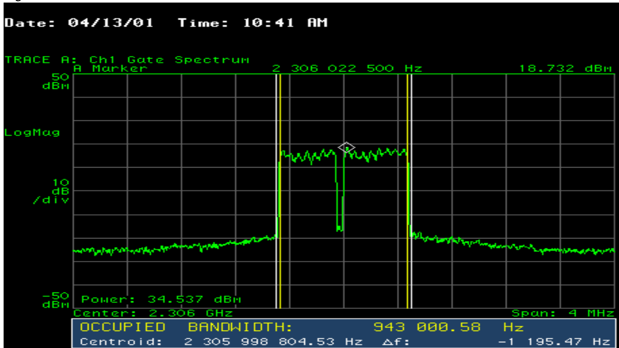
Figure 11.50 1 MHz Band-Power Between 2305.5 and 2306.5 MHz — Sector A
