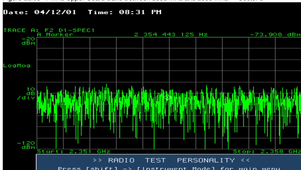
Figure 11.63 7 MHz Upper Guard Band Between 2351 MHz and 2358 MHz — Sector D
