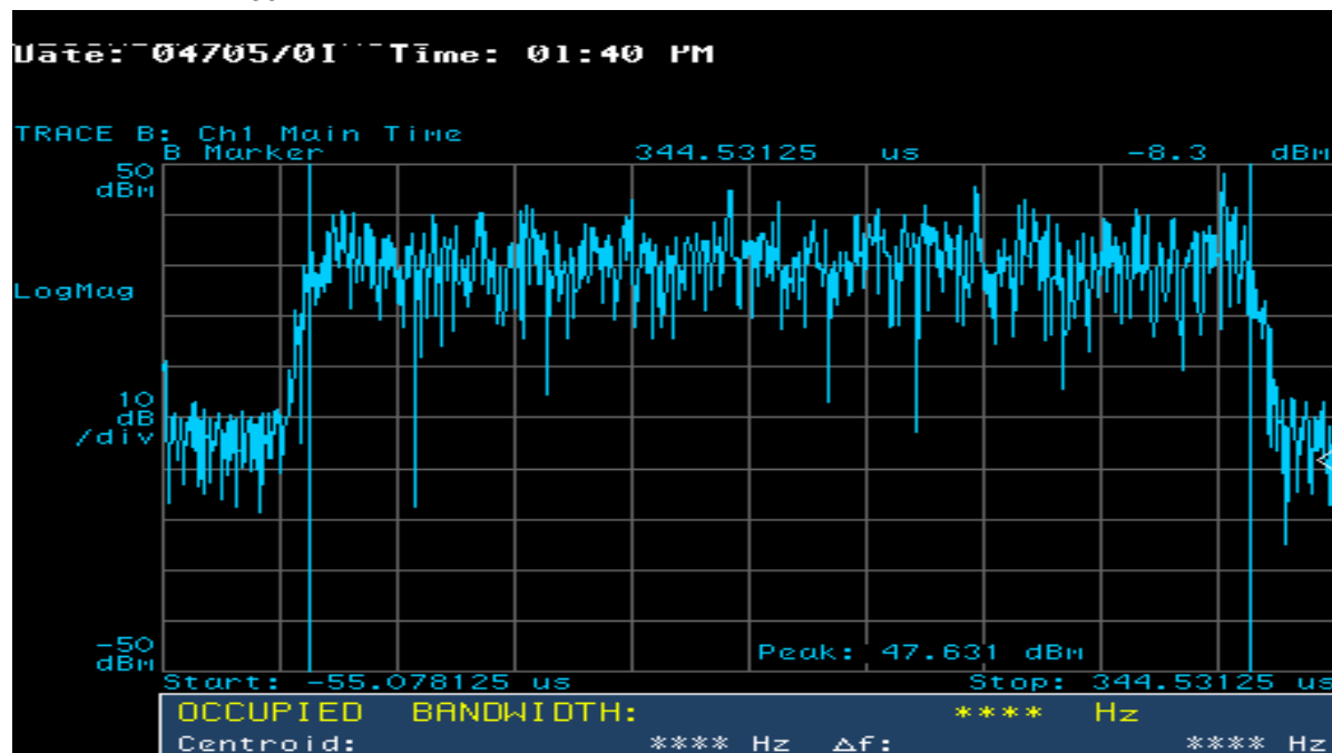
Figure 11.48 Time-Domain Power Envelope, Peak Power at \leq 99.0\% Occurrence — Block B
