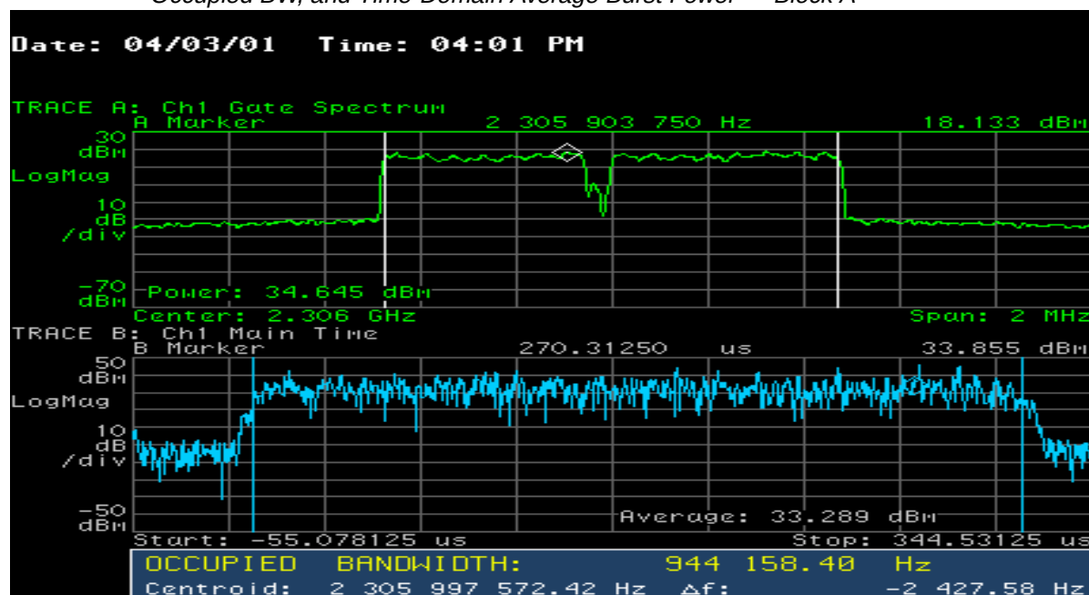
Figure 11.20 Fifteen Simultaneous — Voice Channel Power vs. Frequency, 99.0% Occupied BW, and Time-Domain Average Burst Power — Block A
