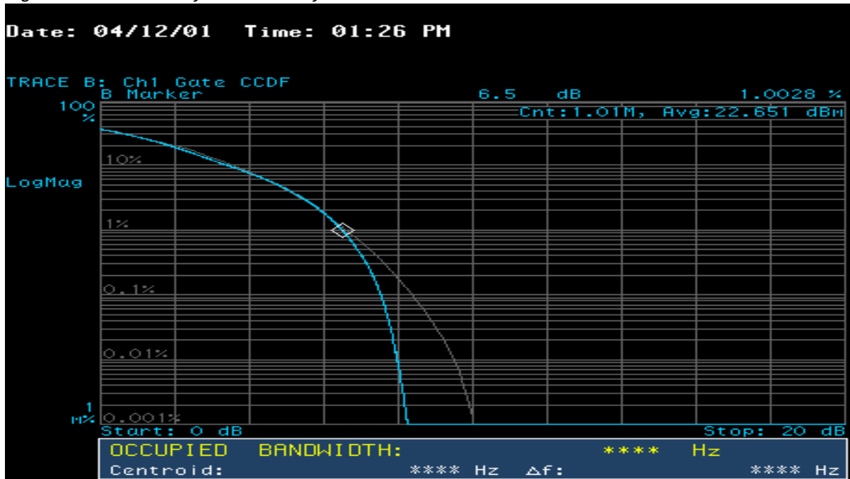
Figure 11.29 Time-Keyed Remote Synchronization Pilots Channel CCDF — Block A
