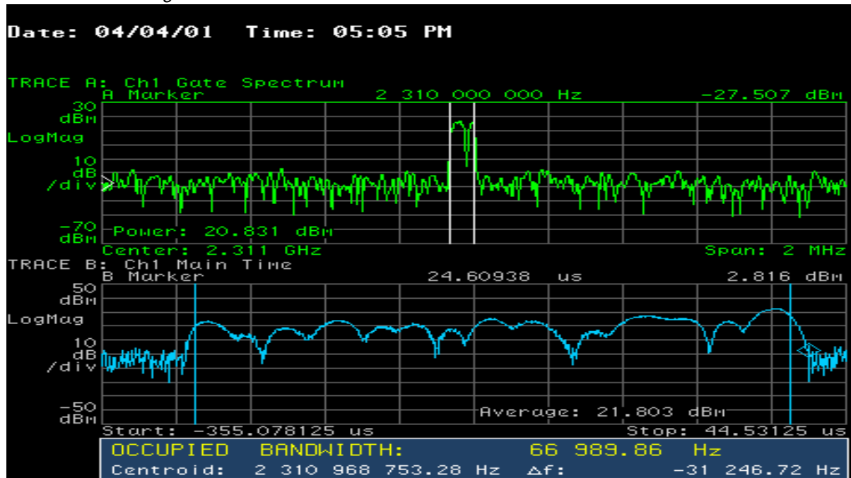
Figure 11.38 NAC Channel Power vs. Frequency, 99% Occupied BW, and Time-Domain Average Power — Block B
