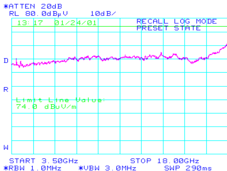
Figure 11.87 3.5 GHz – 18 GHz @1-m Antenna Height Emissions Scan, Horizontal Polarization
