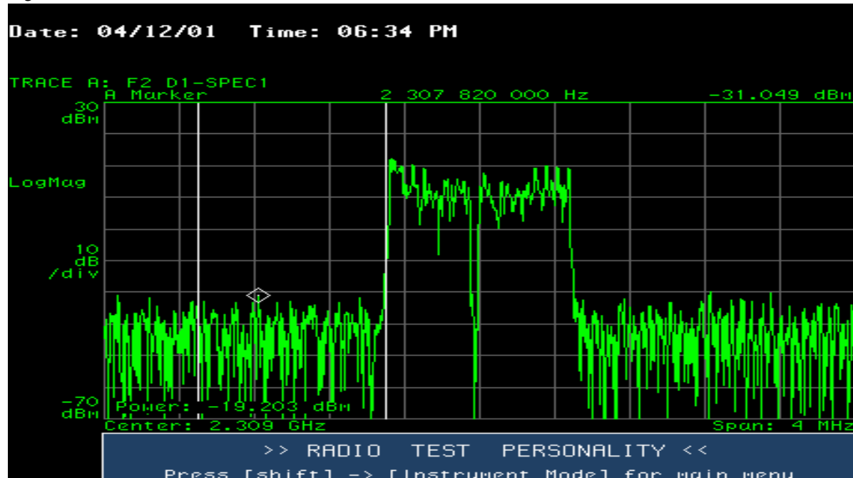
Figure 11.56 1 MHz Band Power Between 2307.5 and 2308.5 MHz — Sector D
