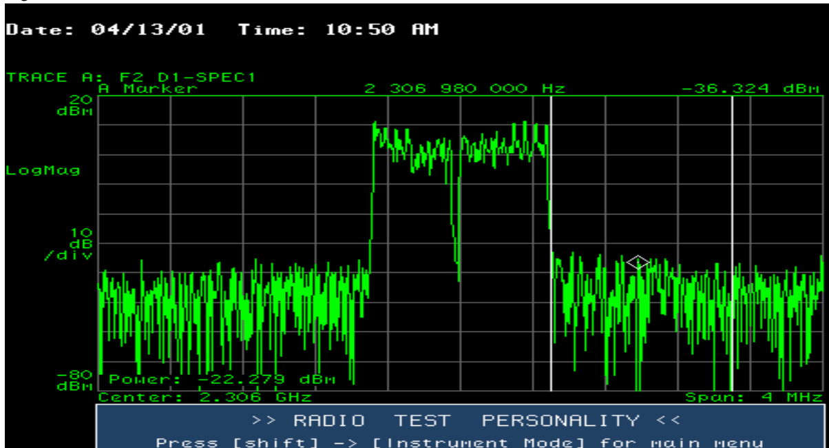
Figure 11.51 1 MHz Band Power Between 2306.5 and 2307.5 MHz — Sector A
