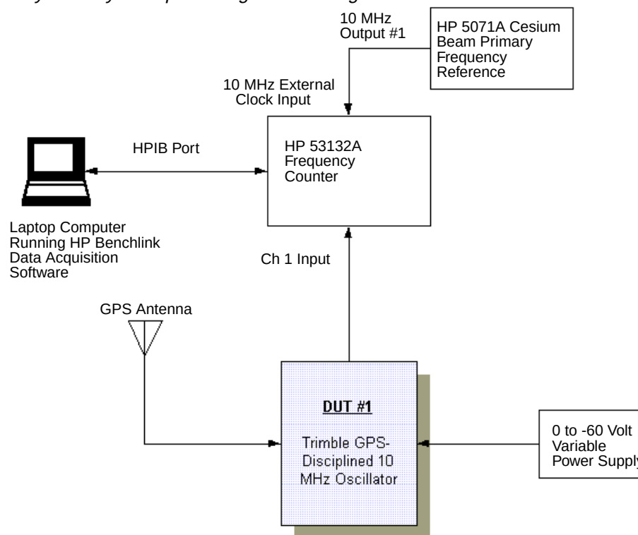
Figure 11.2 Frequency Stability vs. Input Voltage Test Configuration
