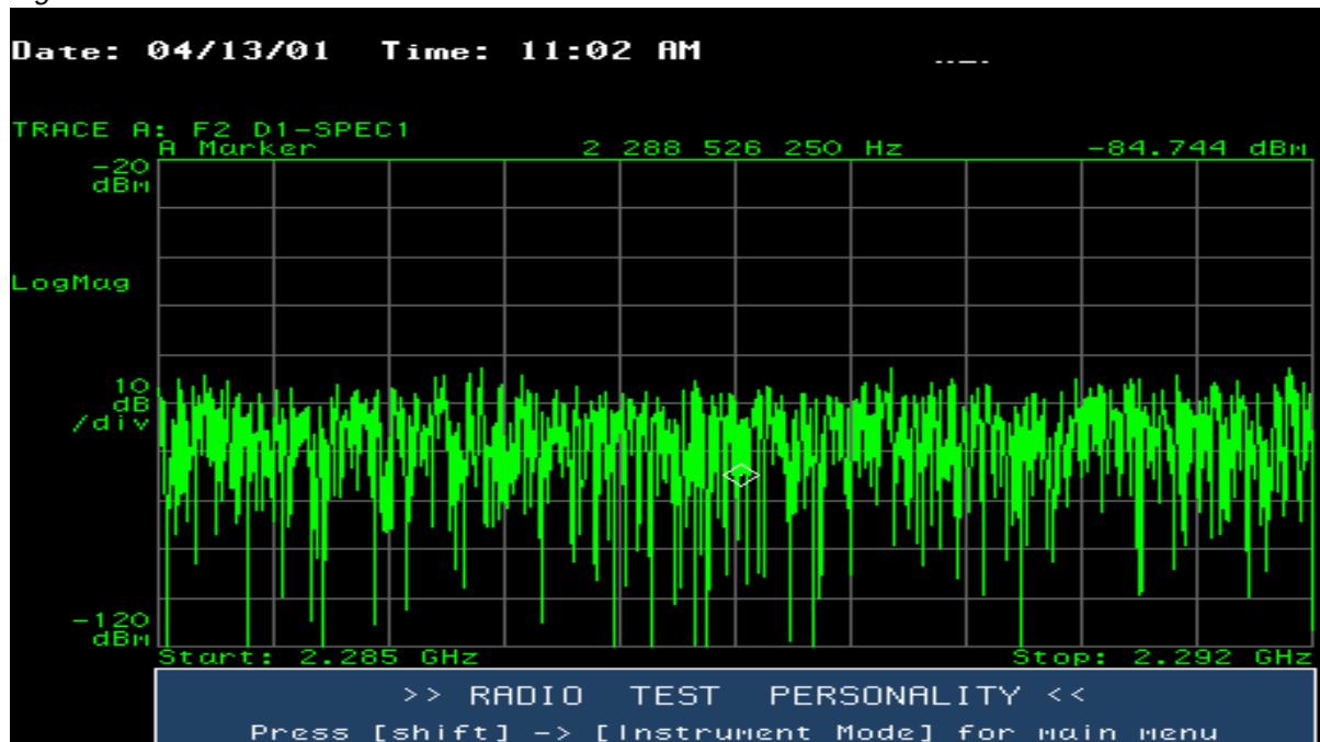
Figure 11.54 7 MHz Lower Guard Band Between 2285 MHz and 2292 MHz — Sector A
