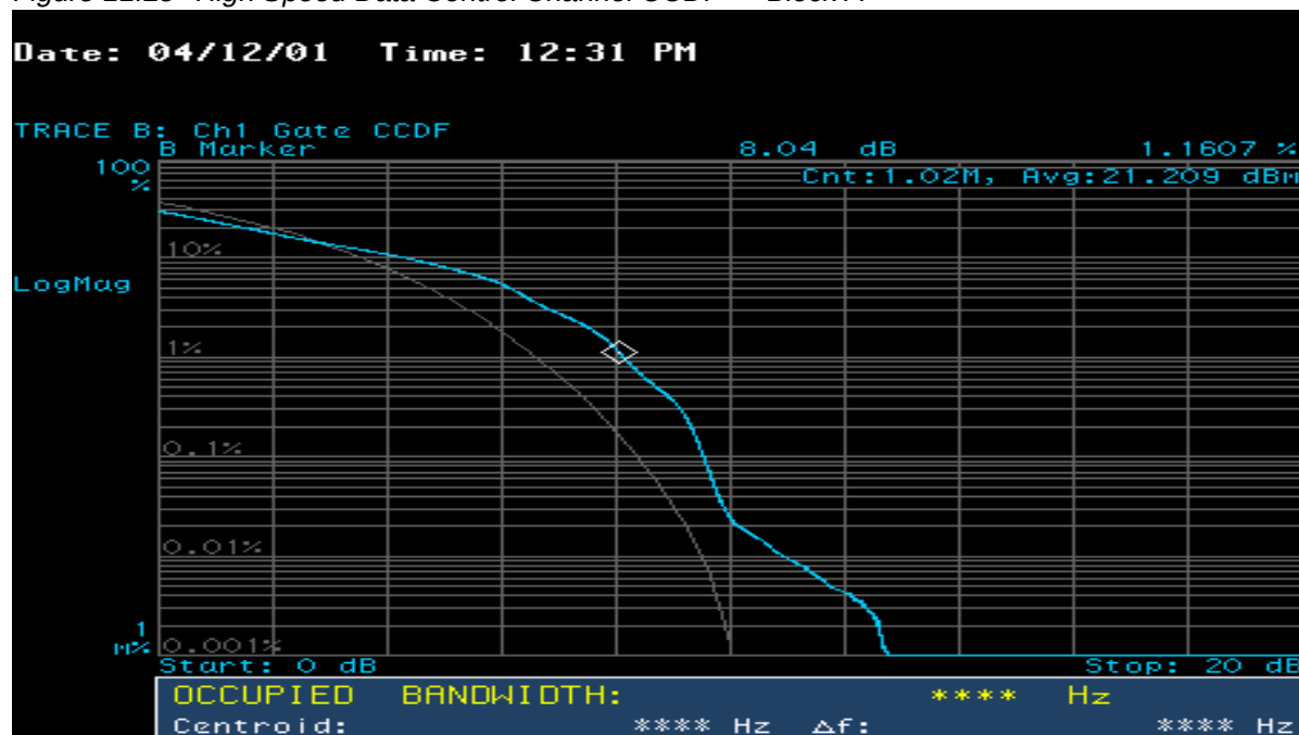
Figure 11.25 High Speed Data Control Channel CCDF — Block A
