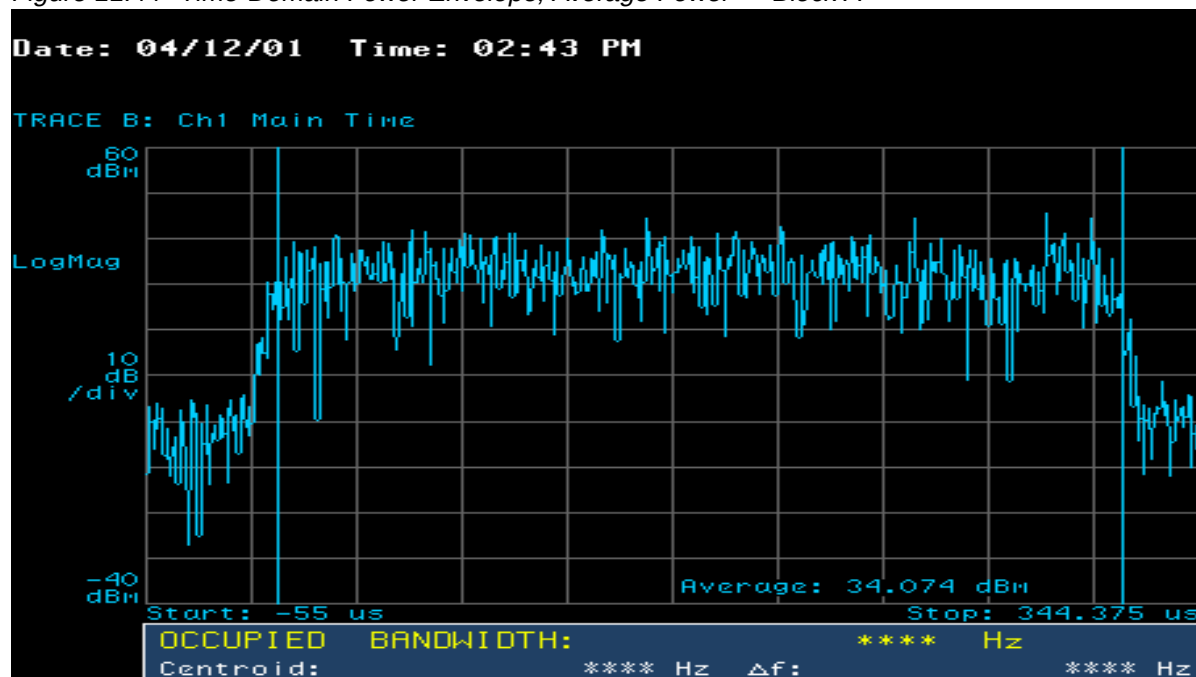
Figure 11.44 Time-Domain Power Envelope, Average Power — Block A
