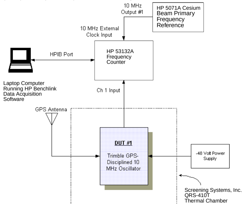
Figure 11.1 Frequency Stability vs. Temperature Test Configuration
