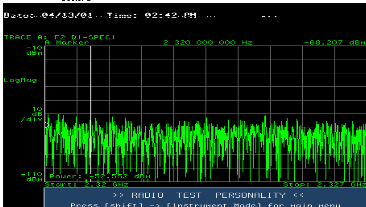
Figure 11.75 7 MHz Upper Guard Band Between 2320 MHz and 2327 MHz — Sector D
