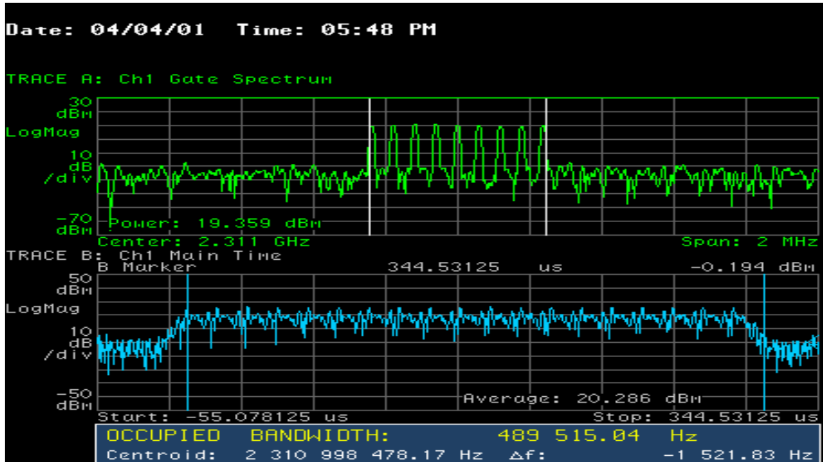
Figure 11.40 Time-Keyed Remote Synchronization Pilots Power vs. Frequency, 99.0% Occupied Bandwidth, and Time-Domain Average Burst Power During Broadcast TDMA Frames — Block B
