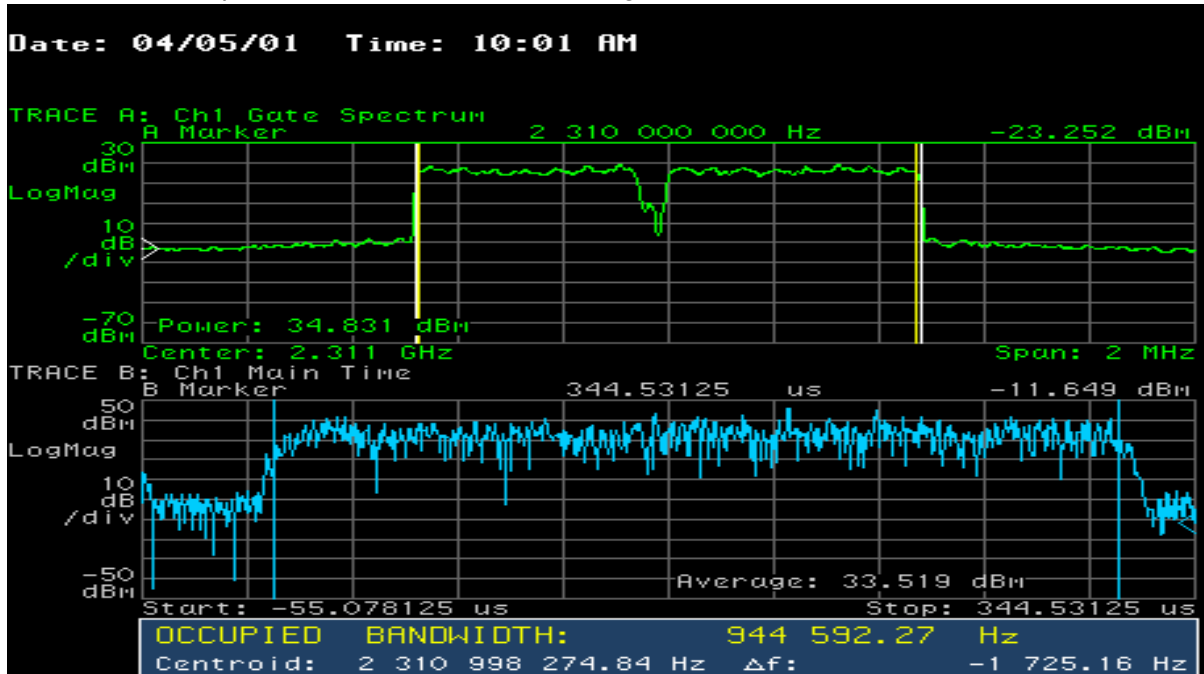
Figure 11.32 Fifteen Simultaneous — Voice Channel Power vs. Frequency, 99.0% Occupied BW, and Time-Domain Average Burst Power — Block B
