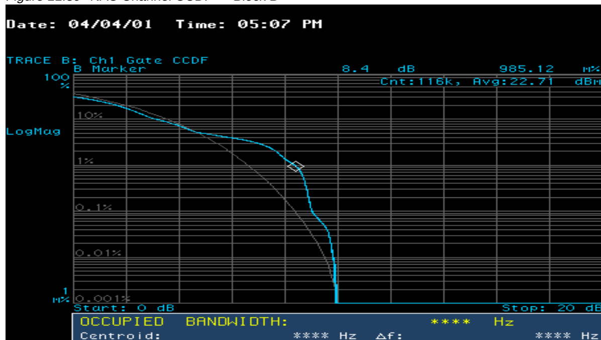
Figure 11.39 NAC Channel CCDF — Block B
