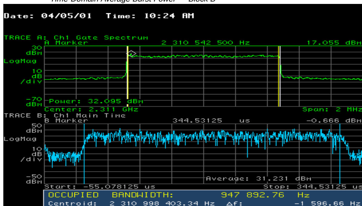
Figure 11.34 High-Speed Data Channel Power vs. Frequency, 99% Occupied BW, and Time-Domain Average Burst Power — Block B
