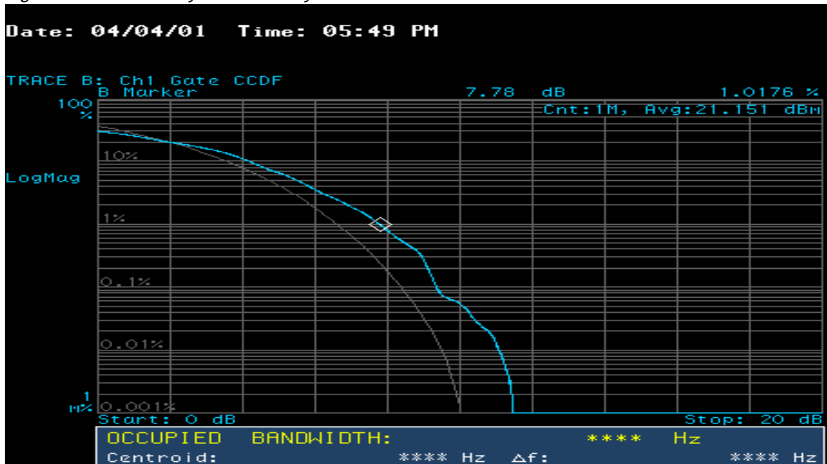
Figure 11.41 Time-Keyed Remote Synchronization Pilots Channel CCDF —Block B
