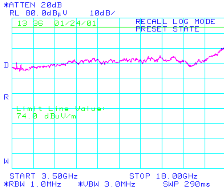
Figure 11.90 3.50GHz – 18GHz @1-m Antenna Height Emissions Scan, Vertical Polarization
