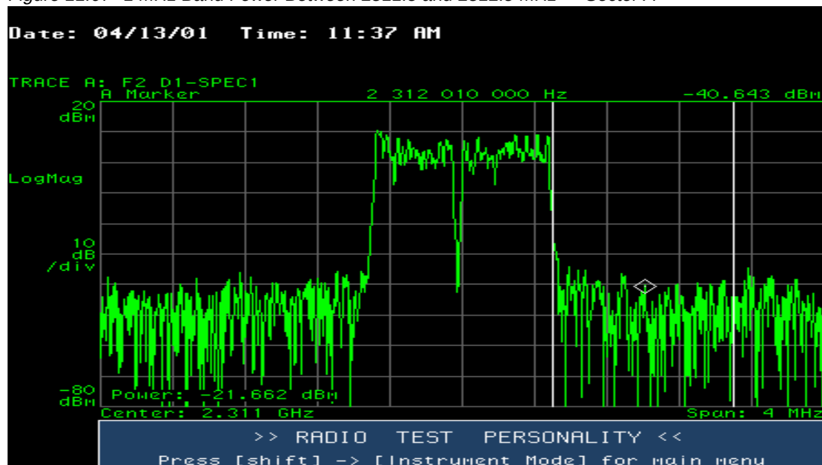
Figure 11.67 1 MHz Band Power Between 2311.5 and 2312.5 MHz — Sector A
