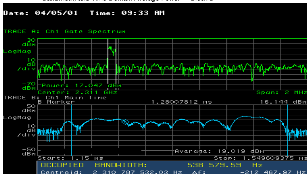
Figure 11.36 High Speed Data Control Channel Power vs. Frequency, 99% Occupied Bandwidth, and Time-Domain Average Power — Block B
