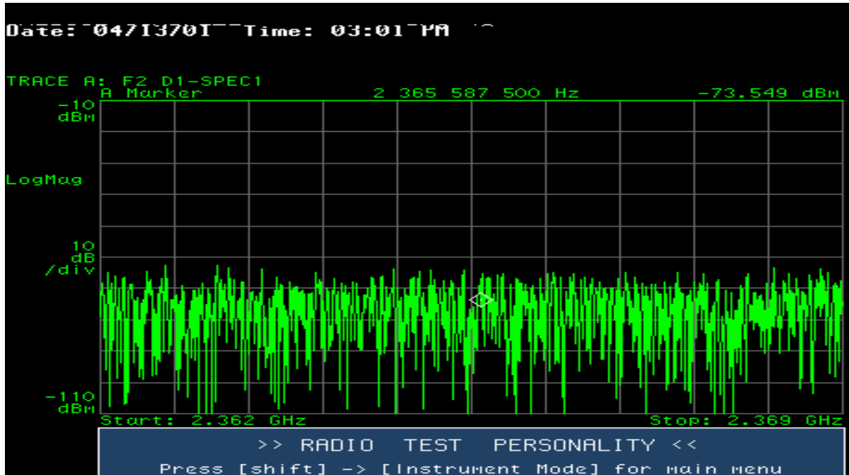
Figure 11.81 7 MHz Upper Guard Band Between 2362 MHz and 2369 MHz — Sector D
