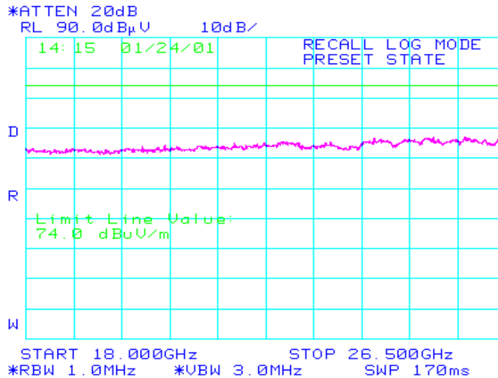
Figure 11.96 18.0 GHz – 26.5GHz @ 1-m Antenna Height Emissions Scan, Horizontal Polarization
