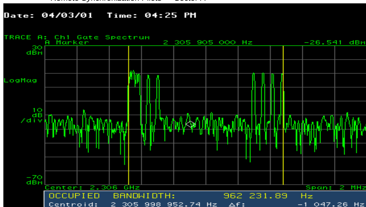
Figure 11.16 Base Station 99% Occupied Bandwidth While Transmitting Simulcast Remote Synchronization Pilots — Sector A
