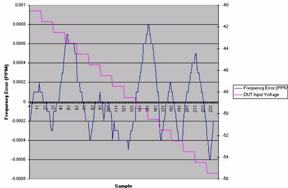
Figure 11.13 Frequency Stability vs. Input Voltage, GPS Locked Mode
