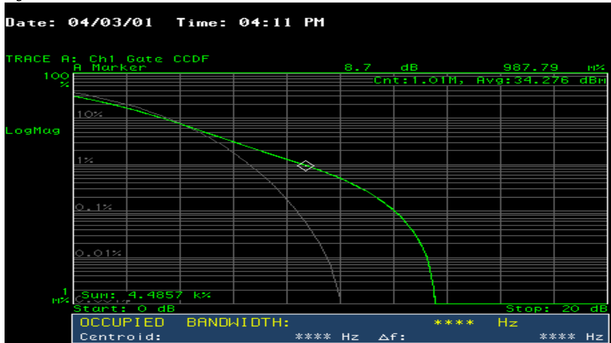
Figure 11.21 Voice Channel CCDF — Block A
