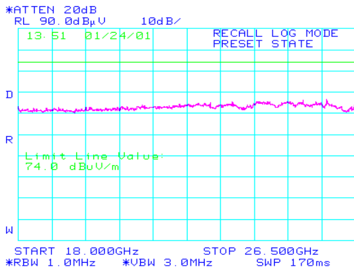
Figure 11.93 18.0 GHz – 26.5GHz @ 1.5-m Antenna Height Emissions Scan, Vertical Polarization
