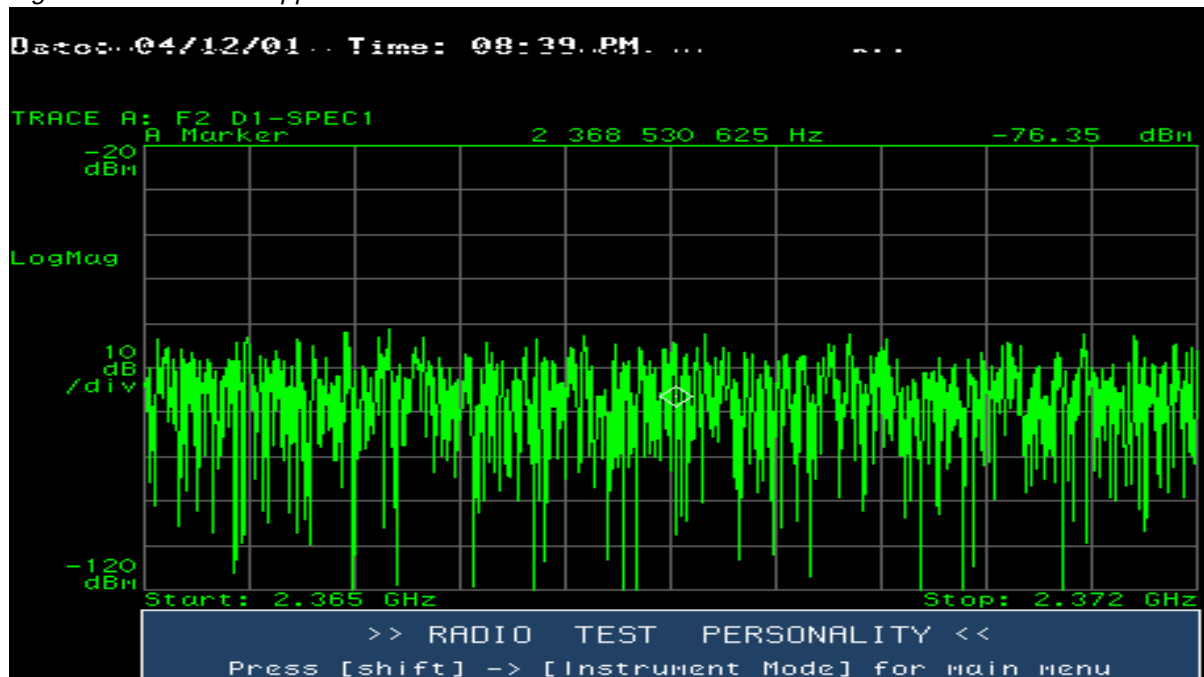
Figure 11.65 7 MHz Upper Guard Band Between 2365 MHz and 2372 MHz — Sector D
