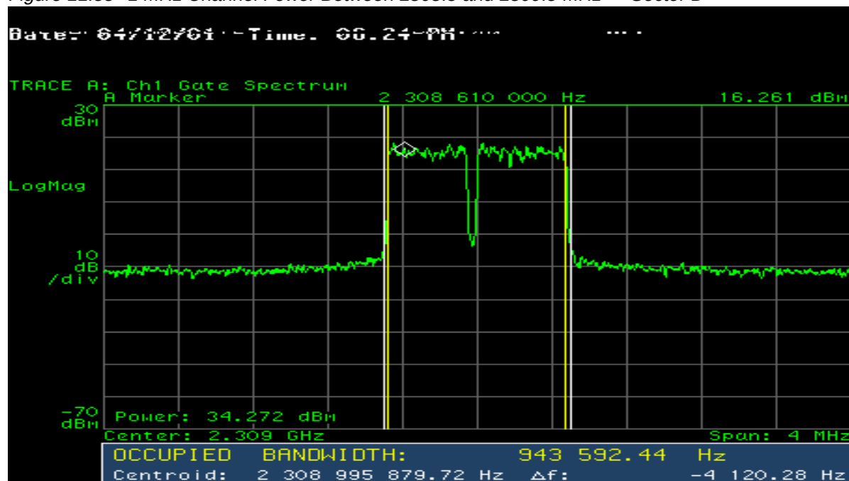
Figure 11.55 1 MHz Channel Power Between 2308.5 and 2309.5 MHz — Sector D
