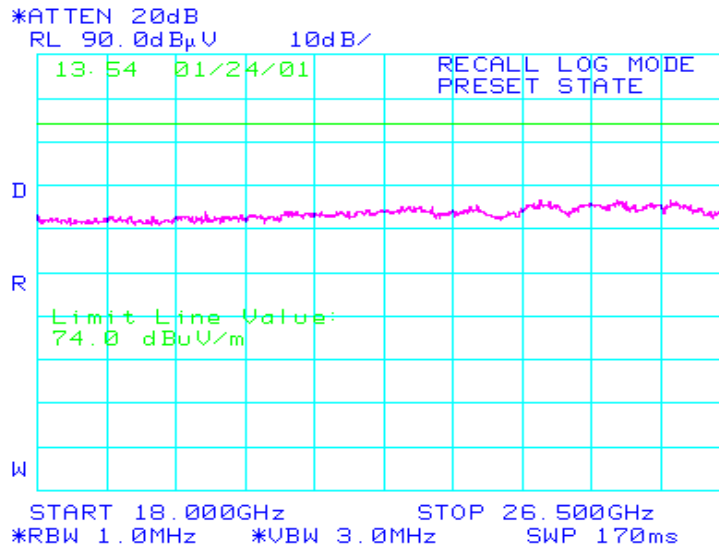
Figure 11.94 18.0 GHz – 26.5GHz @ 1-m Antenna Height Emissions Scan, Vertical Polarization
