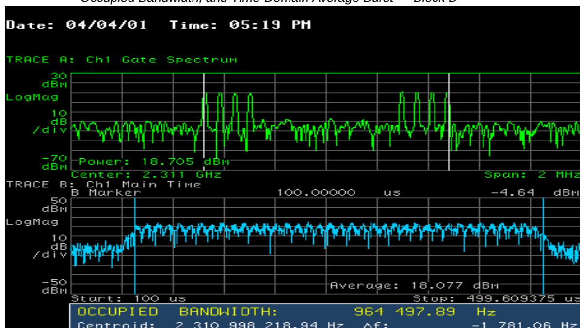
Figure 11.42 Simulcast Remote Synchronization Pilots Power vs. Frequency, 99.0% Occupied Bandwidth, and Time-Domain Average Burst — Block B
