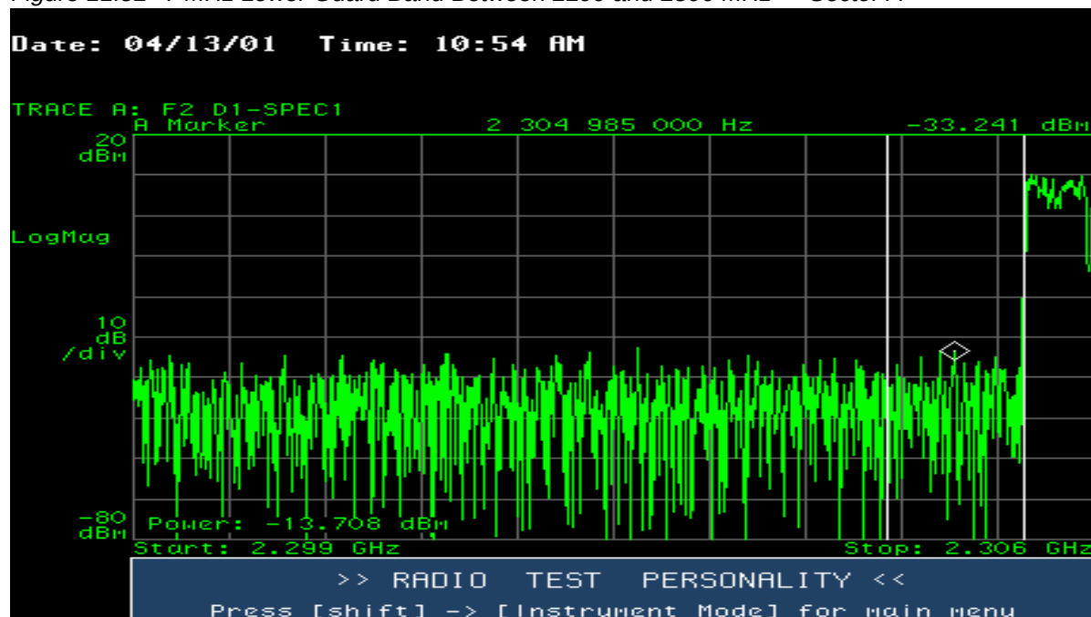
Figure 11.52 7 MHz Lower Guard Band Between 2299 and 2306 MHz — Sector A
