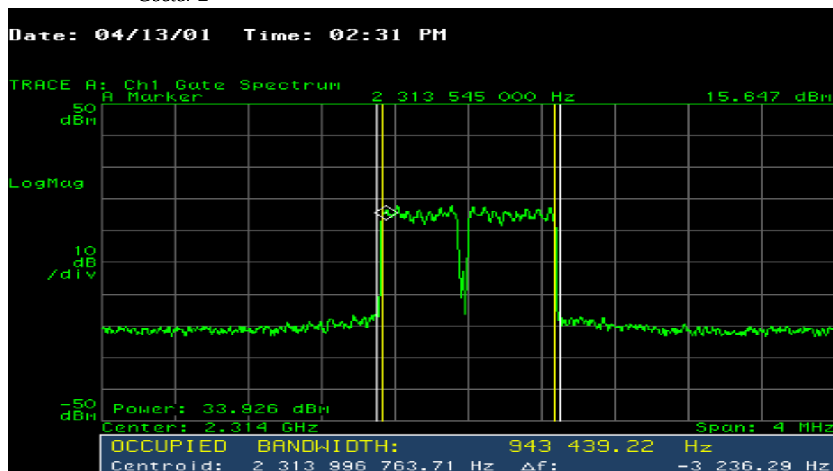
Figure 11.72 1 MHz Channel Power Between 2313.5 MHz and 2314.5 MHz — Sector D
