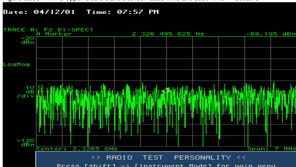
Figure 11.59 7 MHz Upper Guard Band Between 2323 MHz and 2330 MHz — Sector D
