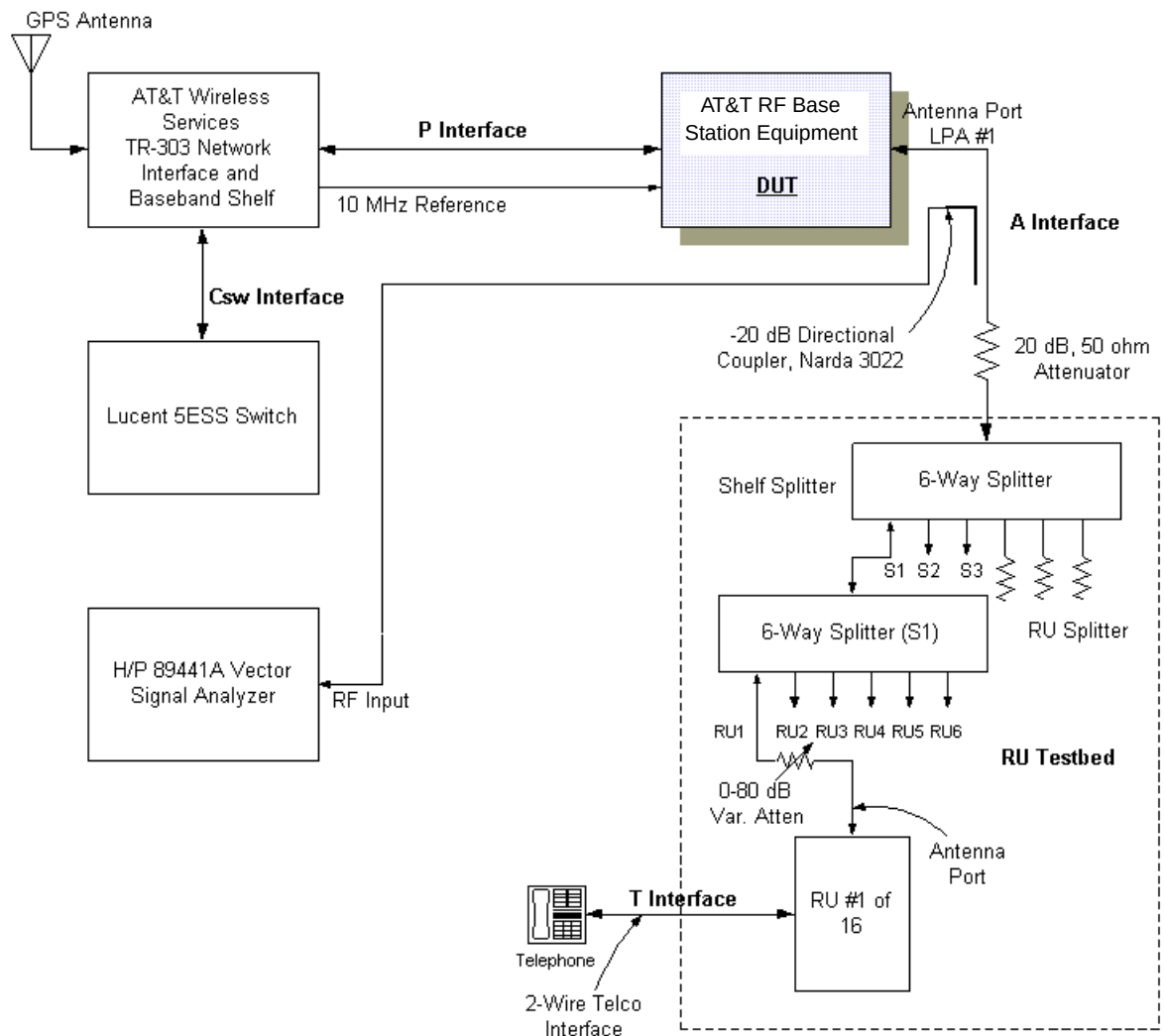
Figure 11.8 Spectral Purity Test Configuration
