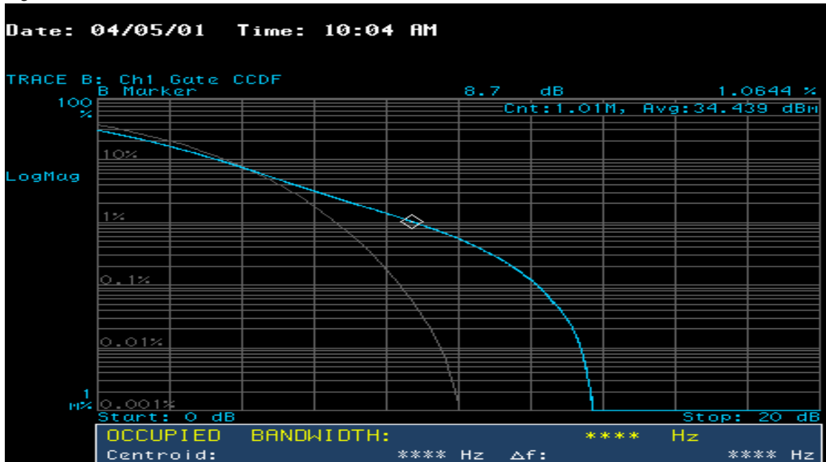
Figure 11.33 Voice Channel CCDF — Block B
