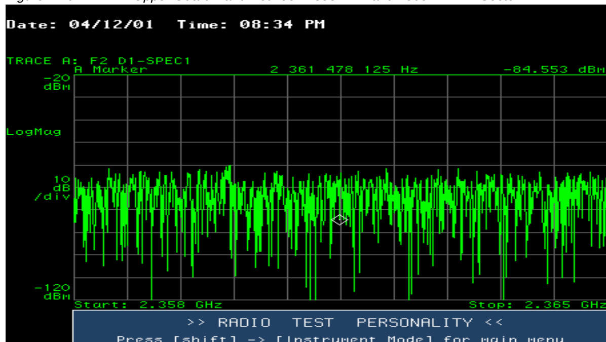
Figure 11.64 7 MHz Upper Guard Band Between 2358 MHz and 2365 MHz — Sector D
