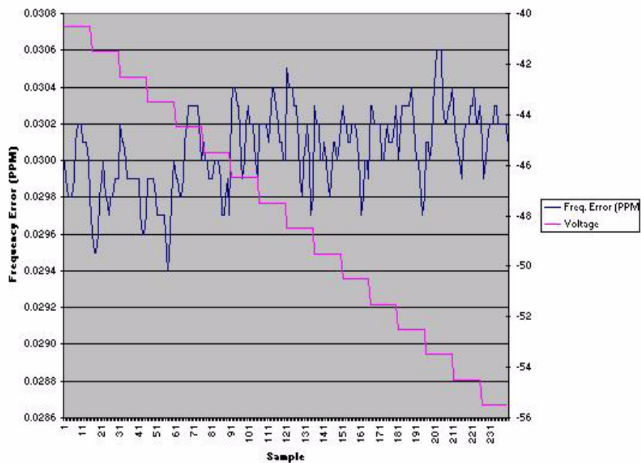
Figure 11.15 Frequency Stability vs. Input Voltage, GPS Free-Run Mode
