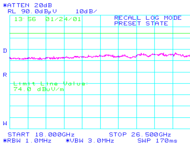
Figure 11.95 18.0 GHz – 26.5GHz @ 2-m Antenna Height Emissions Scan, Vertical Polarization
