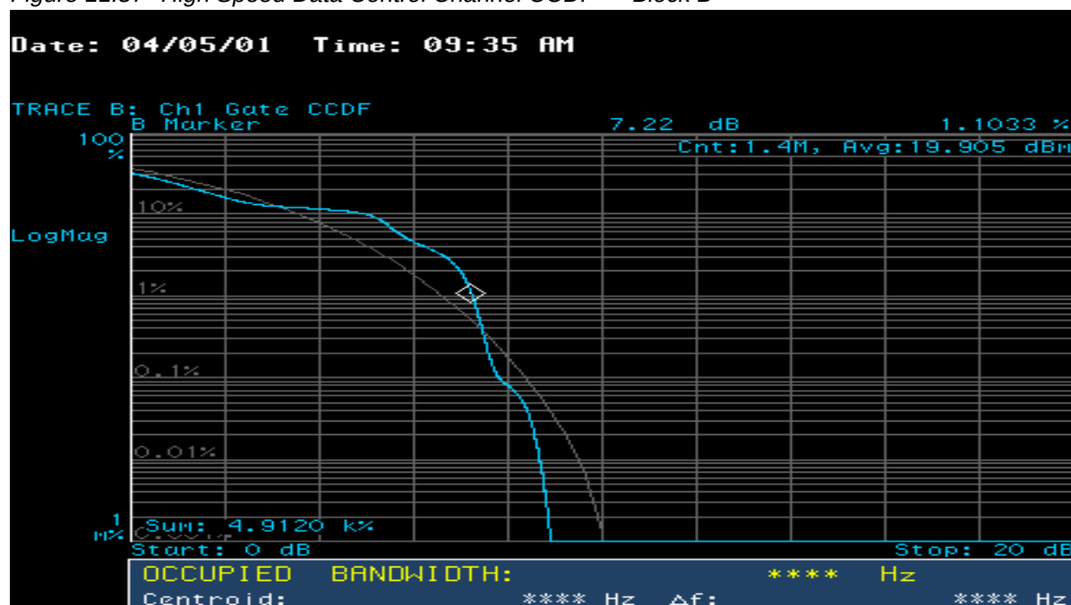
Figure 11.37 High Speed Data Control Channel CCDF — Block B
