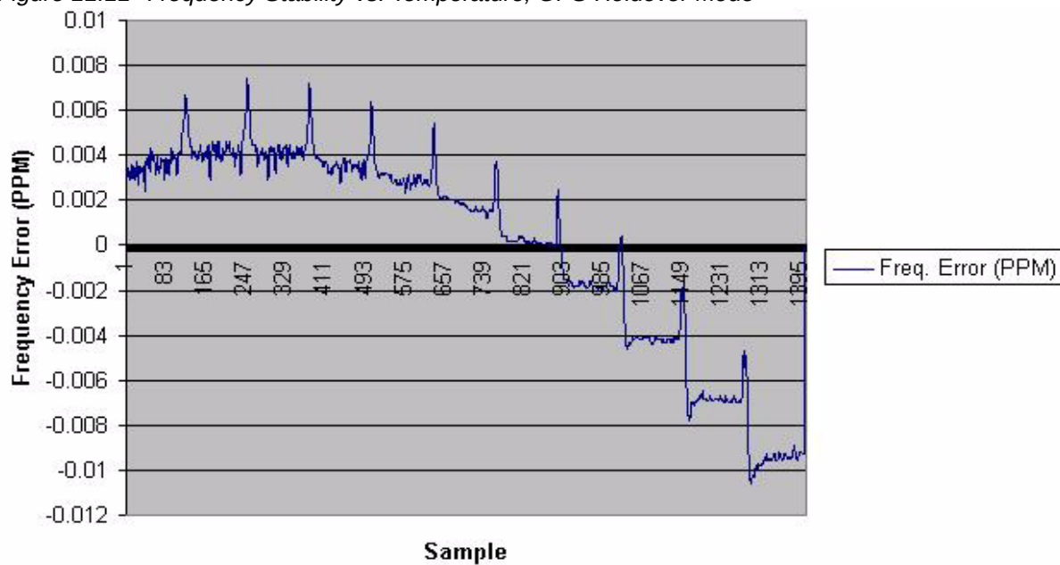
Figure 11.11 Frequency Stability vs. Temperature, GPS Holdover Mode
