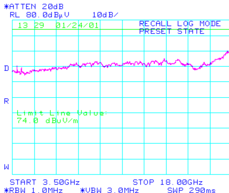
Figure 11.89 3.50GHz – 18GHz @ 2-m Antenna Height Emissions Scan, Horizontal Polarization
