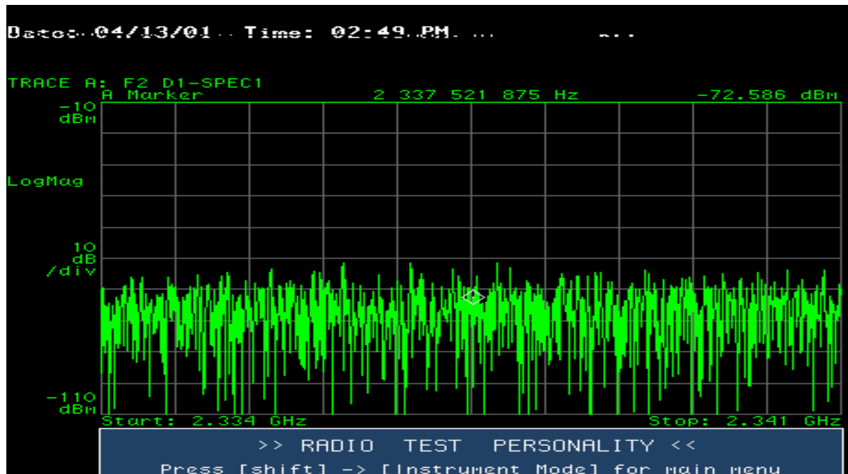
Figure 11.77 7 MHz Upper Guard Band Between 2334 MHz and 2341 MHz — Sector D
