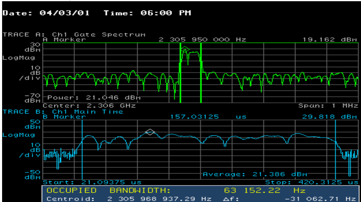
Figure 11.26 NAC Channel Power vs. Frequency, 99% Occupied BW, and Time-Domain Average Power — Block A
