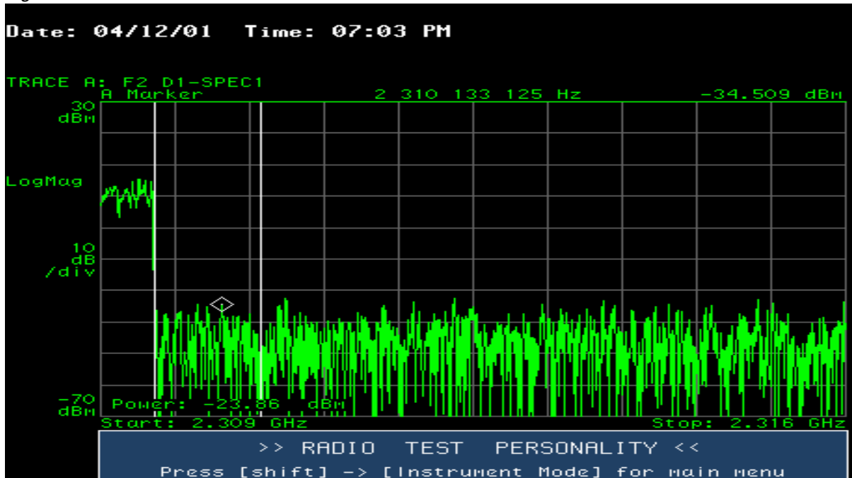
Figure 11.57 1 MHz Band Power Between 2309.5 and 2310.5 MHz — Sector D
