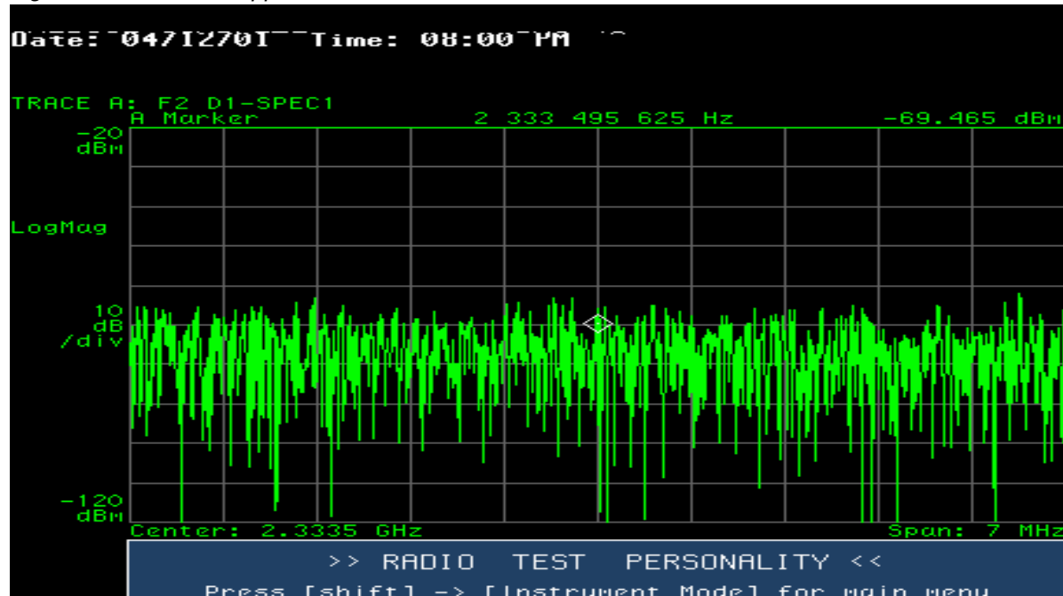
Figure 11.60 7 MHz Upper Guard Band Between 2330 MHz and 2337 MHz — Sector D
