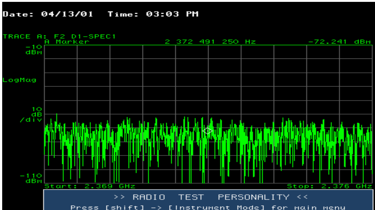
Figure 11.82 7 MHz Upper Guard Band Between 2369 MHz and 2376 MHz — Sector D
