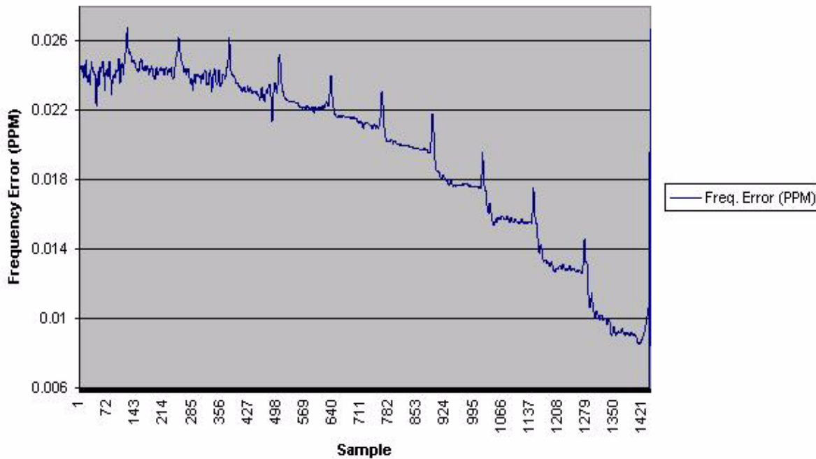
Figure 11.12 Frequency Stability vs. Temperature, GPS Free-Run Mode
