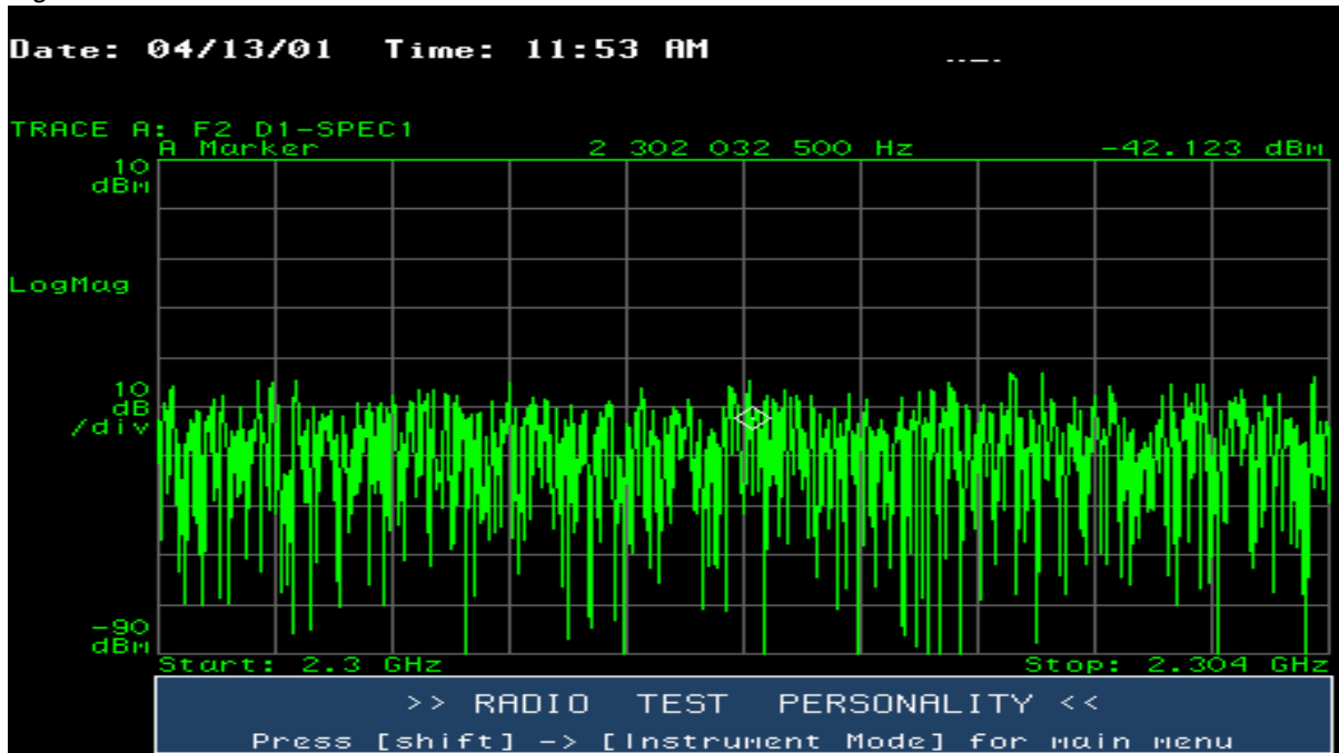
Figure 11.69 7 MHz Lower Guard Band Between 2300 MHz and 2304 MHz — Sector A
