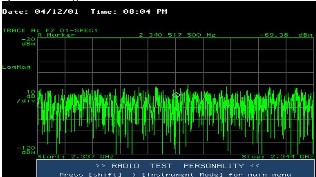
Figure 11.61 7 MHz Upper Guard Band Between 2337 MHz and 2344 MHz — Sector D
