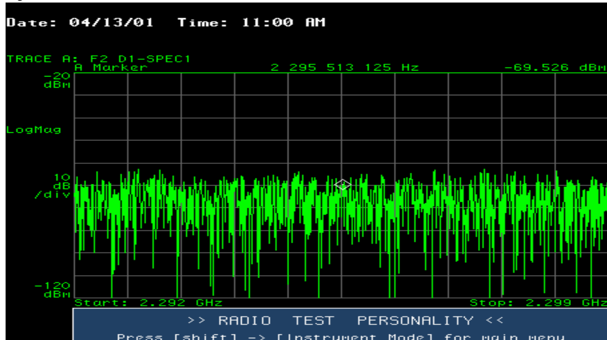
Figure 11.53 7 MHz Lower Guard Band Between 2292 MHz and 2299 MHz — Sector A
