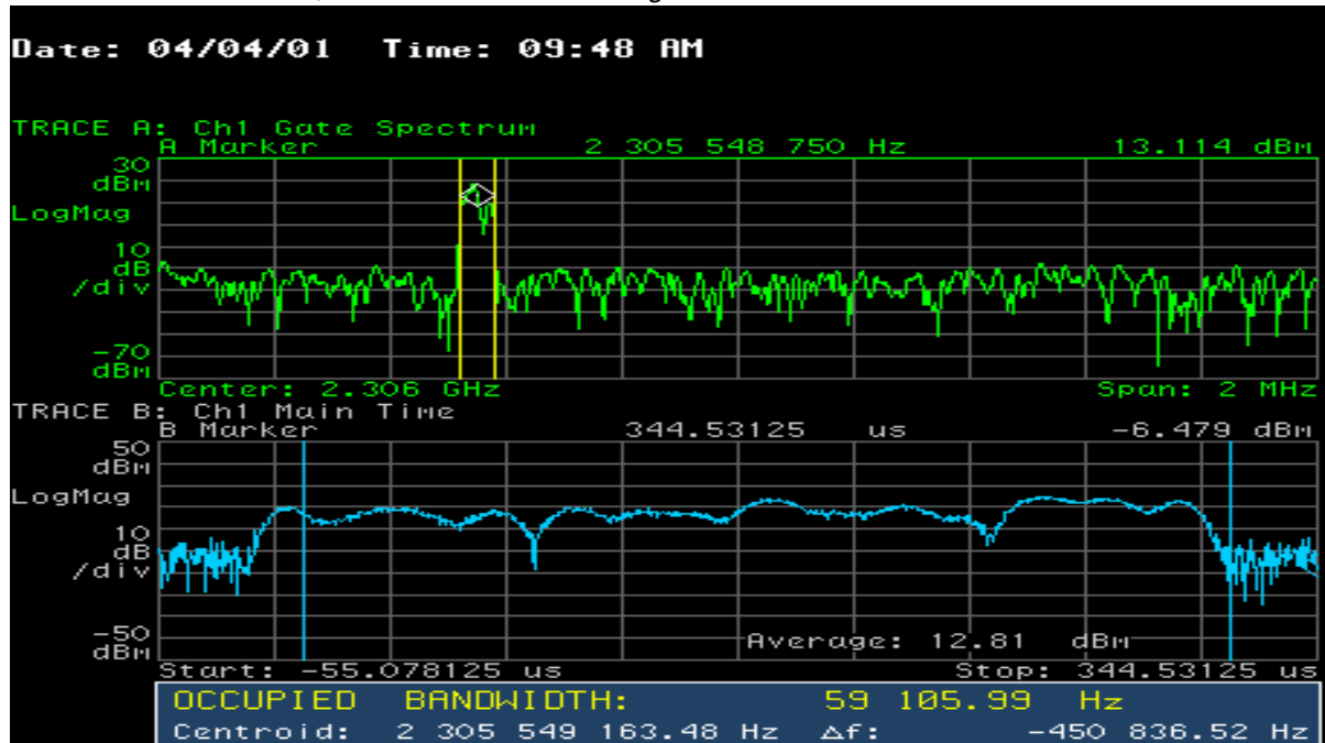
Figure 11.24 High Speed Data Control Channel Power vs. Frequency, 99% Occupied Bandwidth, and Time-Domain Average Power — Block A
