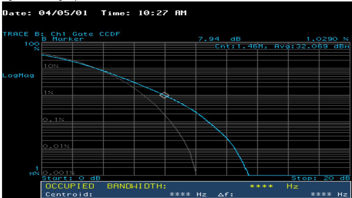
Figure 11.35 High-Speed Data Channel CCDF — Block B
