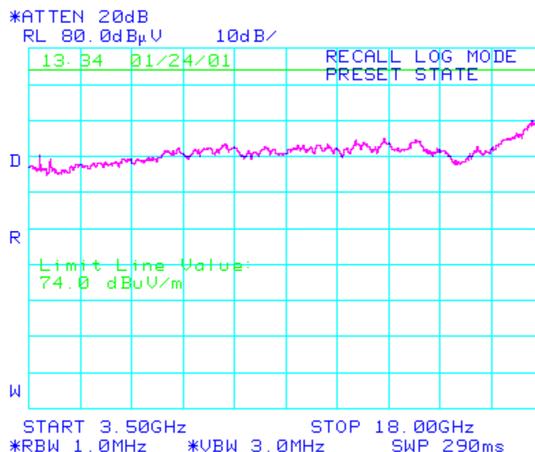
Figure 11.91 3.50GHz – 18GHz @1.5-m Antenna Height Emissions Scan, Vertical Polarization
