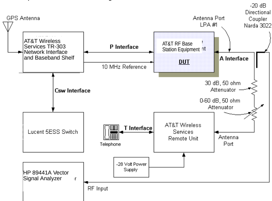
Figure 11.4 Occupied Bandwidth Test Configuration
