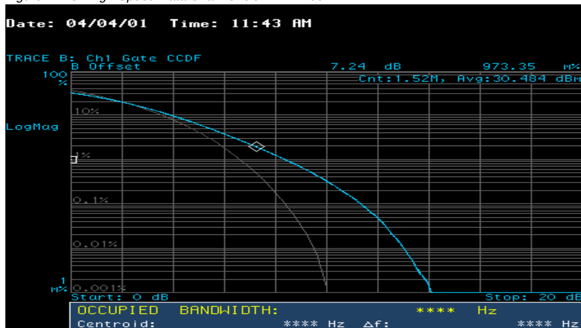
Figure 11.23 High-Speed Data Channel CCDF — Block A
