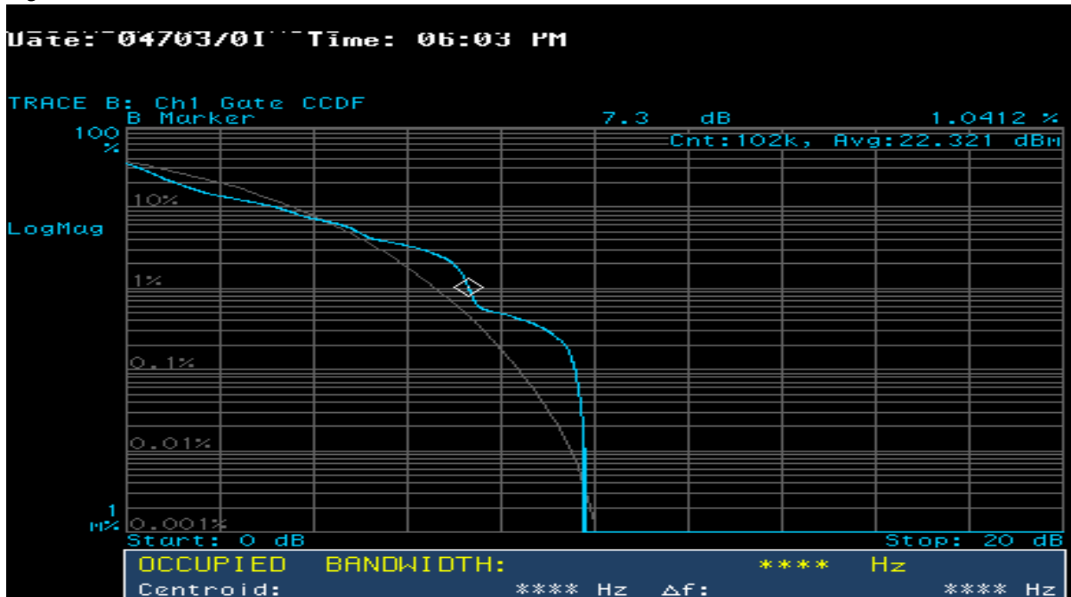
Figure 11.27 NAC Channel CCDF — Block A
