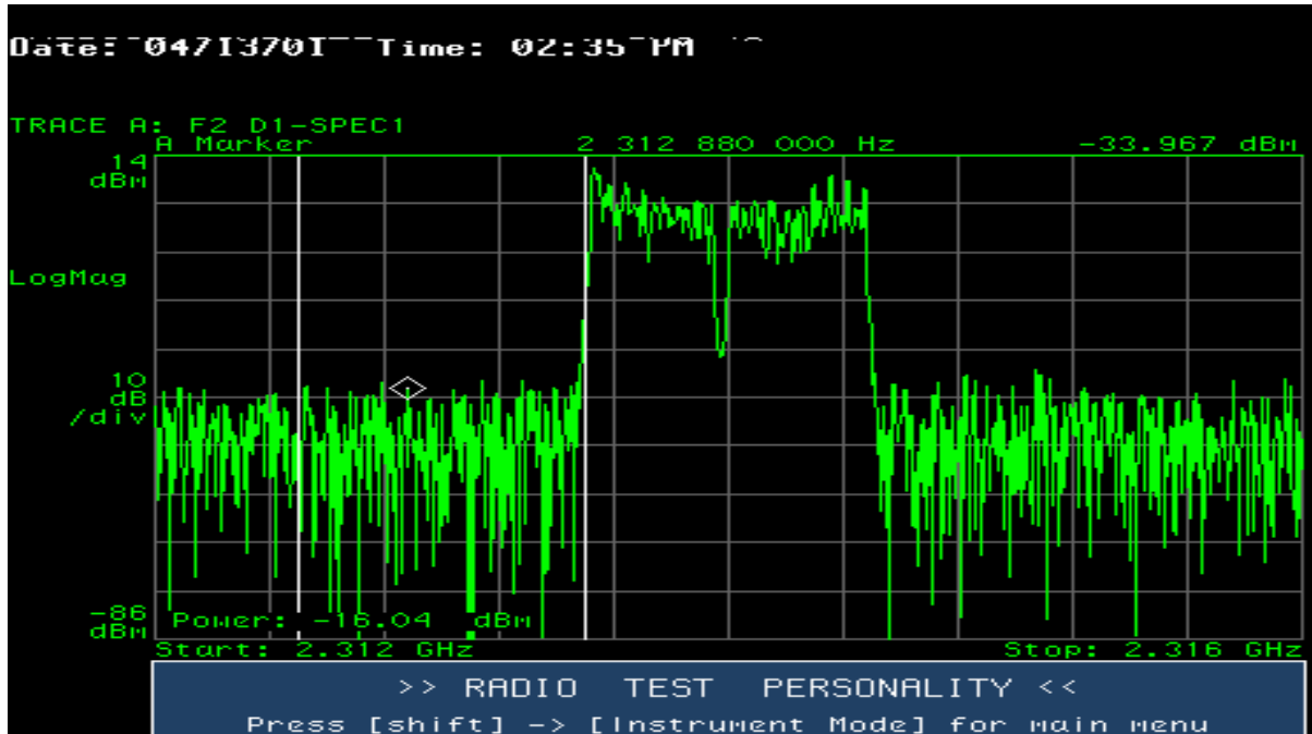
Figure 11.73 1 MHz Channel Power Between 2312.5 MHz and 2313.5 MHz — Sector D
