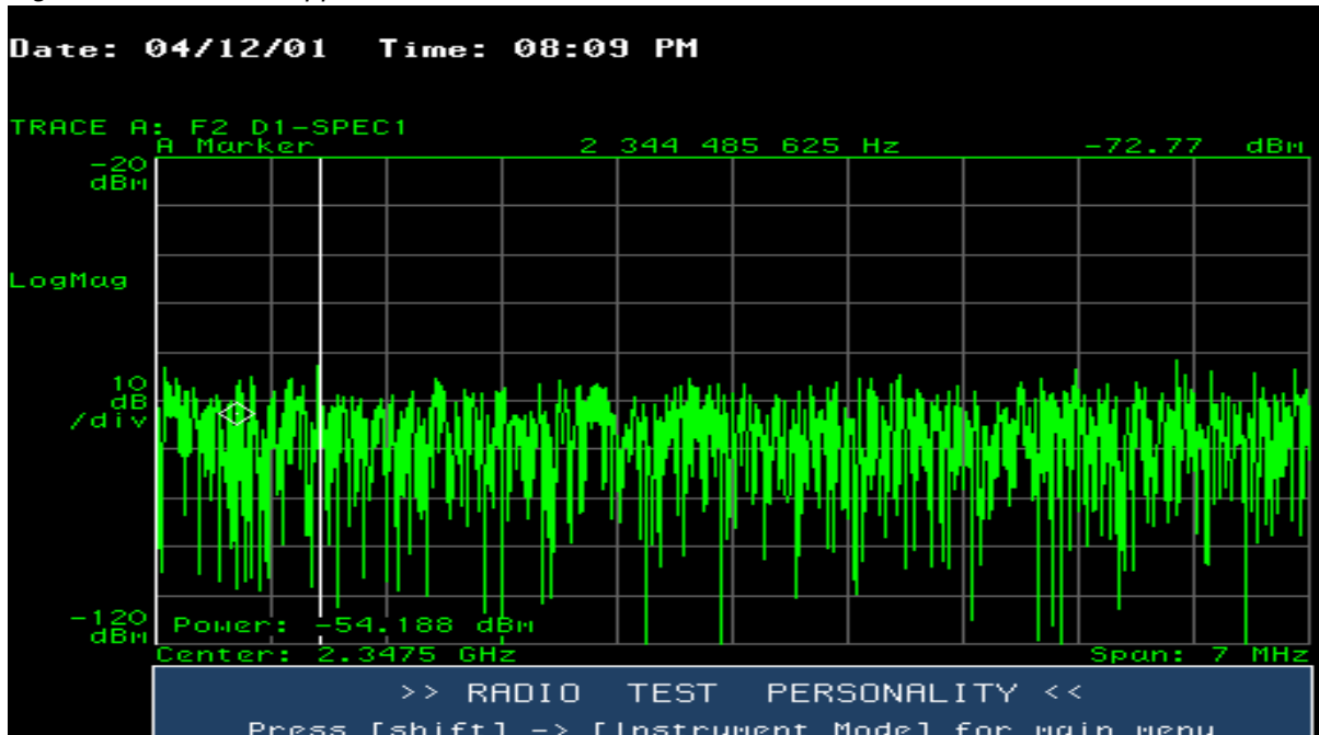
Figure 11.62 7 MHz Upper Guard Band Between 2344 MHz and 2351 MHz — Sector D
