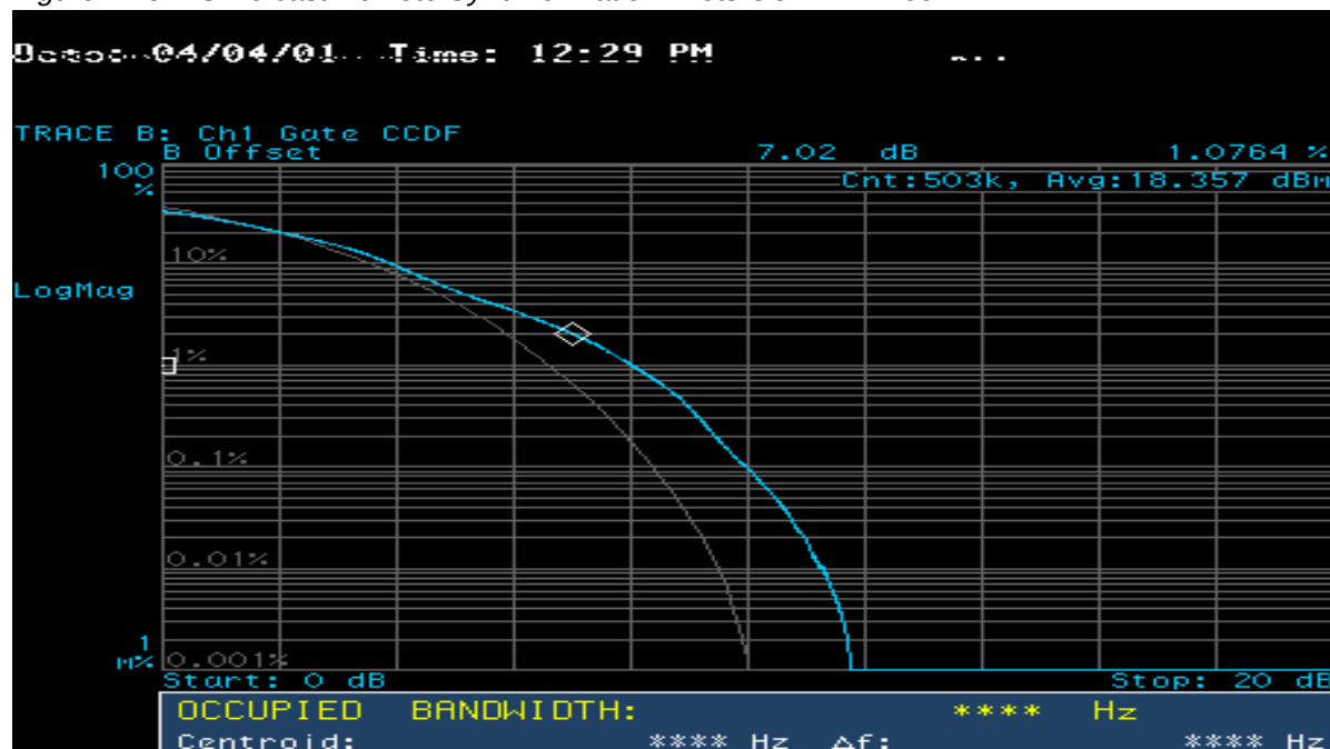
Figure 11.31 Simulcast Remote Synchronization Pilots CCDF — Block A
