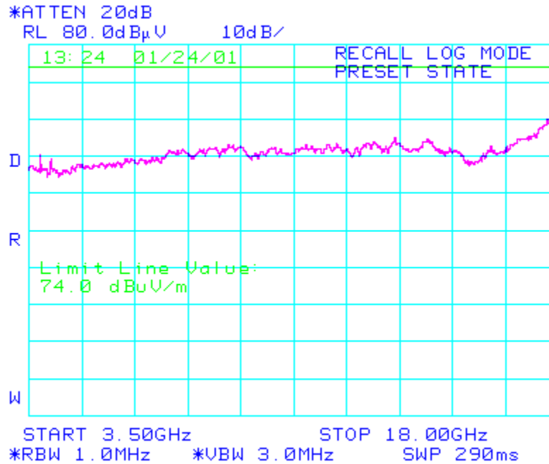
Figure 11.88 3.5 GHz – 18 GHz @ 1.5-m Antenna Height Emissions Scan, Horizontal Polarization
