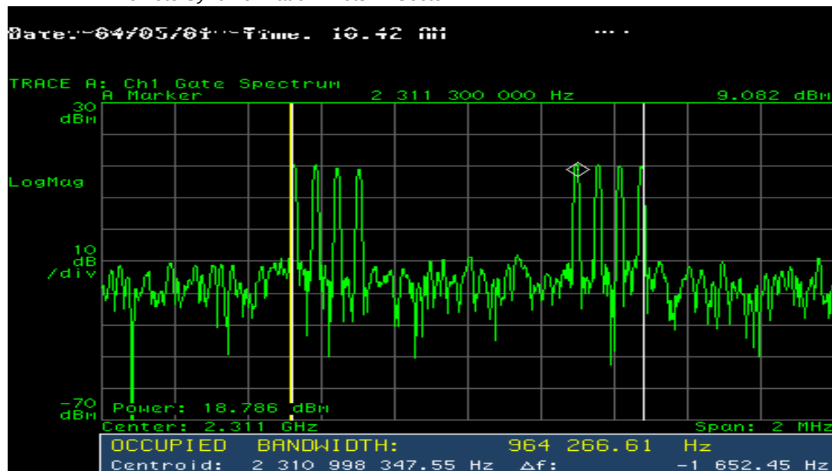
Figure 11.18 Base Station 99% Occupied Bandwidth While Transmitting Simulcast Remote Synchronization Pilots — Sector A
