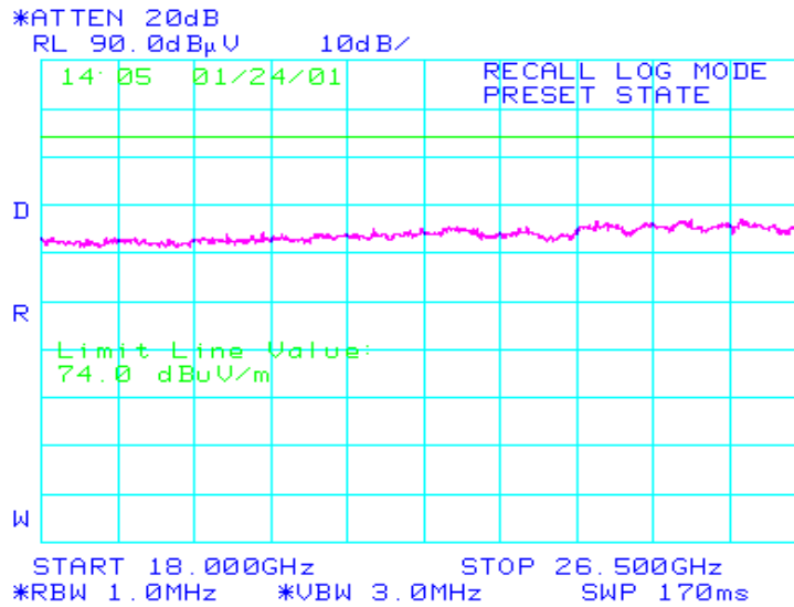
Figure 11.98 18.0 GHz – 26.5GHz @ 2-m Antenna Height Emissions Scan, Horizontal Polarization
