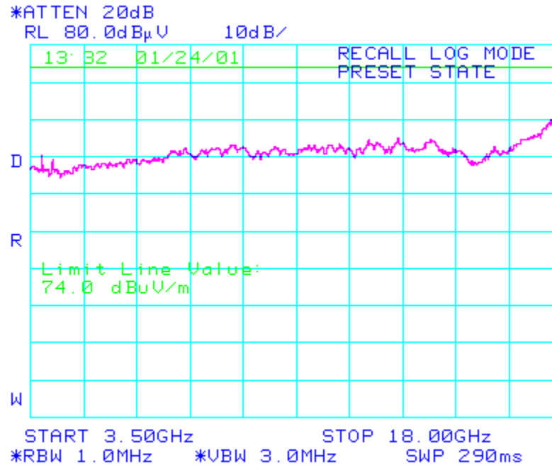
Figure 11.92 3.50GHz – 18GHz @ 2-m Antenna Height Emissions Scan, Vertical Polarization
