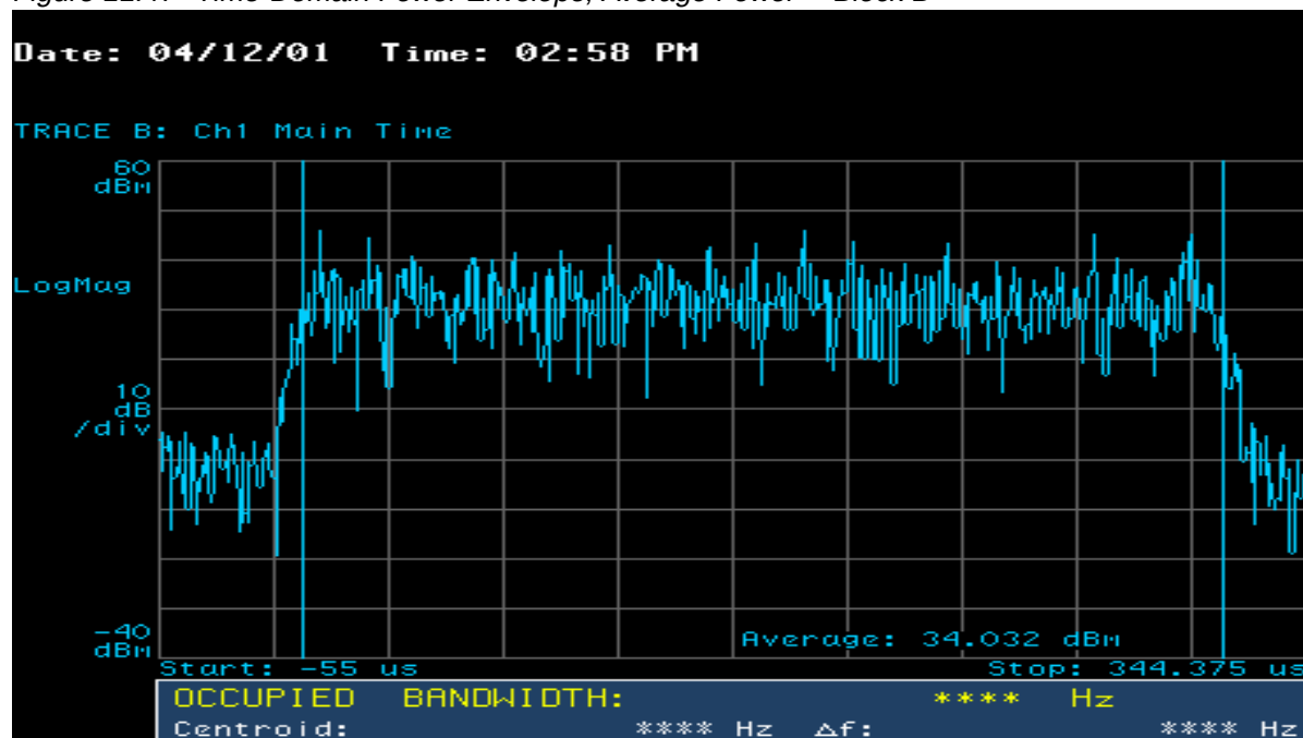
Figure 11.47 Time-Domain Power Envelope, Average Power— Block B
