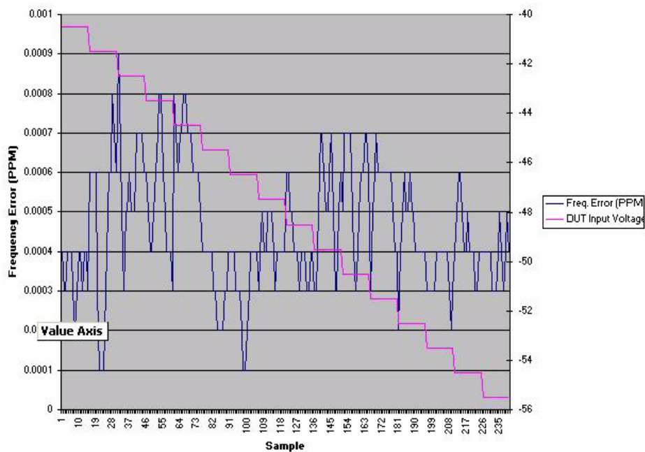
Figure 11.14 Frequency Stability vs. Input Voltage, GPS Holdover Mode
