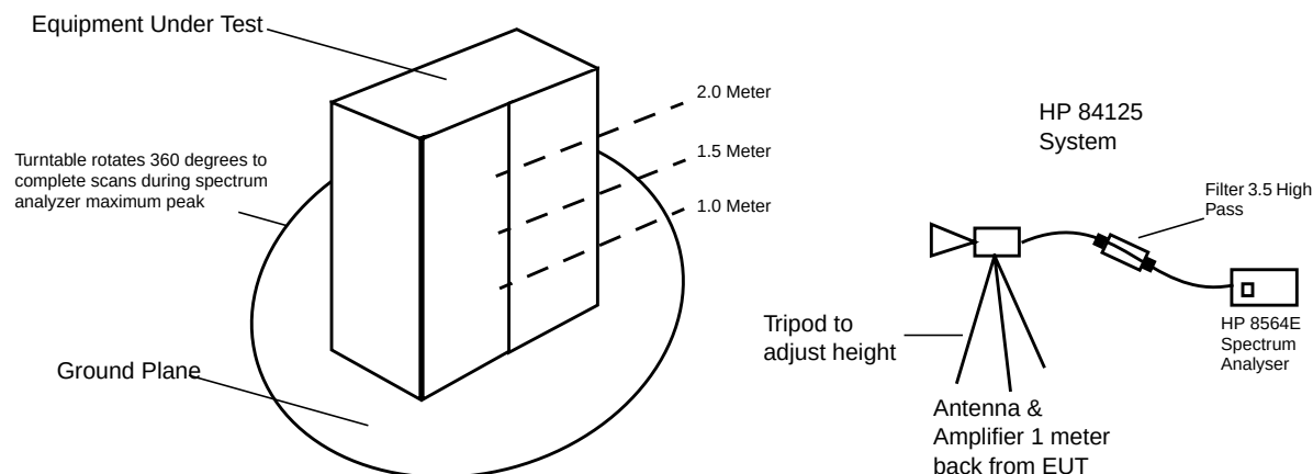
Figure 11.84 Radiated Emissions Testing
