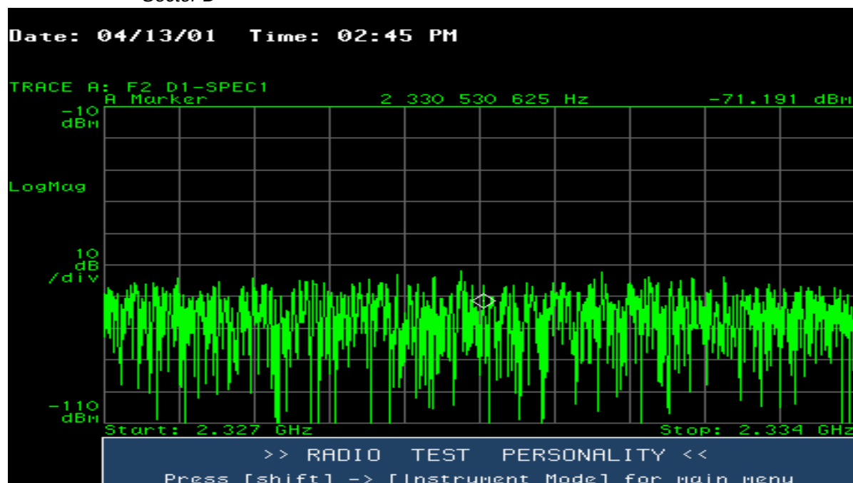
Figure 11.76 7 MHz Upper Guard Band Between 2327 MHz and 2334 MHz — Sector D
