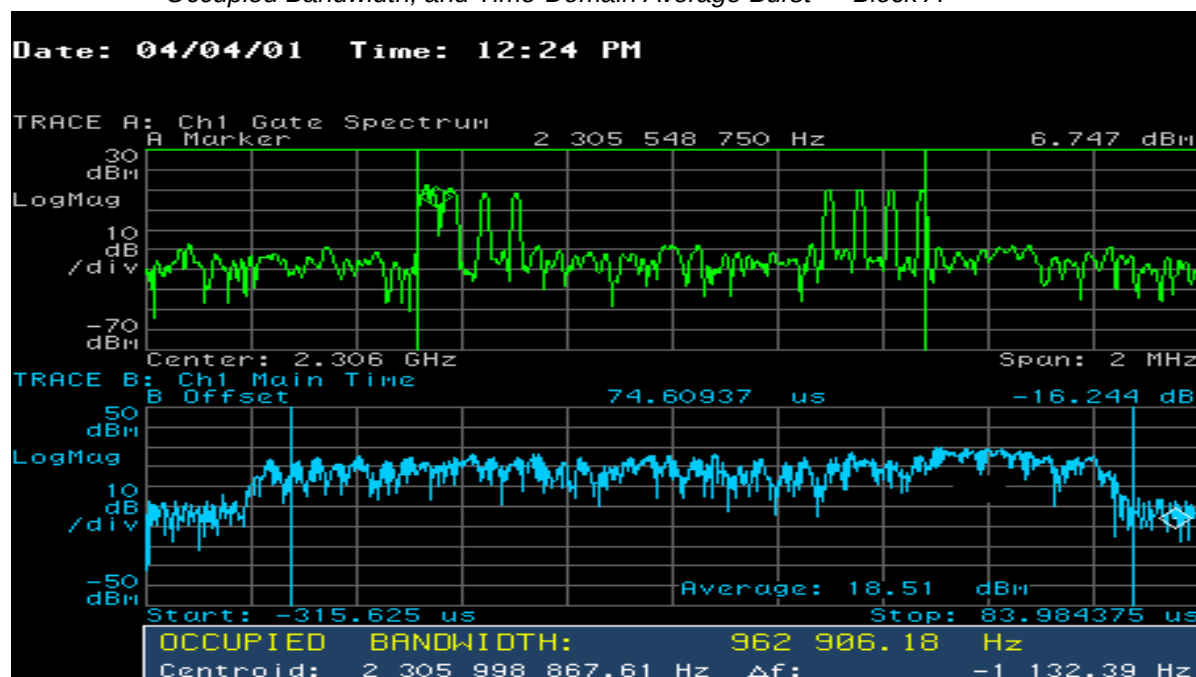
Figure 11.30 Simulcast Remote Synchronization Pilots Power vs. Frequency, 99.0% Occupied Bandwidth, and Time-Domain Average Burst — Block A
