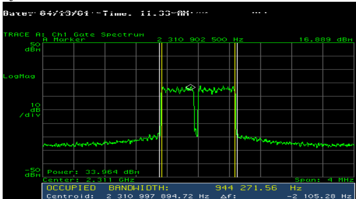
Figure 11.66 1 MHz Band-Power Between 2310.5 and 2311.5 MHz — Sector A
