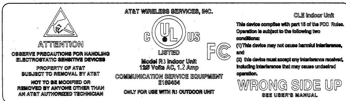
Figure 5.1 FCC ID Label for the R3 Indoor Unit
