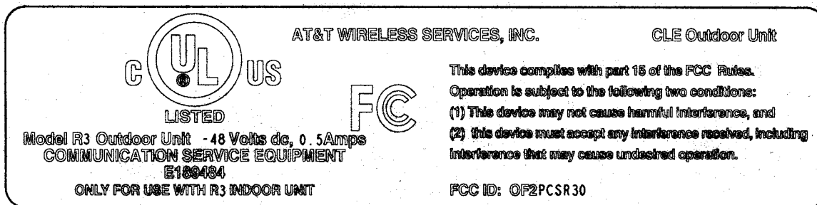
Figure 5.2 FCC ID Label for the R3 Outdoor Unit
