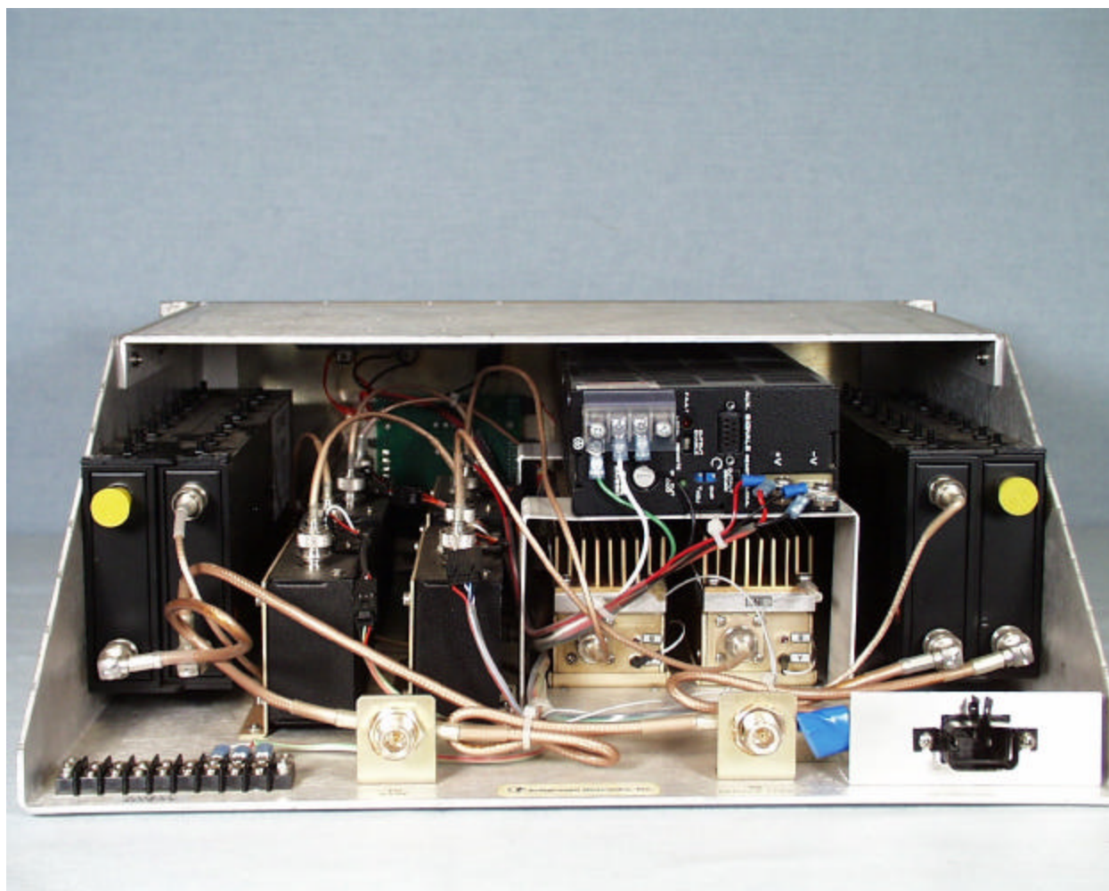
Back View of the Celwave BDA
