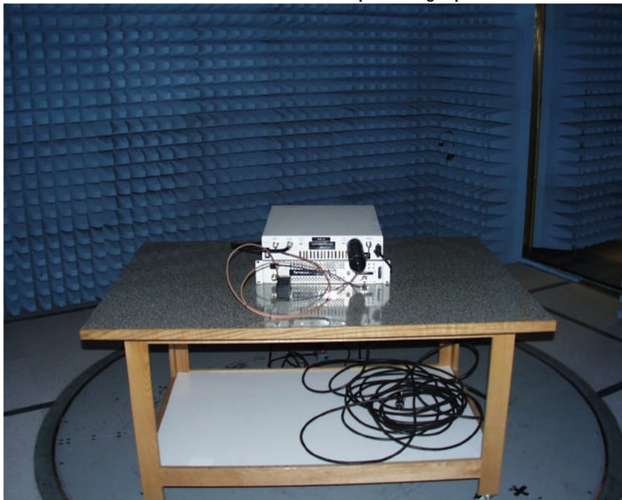
Front view of the test set-up
