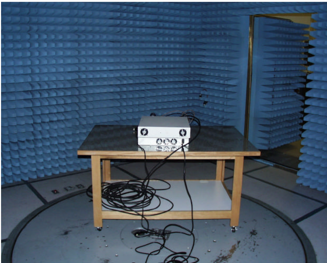
Back view of the test set-up
