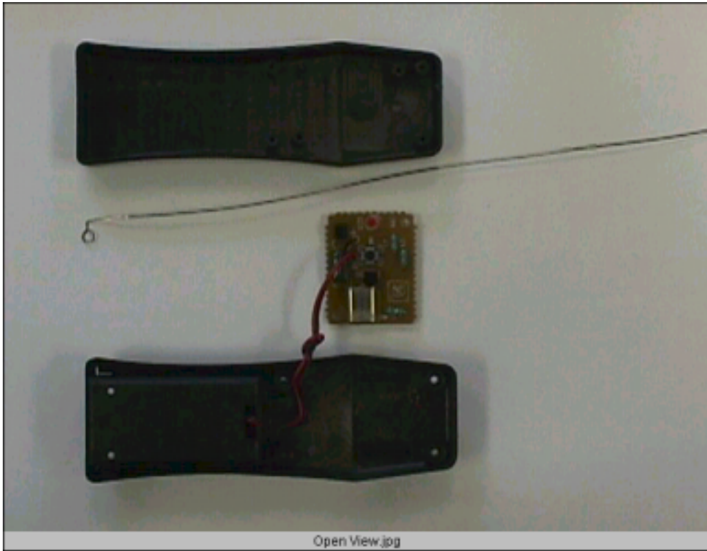
Expedite International - Transmitter, open showing Antenna, Transmitter PCB and outer shells.
