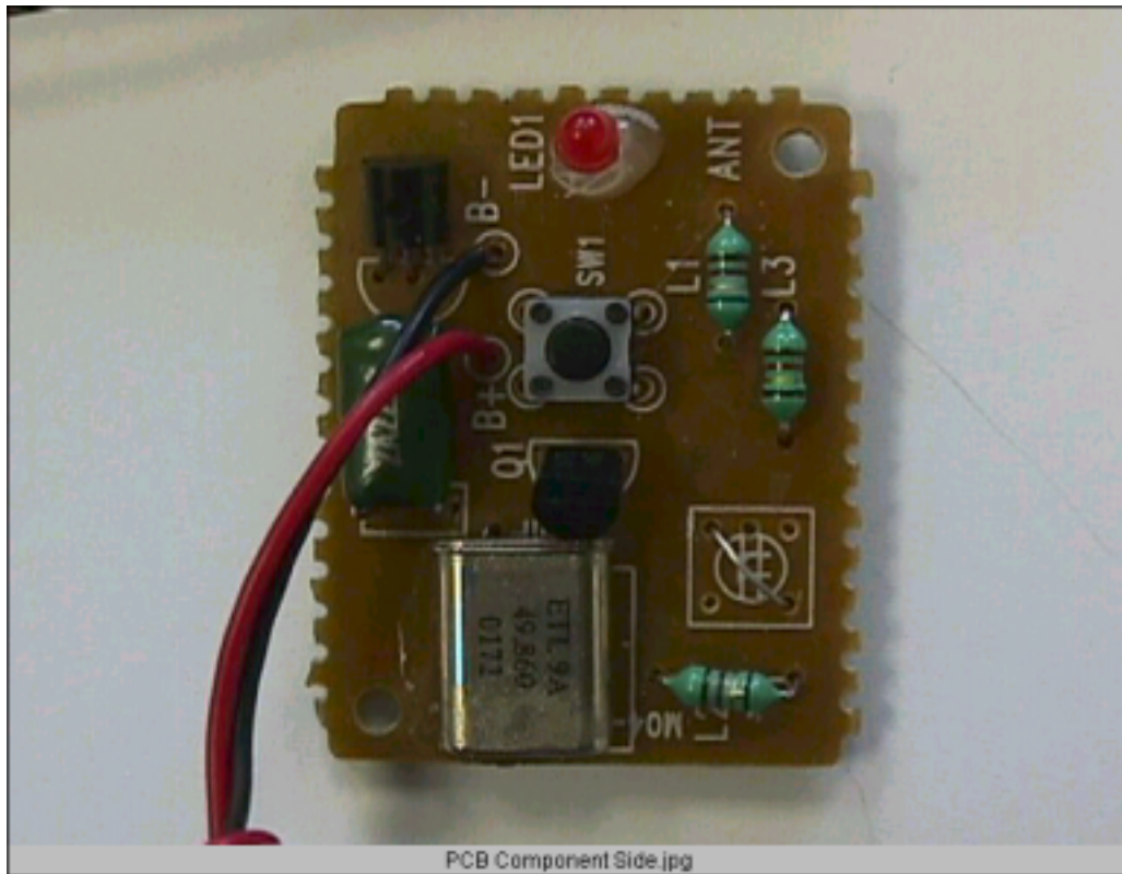
Expedite International - Transmitter PCB, Component Side
