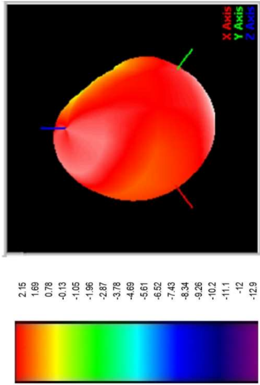
Typical H-Plane Antenna Pattern
