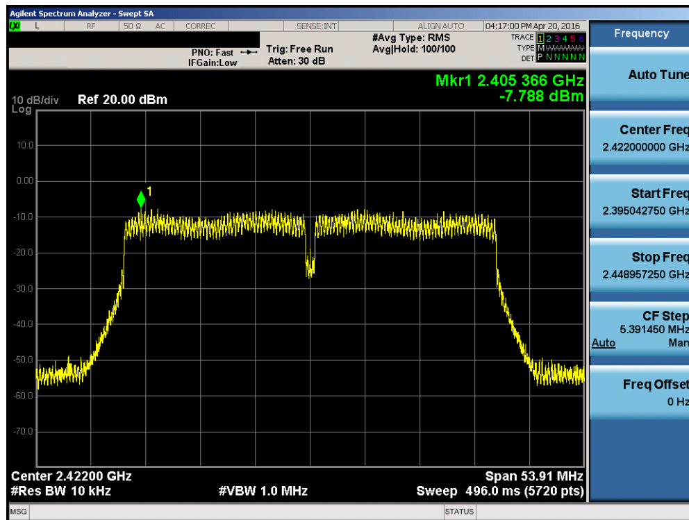
Plot 7-22. Power Spectral Density Plot (802.11n (40MHz BW) – Ch. 1 + 5)
