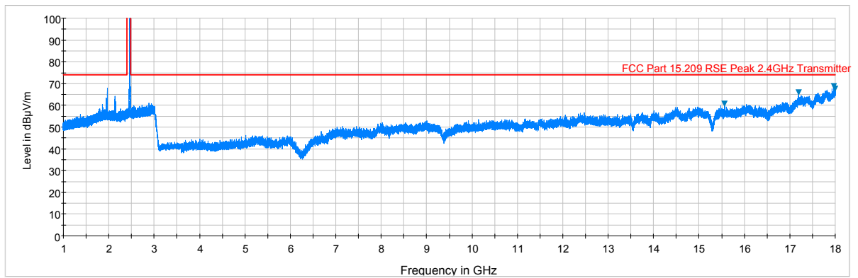
Plot 7-47. Radiated Spurious Plot above 1GHz (802.11b – Ch. 11, Ant. Pol. H)
