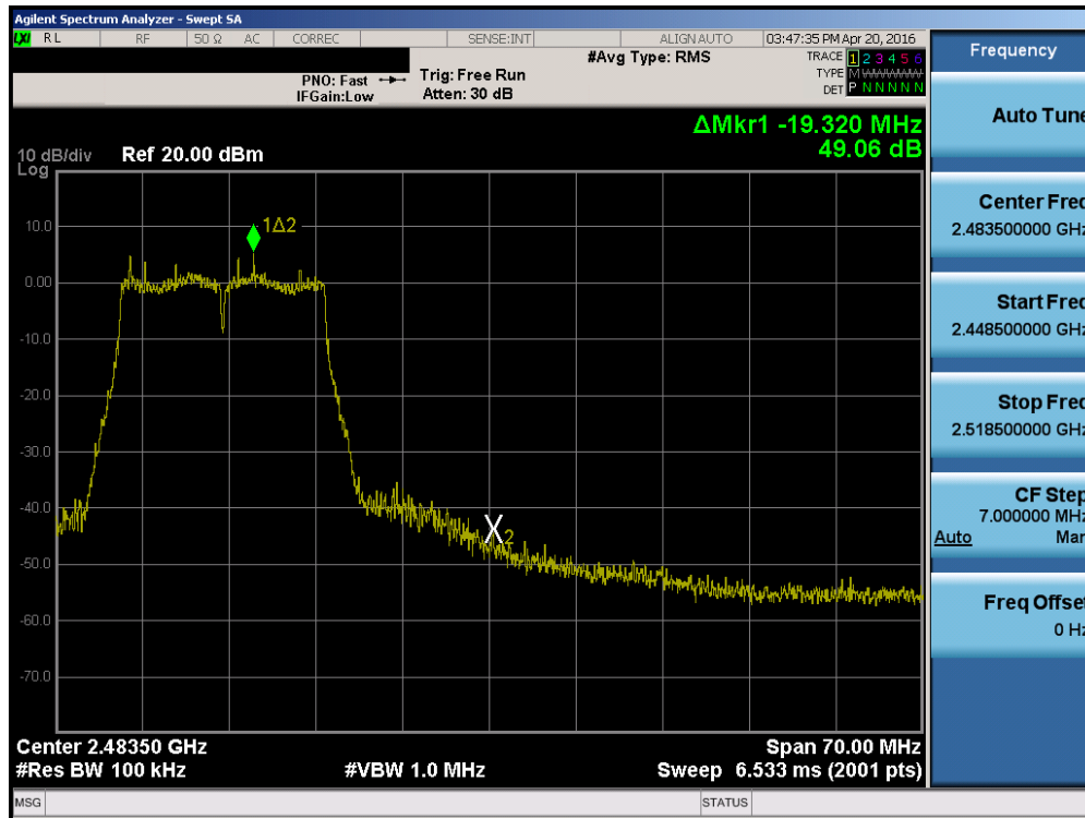
Plot 7-29. Band Edge Plot (802.11g – Ch. 11)
