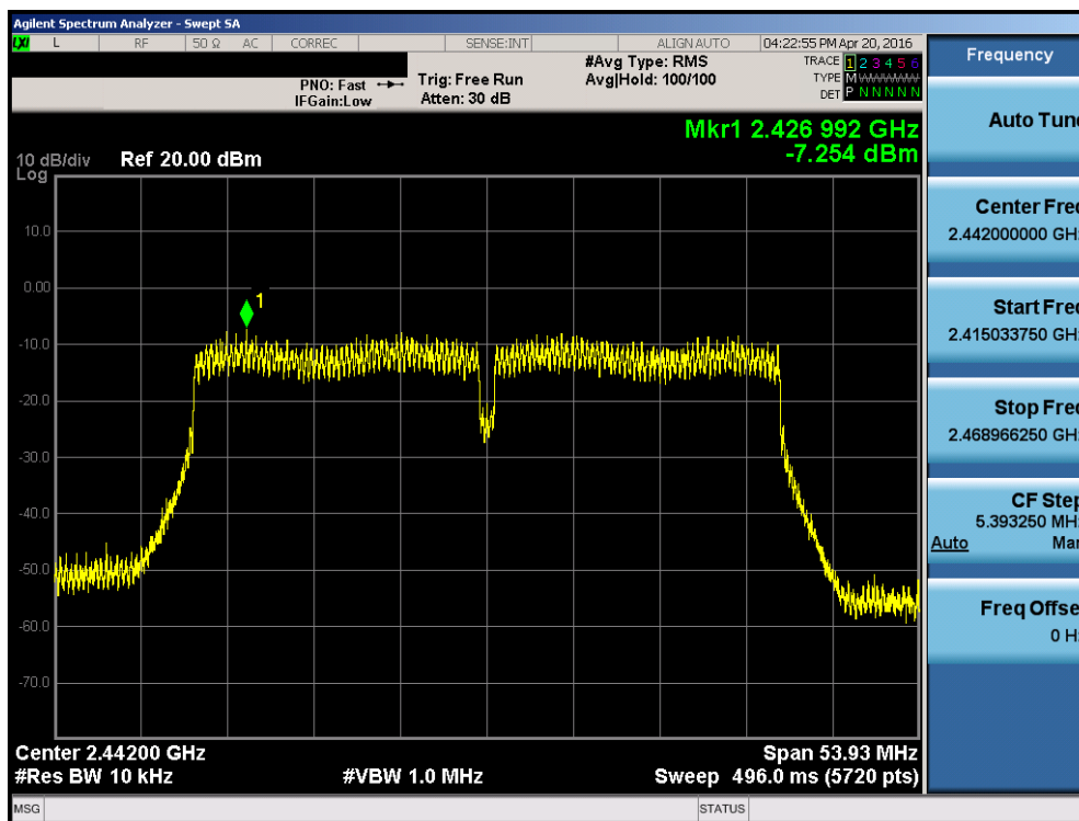
Plot 7-23. Power Spectral Density Plot (802.11n (40MHz BW) – Ch. 5 + 9)
