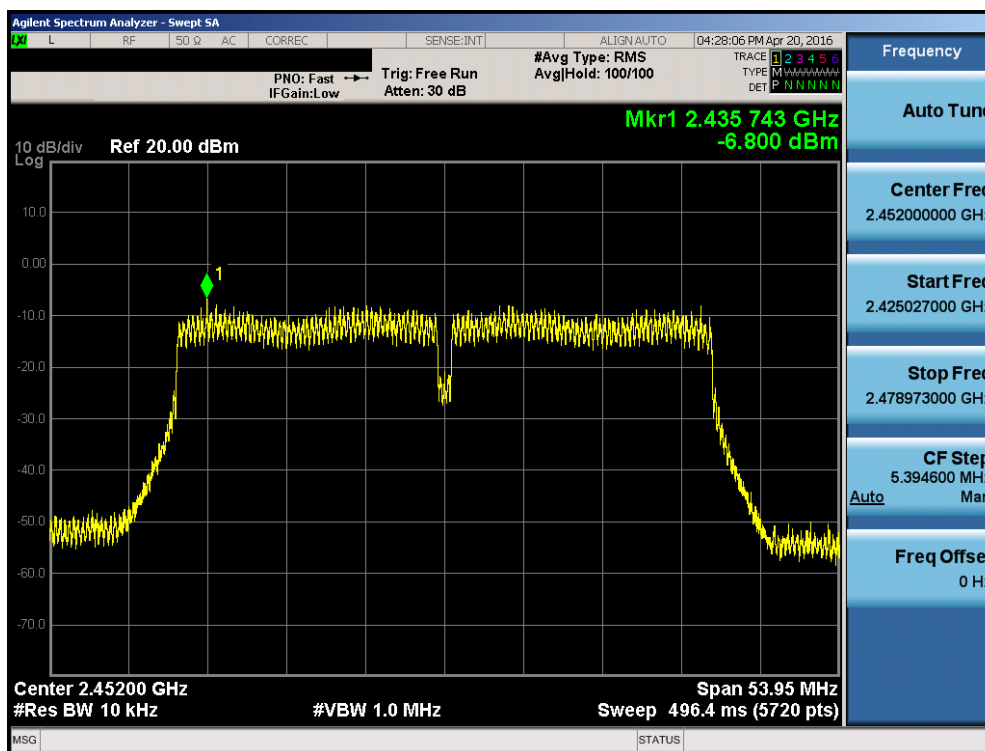
Plot 7-24. Power Spectral Density Plot (802.11n (40MHz BW) – Ch. 7 + 11)
