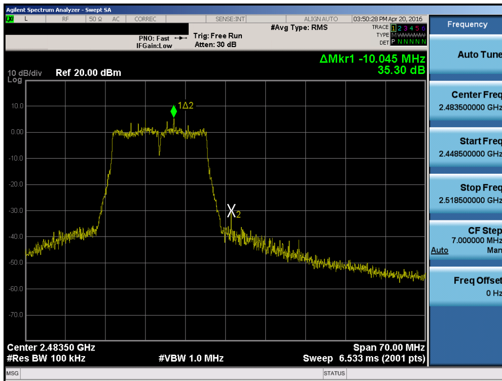
Plot 7-30. Band Edge Plot (802.11g – Ch. 13)
