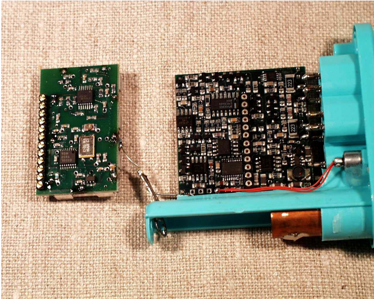
Figure 3: PCB and RF board assembly with RF board removed
