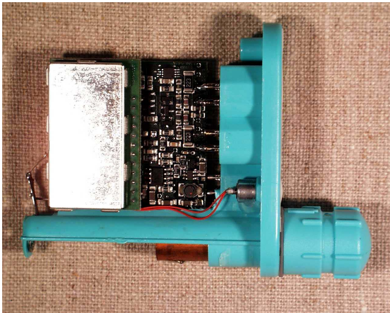
Figure 2: PCB and RF boards assembled, top view
