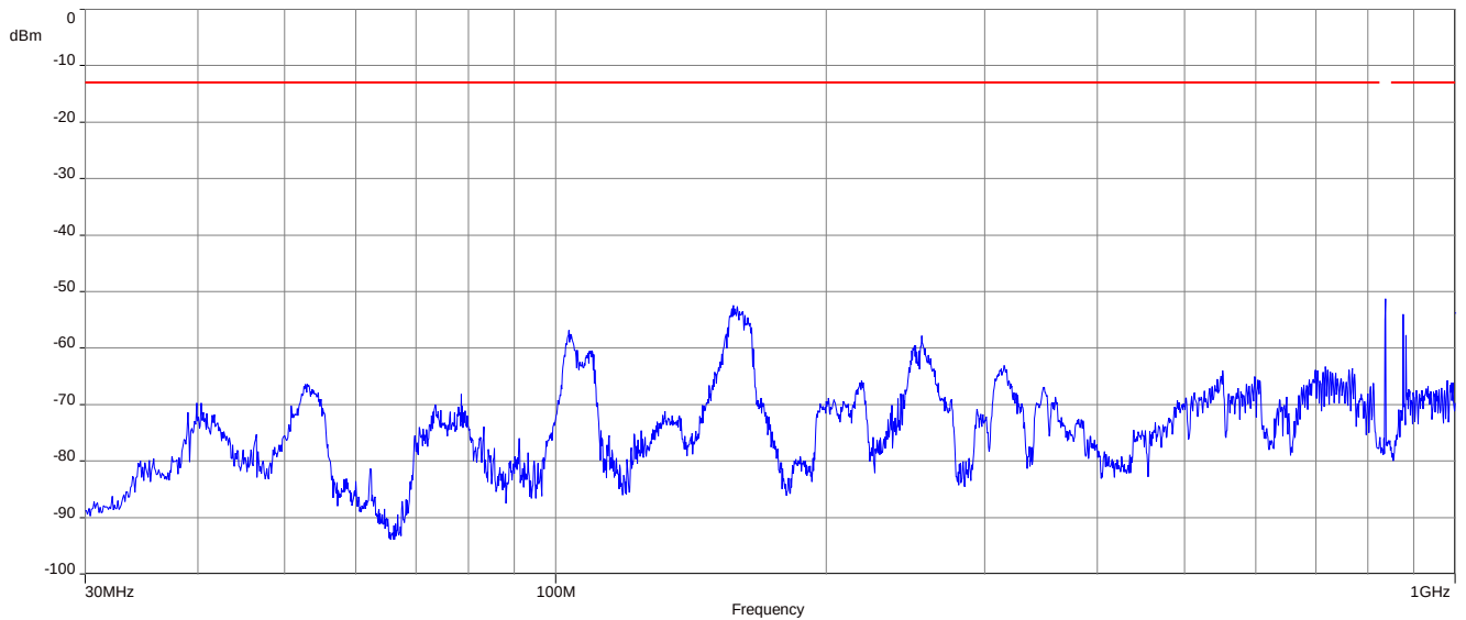
Plot 2: Channel 189 (30 MHz – 1 GHz)
