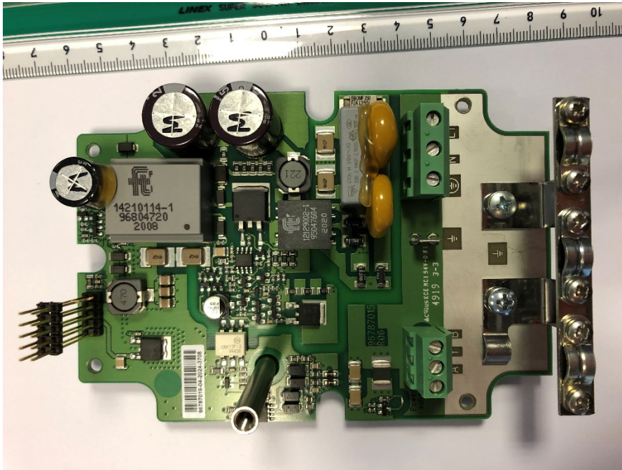
Front / component side
