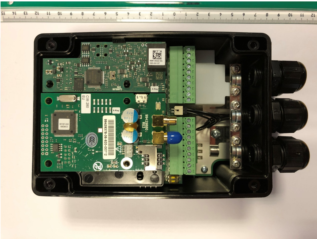
Closeup with optional CIM 280 module inserted
