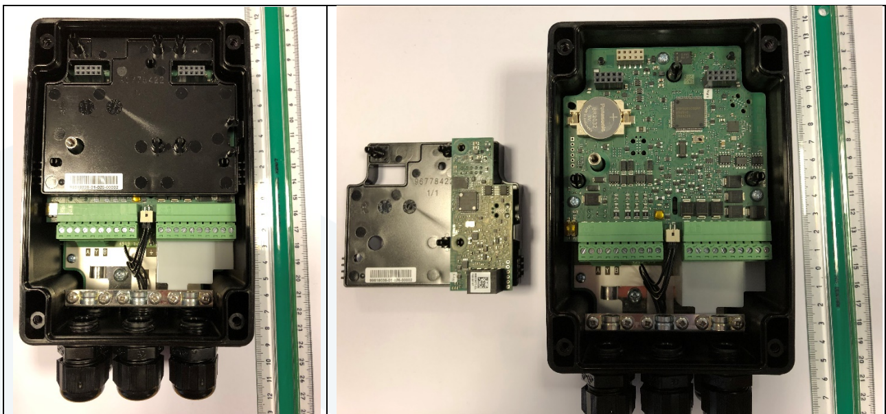
Photos of IO board
