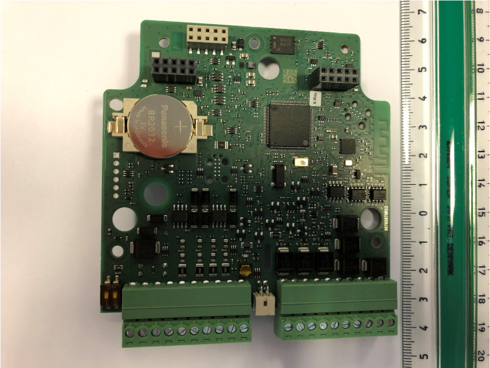
Front / component side
