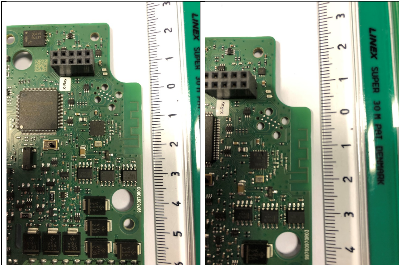
Radio area & antenna closeup
