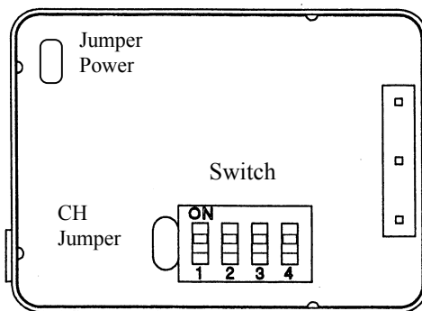
CDP - TX - 02
