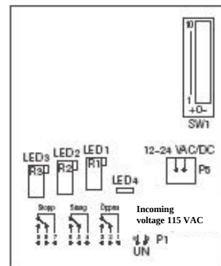
Figur 1. Receiver 3 functions
