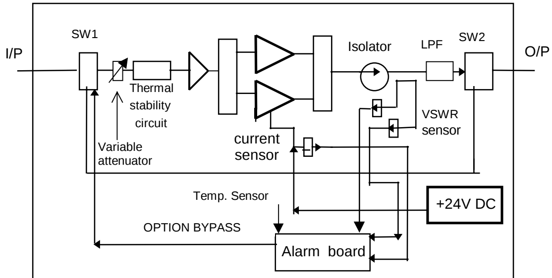
Figure 3 HPA Module
