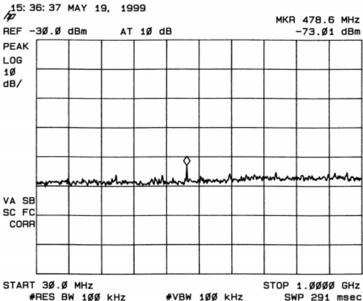
Plot 9.2: Conducted emissions 30 MHz – 1.0 GHz
