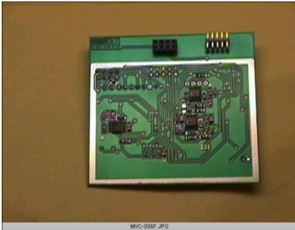
Qual-Tron: PCB Decoder Receiver Foil Side
