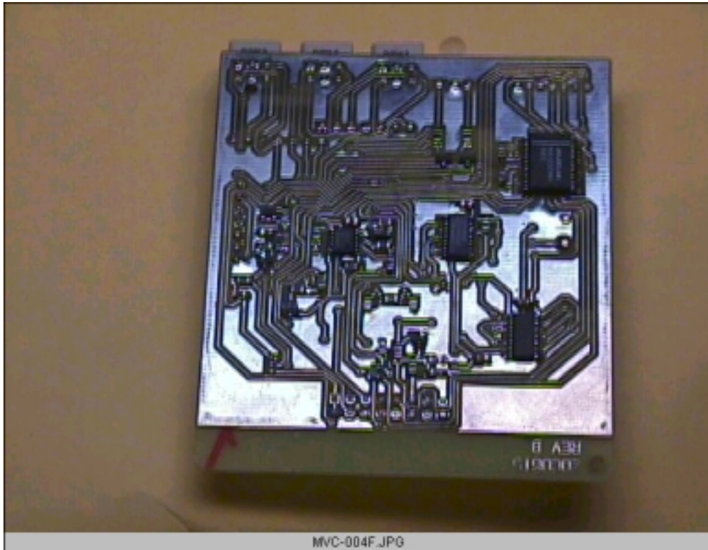
Qual-Tron: PCB Transmitter Encoder Foil Side
