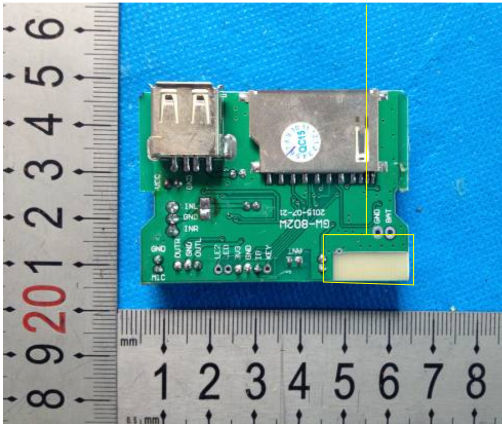
One internal BT Antenna, Fixed on PCB, length: 16mm
