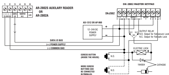
Dual-Station Access Control Door Lock
