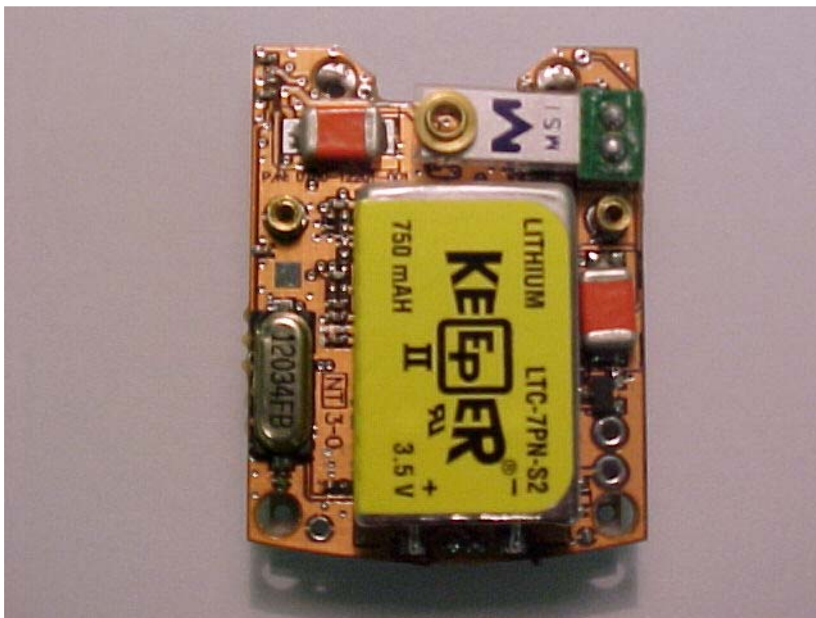
Photo Three – Internal PCB with Battery
