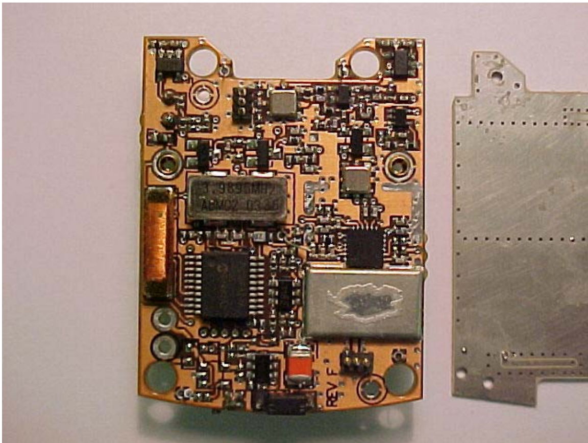
Photo Six – Internal Close-up of Flip side of Component PCB
