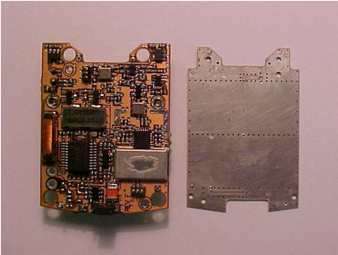
Photo Five – Internal PCB's Separated showing flip side of PCB Antenna
