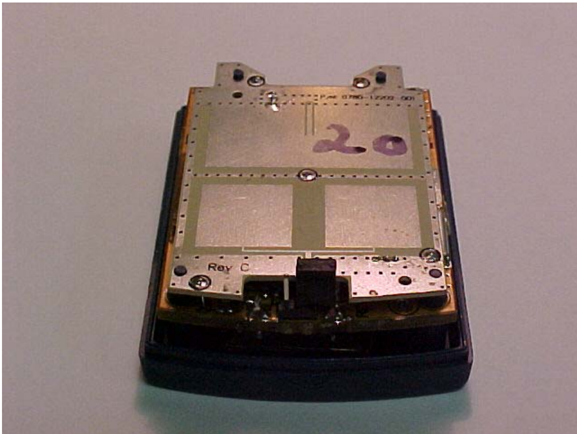
Photo Two – Internal Two PCB's Layered Together
