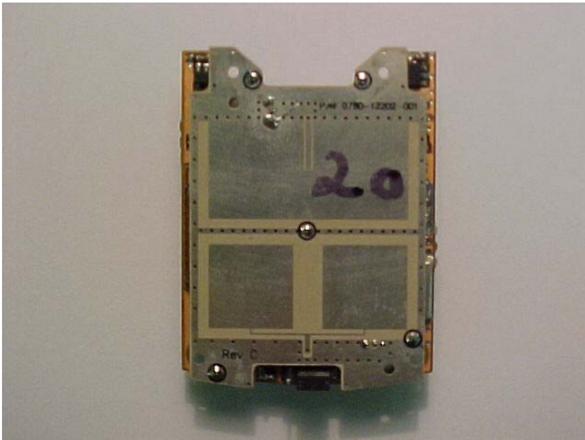
Photo Four – Internal PCB Antenna
