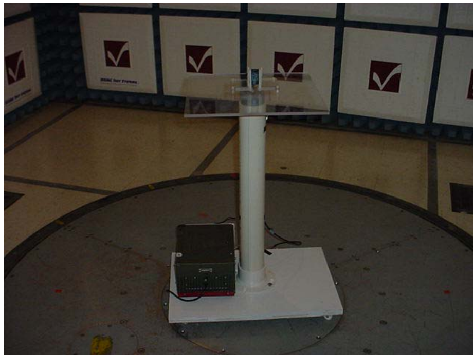
EUT Setup During Radiated Emission Testing
