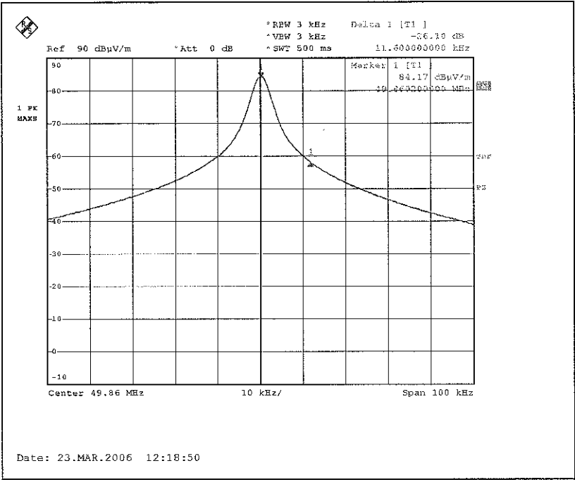
Bandwidth Plot
