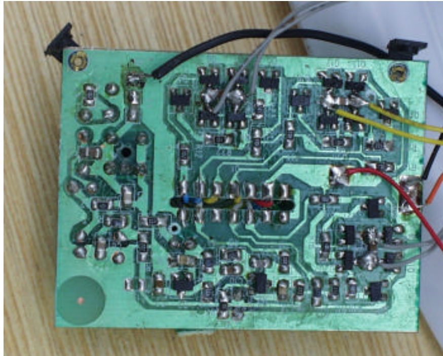
FRONT VIEW OF THE PRINTED WIRING BOARD
