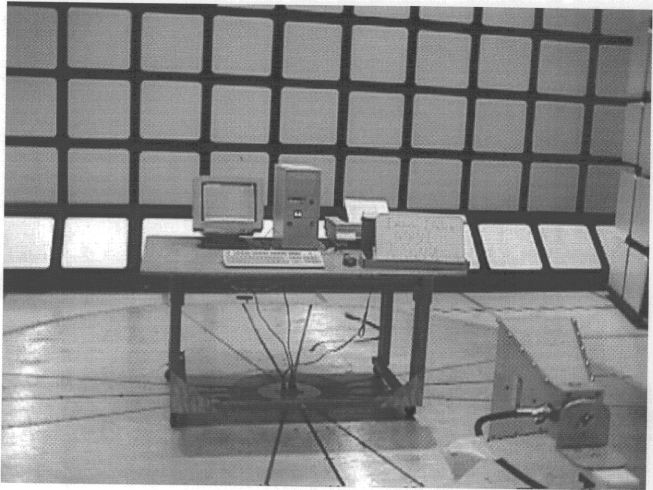
RADIATED EMISSIONS 1GHZ – 10GHZ
