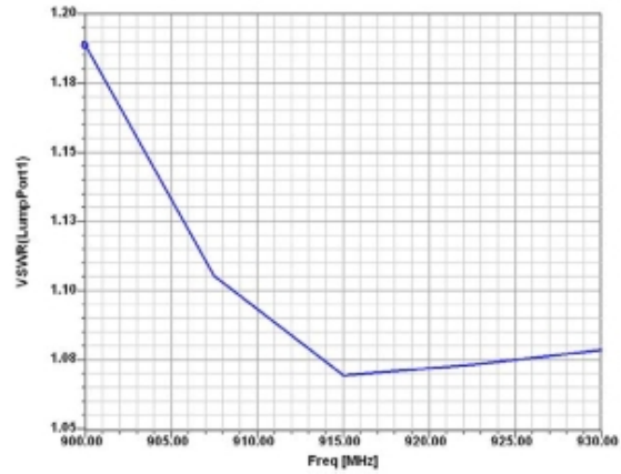
VSWR diagram
