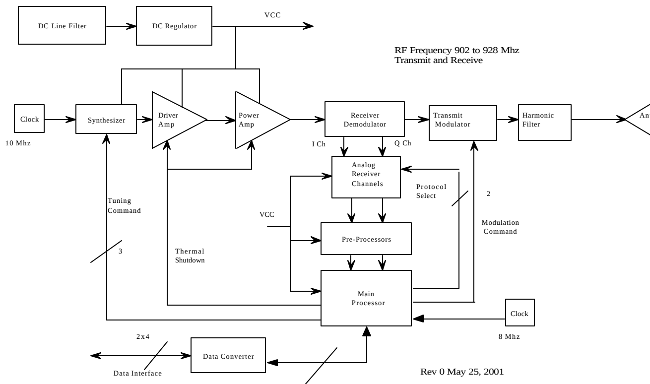
figure 1. Functional Diagram of AWID LR-911
