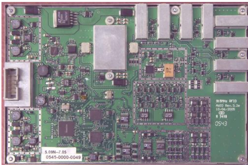
MAIN BOARD – TOP SIDE with SHIELD
