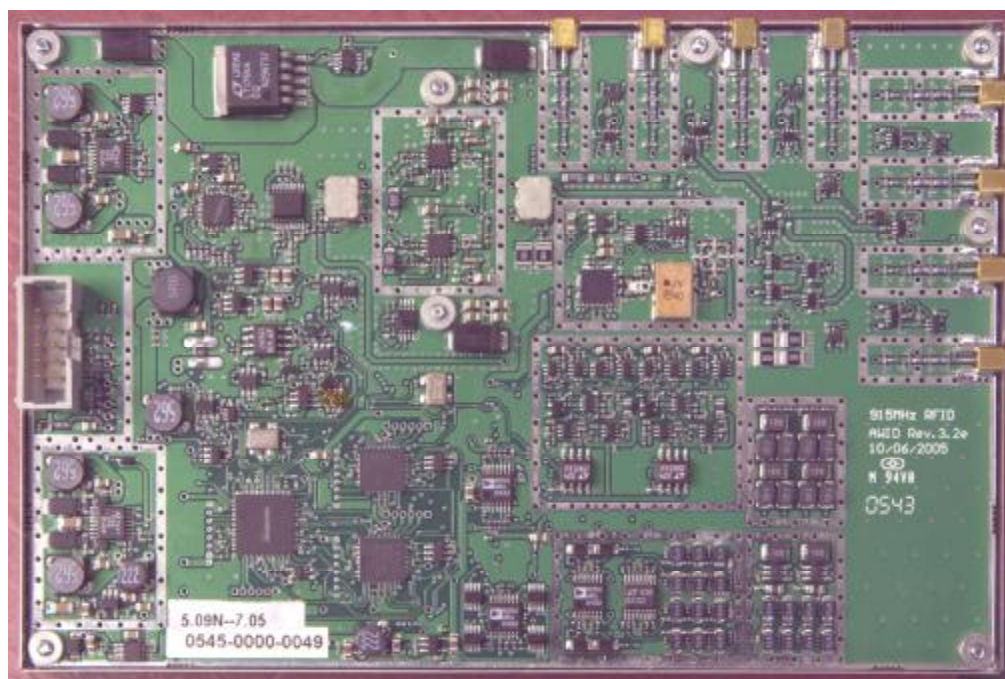
MAIN BOARD – TOP SIDE without SHIELD
