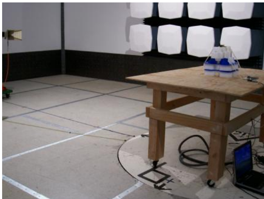
Radiated Emission setup > 1 GHz with 2 dBi Dipole Antenna
