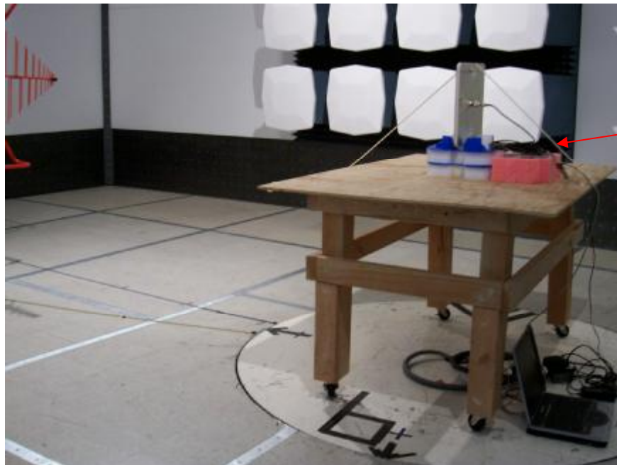
Radiated Emission setup < 1 GHz with 10 dBi Patch Antenna
