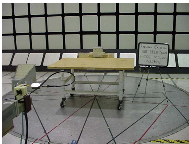
Front – 1-10GHz
