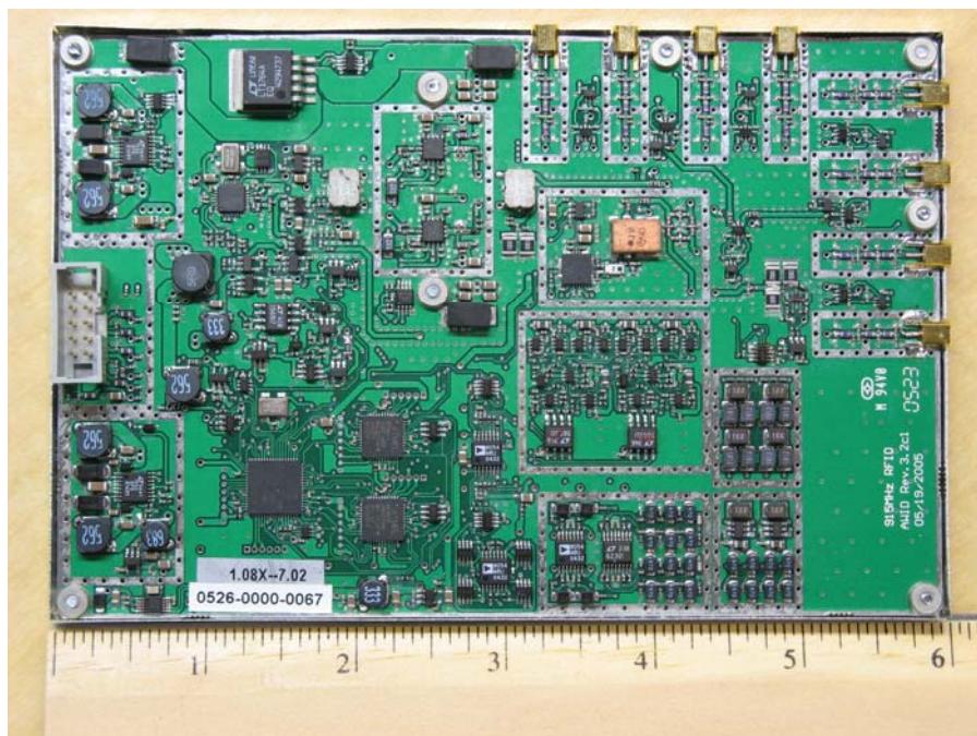
MAIN BOARD – TOP SIDE without SHIELD
