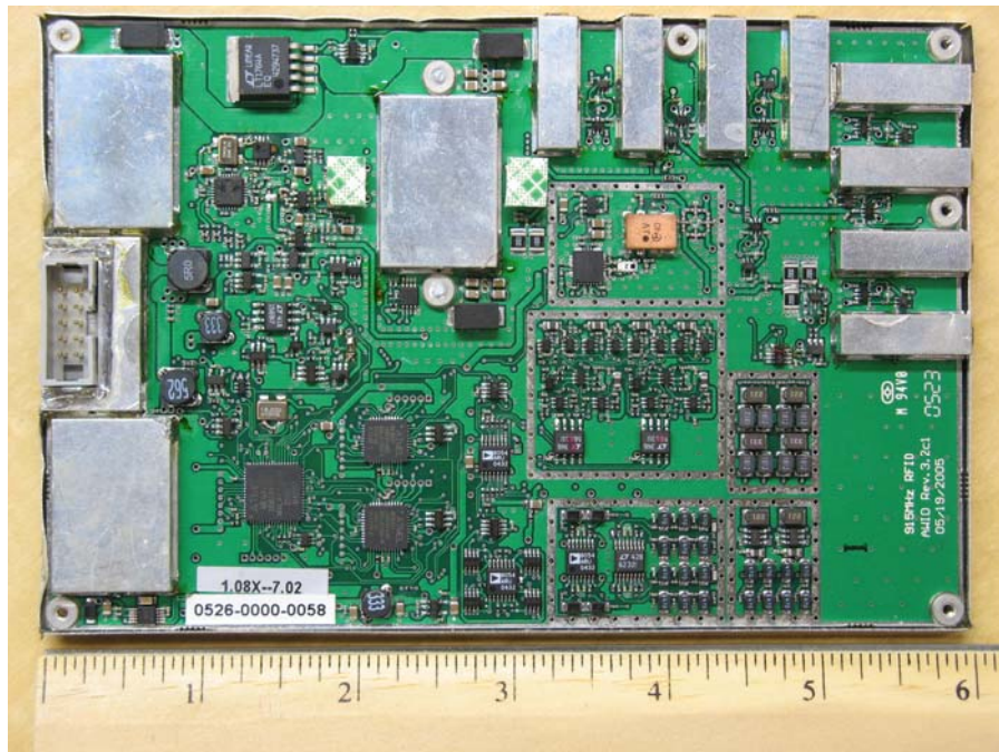
MAIN BOARD – TOP SIDE with SHIELD
